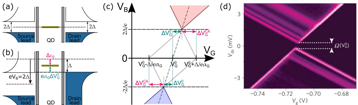
Fig. 1.16: (a) Energy diagram of an SC-QD-SC transistor at a degeneracy point for V_G = V_G^0 and V_B = 0 V. (b) When asymmetrically biasing the junction by V_B = 2\Delta/e , the bias coupling induces a level-depth shift of \Delta\epsilon_0 . A certain gate detuning of \Delta V_G^0 , aligning the level with the coherence peaks (black dashed line) is required to reach the conduction point. (c) Illustrative stability diagram SC-QD-SC transistor, indicating the zero- V_B position of the degeneracy point and the V_G -shifts of the diamond apexes caused both by the bias lever arm ( \Delta V_G^{CA} ) and the asymmetric biasing configuration ( \Delta V_G^0 ). The dashed-dotted black line indicates the position of \epsilon_0 = 0 at finite V_B . (d) dI/dV_B map of an aluminum QD transistor contacting a C_{60} molecule, made by electromigration, highlighting the spectroscopic gap and diamond apexes misalignment at charge degeneracy (extracted from [39]).
