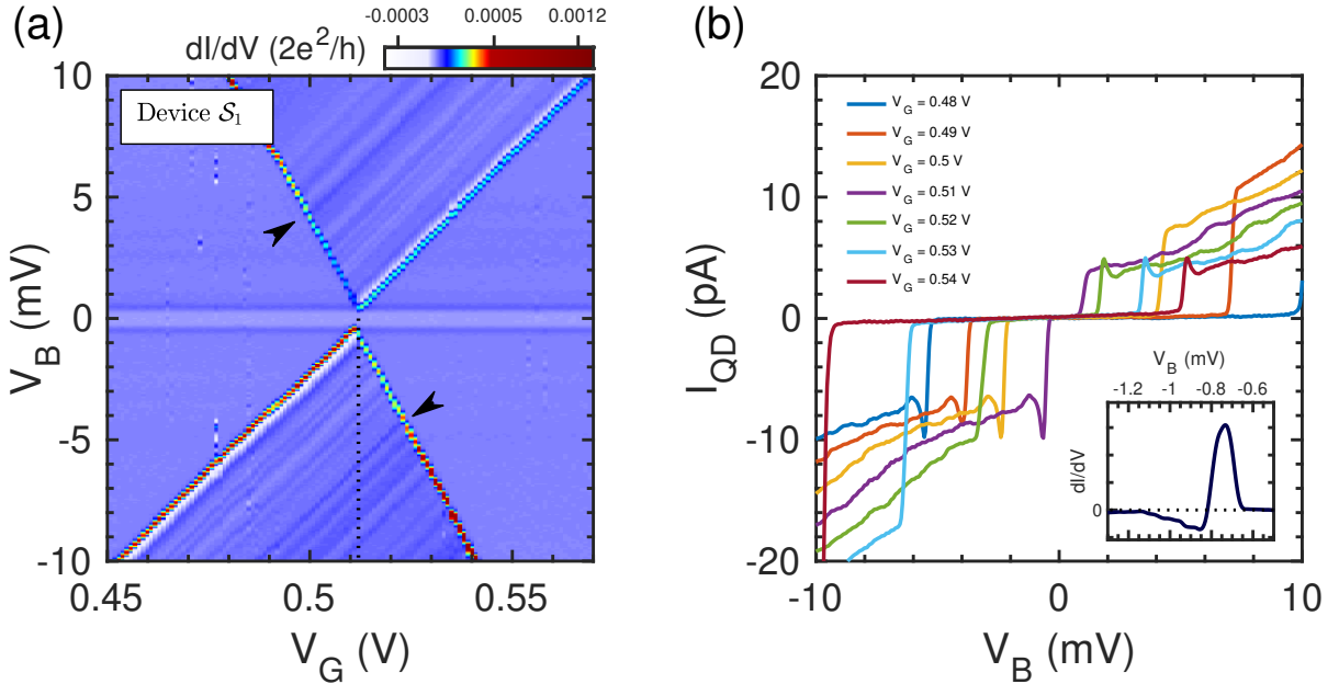
Fig. 4.1: (a) dI/dV_B transport map measured at 80 mK, showing the single degeneracy point at V_G^0 \approx 0.512 V (black dashed arrow) of device \mathcal{S}_1 that could be accessed. The slightly stronger resonance inside the on-state diamonds (black arrows) is identified with the addition of a subsequent QD energy level inside the V_B -window. (b) I - V_B curves showing the current flowing solely through the QD at different V_G values. Inset: dI/dV_B versus V_B for V_G = 0.51 V, zooming at the DE^+ peak (with a \text{FWHM} \approx 88 \mu\text{eV} ).
