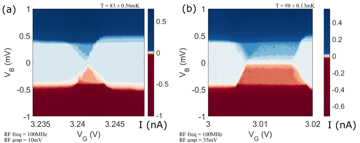
Fig. A.6: (a,b) Current maps of device S_5 acquired while applying a sinusoidal RF signal at the gate electrode of f = 100 MHz and respective amplitudes of 10 and 35 mV at the input of the cryostat.
