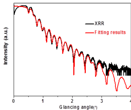
Figure 5-14. Measured (black line) and fitted (red line) XRR curves of the PFP-1 stack accounting for the presence of Pt_{69}Fe_{31} interlayers at both interfaces.
