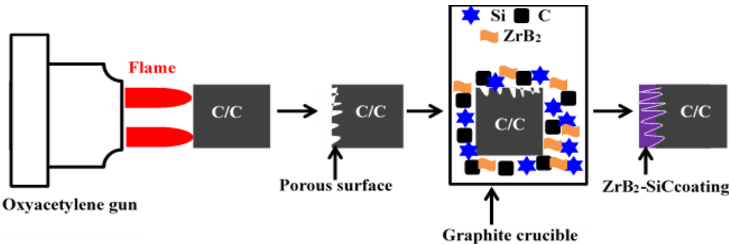
Figure 2-7. Schematic diagram of C/C blasting treatment and introducing ZrB 2 into SiC coating by pressure-less reactive sintering.
