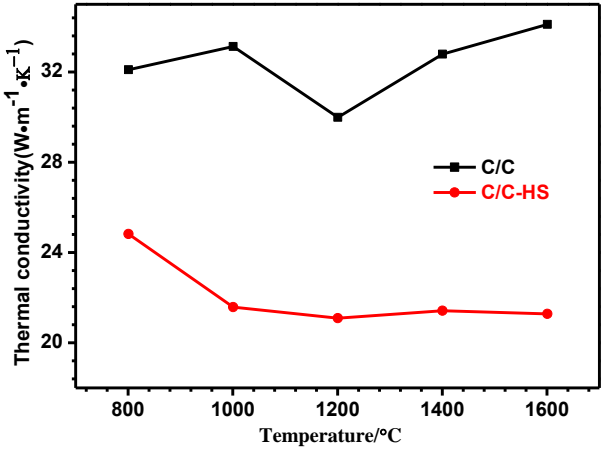
Figure 6-11. Thermal conductivity of the C/C and C/C-HS at high temperature.
