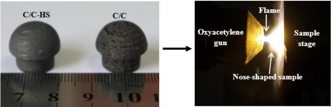
Figure 6-12. Macroscopic image (left) of the fabricated C/C and the C/C-HS and experimental setup (right) of the ablation test using oxyacetylene torch.
