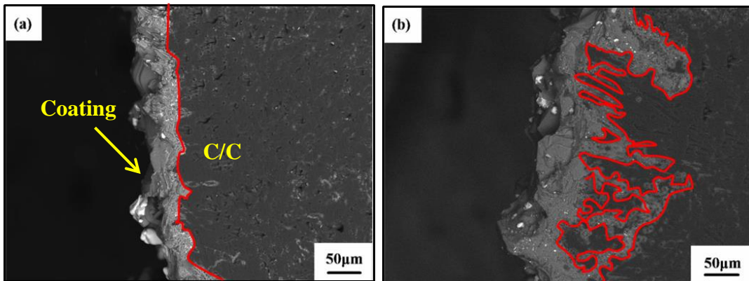
Figure 4-9. Cross-section morphologies of the coating, (a) Z-S-1, (b) Z-S-2.
