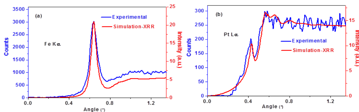
Figure 5-15. Comparison of the experimental and revised simulated Fe Kα (a) and Pt Lα (b) Kossel curves of the PFP-1 stack.
