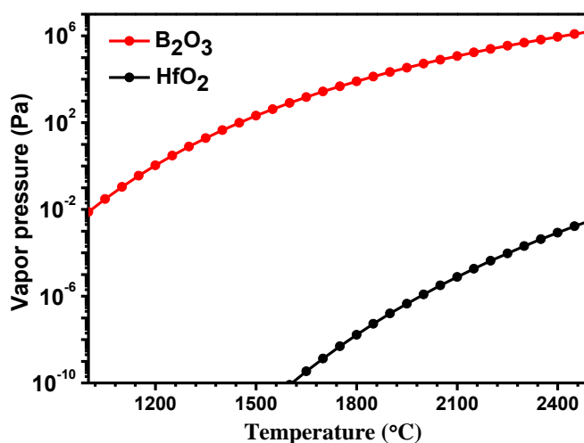
Figure 6-9. Vapor pressure vs temperature for B_2O_3 and HfO_2 calculated at ambient pressure (Vapor pressure in logarithmic scale).
