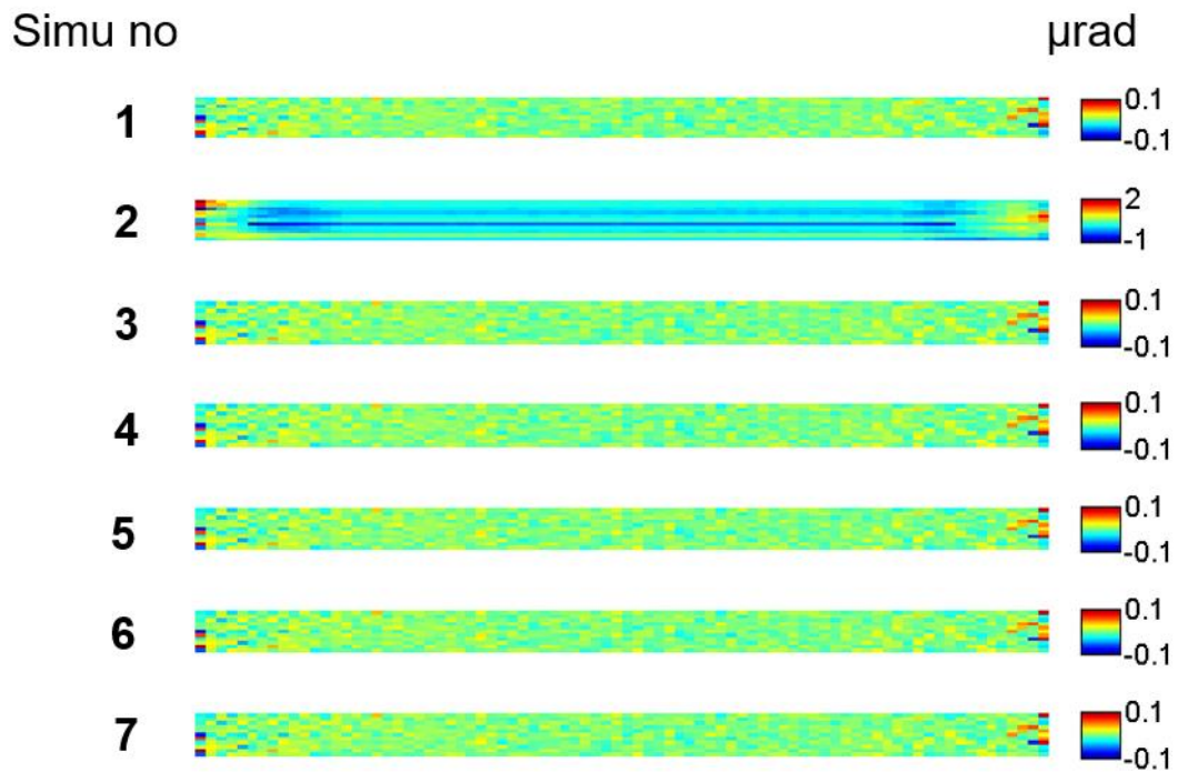
Figure 3.14 : Simulated tangential slope errors of size 100 x 13.2 mm 2 , stitched with different PyLOSt algorithms.
