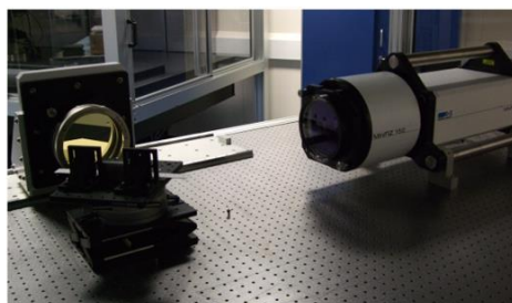
Photograph of the Minifz interferometer in double-pass configuration
