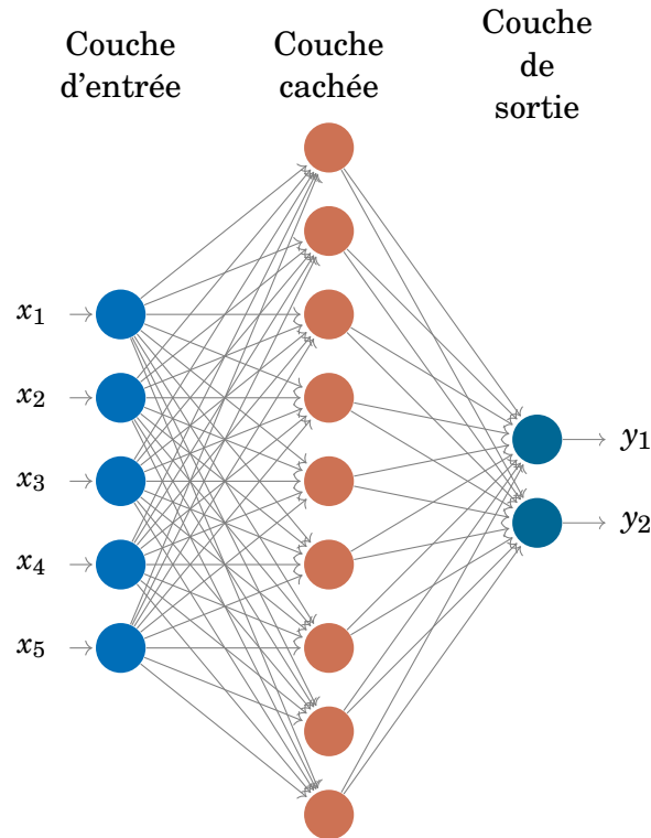
FIGURE II.3 – Le perceptron
