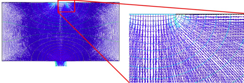
FIGURE 2.10: Zoom-in plot of the current streamlines at the ends of the electrode for L_e = 0.2 .
