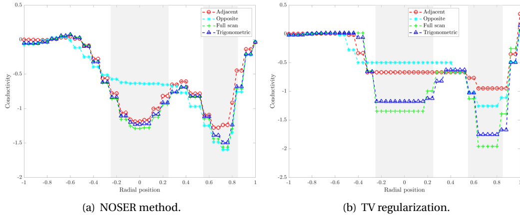
FIGURE 5.24: [Case 4] Profiles of the reconstructed conductivity contrasts \Delta\sigma_{\text{id}}^h along one diameter for the different excitation strategies and reconstruction methods considered.
