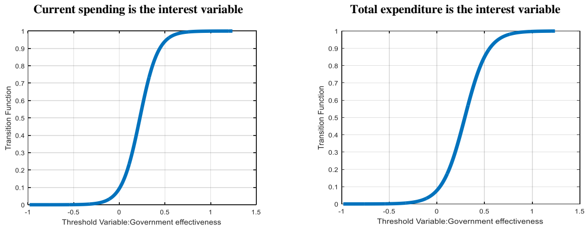
Figure 6: Transition functions
