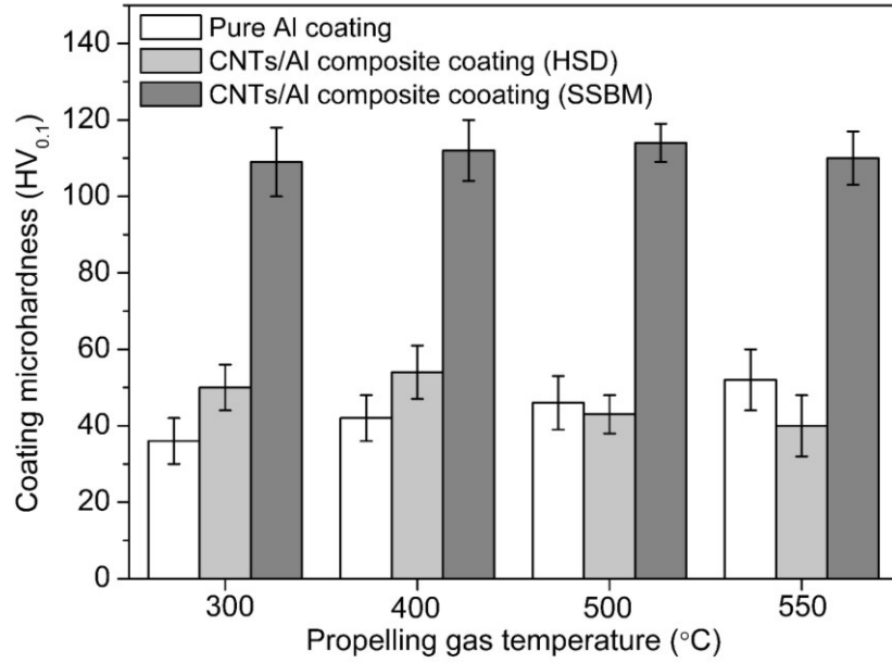
Figure 3-17 Microhardness of the as-sprayed coatings.
