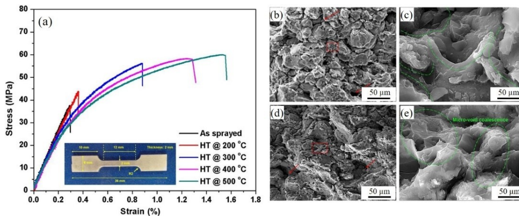
Figure 1-31 Tensile stress-strain plots of as-sprayed and heat-treated B_4C/Al composite samples. Fracture morphologies of (b and c) as-sprayed and heat-treated (500 °C) B_4C/Al composite samples [101].
