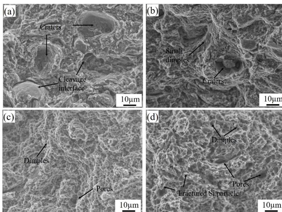
Figure 4-23 Fracture morphologies of the as-sprayed and annealed TiB_2/AlSi10Mg-CT2 composite samples at different temperatures after the tensile test: (a) as-sprayed state; (b) 300 °C; (c) 400 °C; (d) 500 °C.
