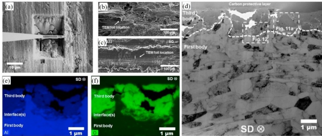
Figure 1-28 TEM investigation of the wear mechanisms of CSed Al_2O_3/Al composite coating: (a) technique of TEM foil; (b) and (c) wear track surfaces showing TEM foil locations; (d) TEM micrograph of the cross-section region near the wear track surface; (e) and (f) EDS mapping of Al K\alpha and O K\alpha intensities in the third body, the surrounding first body, and interfaces [102].
