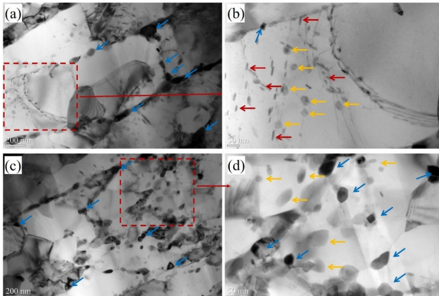
Figure 5-25 TEM micrographs of the TiB_2/7075Al-C1 deposit showing the precipitate structure. (b) and (d) the magnified micrographs within red dashed boxes of (a) and (c), respectively. Red arrows show needle-like precipitates dispersed in the Al matrix, while the yellow arrows indicate the spherical precipitates. The blue arrows indicate the in-situ formed TiB_2 nanoparticles in the Al matrix.
