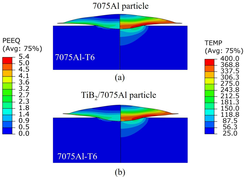
Figure 5-12 Distribution of PEEQ (on the left-hand side) and temperature (on the right-hand side) of the single (a) 7075Al and (b) TiB 2 /7075Al composite particles deposited onto 7075Al-T6 substrate in C3.
