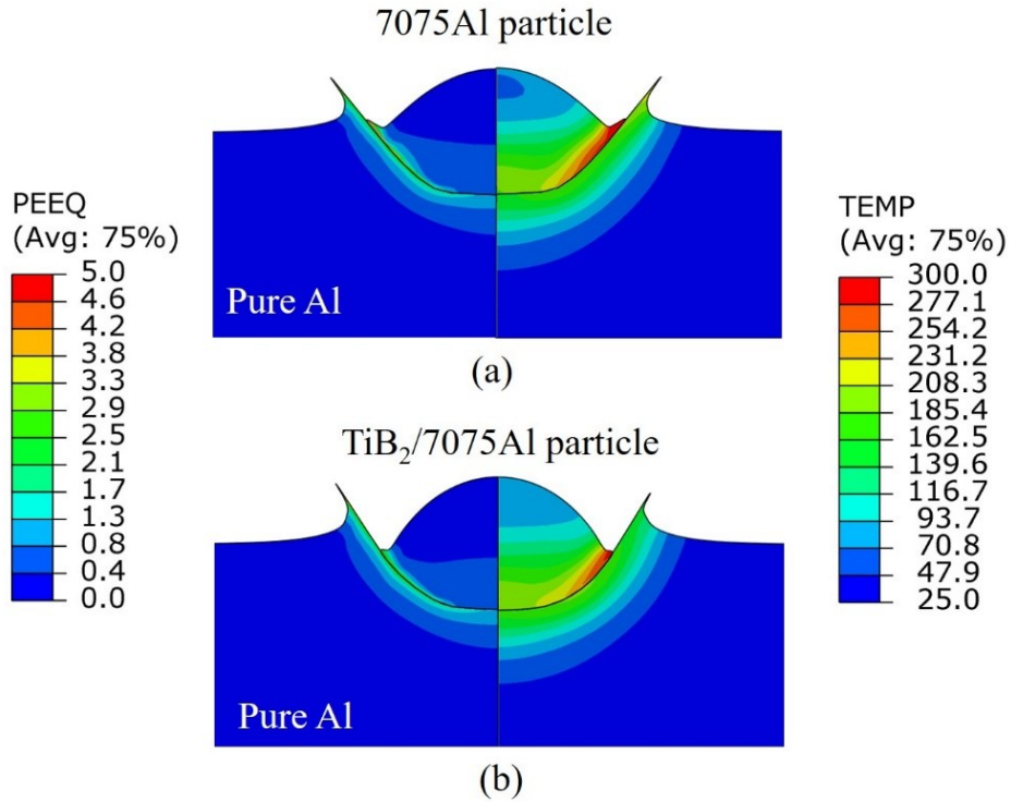
Figure 5-9 Distribution of PEEQ (on the left-hand side) and temperature (on the right-hand side) of the single (a) 7075Al and (b) TiB_2/7075Al composite particles deposited onto pure Al substrate in C3.
