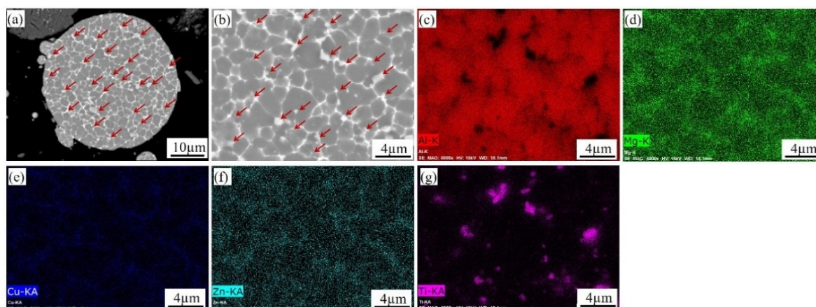
Figure 2-10 BSE/SEM micrographs of the cross-section of (a) a whole \text{TiB}_2/7075\text{Al} composite particle in the as-received condition and (b) magnified view highlighting the distribution of \text{TiB}_2 particles; corresponding EDS element distributions of (c) Al, (d) Mg, (e) Cu, (f) Zn and (g) Ti.
