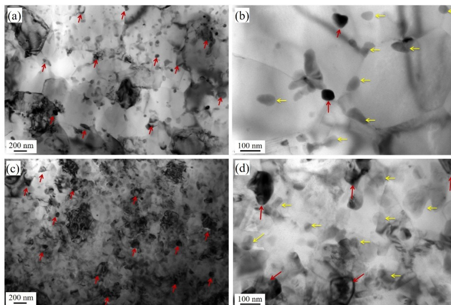
Figure 4-37 TEM bright-field (BF) images of CSed and FSPed TiB_2/AlSi10Mg-CT2 composite samples; (b) and (d) are the magnified views.
