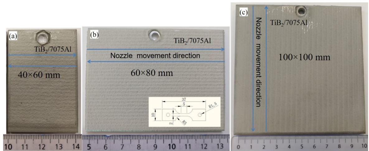
Figure 2-16 Photos of the CSed TiB_2/7075Al composite coatings onto Al substrates using different processing parameters: (a) C1; (b) C2; (c) C3.
