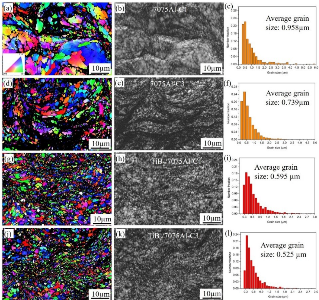
Figure 5-23 SEM/EBSD characterization of the cross-section of the CSed (a-f) pure 7075Al and TiB_2/7075Al composite deposits in different processing conditions: (a-c) 7075Al-C1; (d-f) 7075Al-C3; (g-i) TiB_2/7075Al-C1 ; (j-l) TiB_2/7075Al-C3 . The first column displays grain orientation maps, and the middle column presents the band contrast. The last column shows grain size distribution of the Al matrix (the TiB_2 phase was eliminated).
