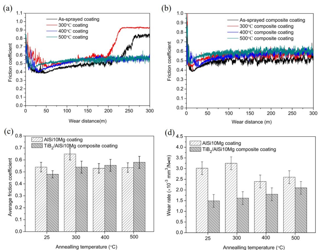
Figure 4-17 Friction coefficient vs. sliding wear distance for (a) AlSi10Mg -CT1 and (b) TiB_2/AlSi10Mg -CT1 composite coatings. (c) and (d) display the average friction coefficient and wear rate as a function of annealing temperatures, respectively.
