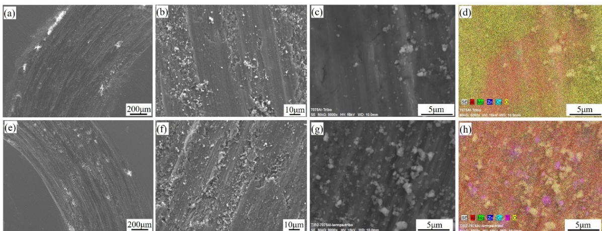
Figure 5-31 Overviews, magnified views and EDS mapping of the worn morphologies of C1 7075Al-C1 and TiB 2 /7075Al-C1 composite coatings.
