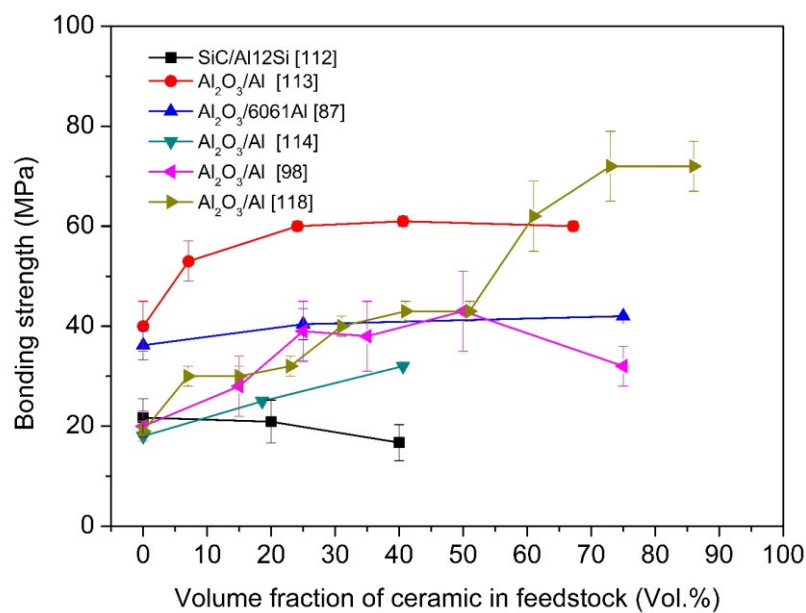
Figure 1-26 Bonding strength as a function of volume fraction of ceramics in the source powder mixture.
