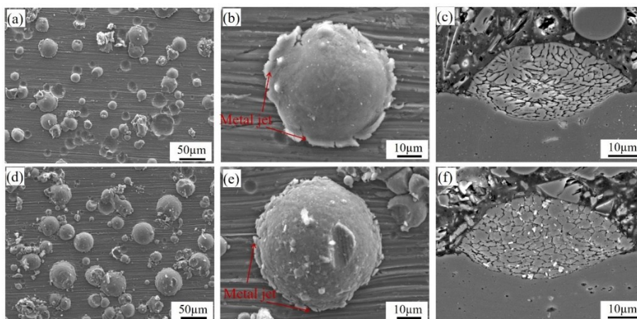
Figure 5-13 Surface and cross-sectional morphologies of single 7075Al and TiB_2/7075Al composite splats deposited onto Al substrate at C1: (a-c) 7075Al; (d-f) TiB_2/7075Al composite.
