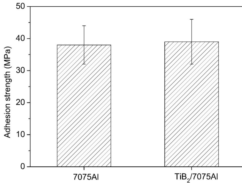
Figure 5-29 Adhesion strength evolution of 7075Al and TiB_2/7075Al composite in C1.
