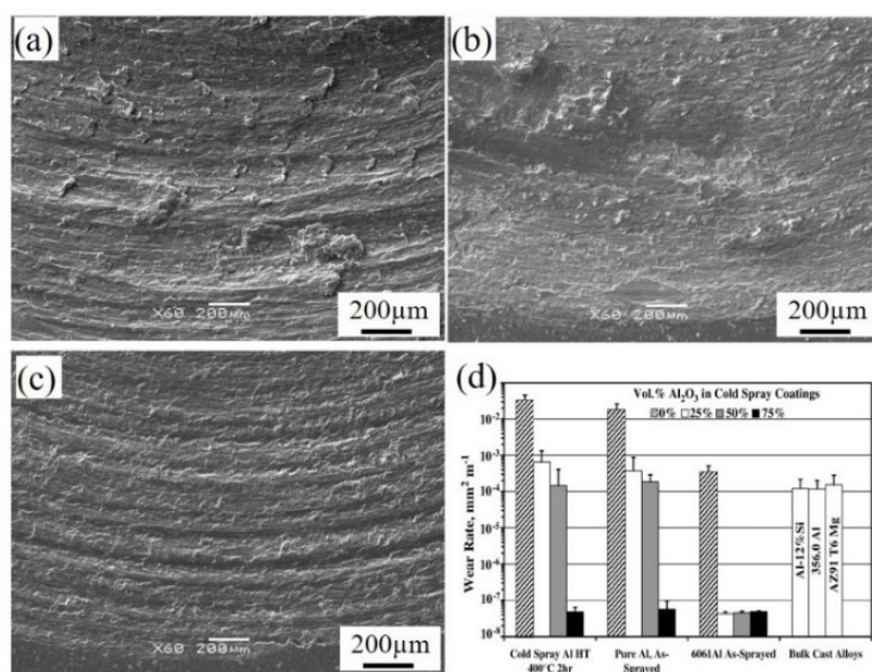
Figure 1-27 Wear tracks on CSed Al coating (b) CSed Al-50% Al_2O_3 coating and (c) CSed Al-75% Al_2O_3 coating. (d) wear rates of coatings compared to bulk alloys [130].
