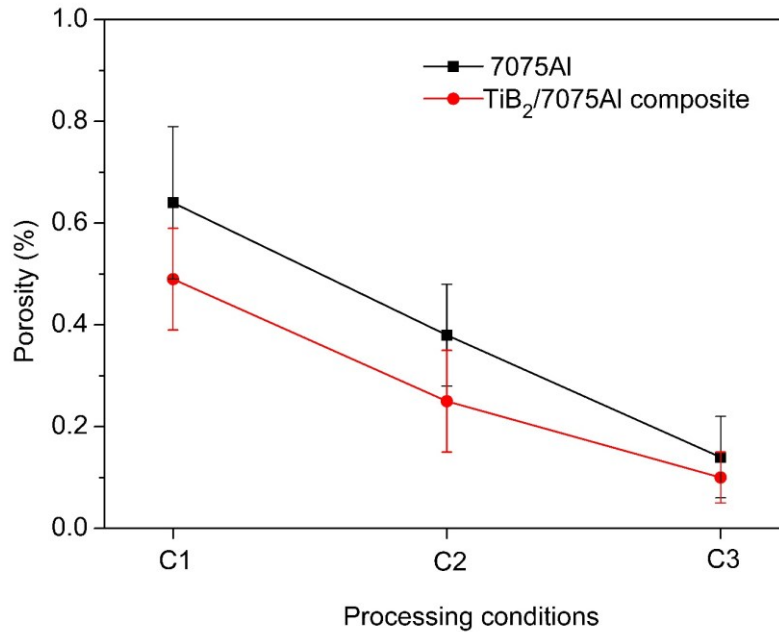
Figure 5-20 Porosity evolution of the 7075Al and TiB_2/7075Al composite deposits in different processing conditions.
