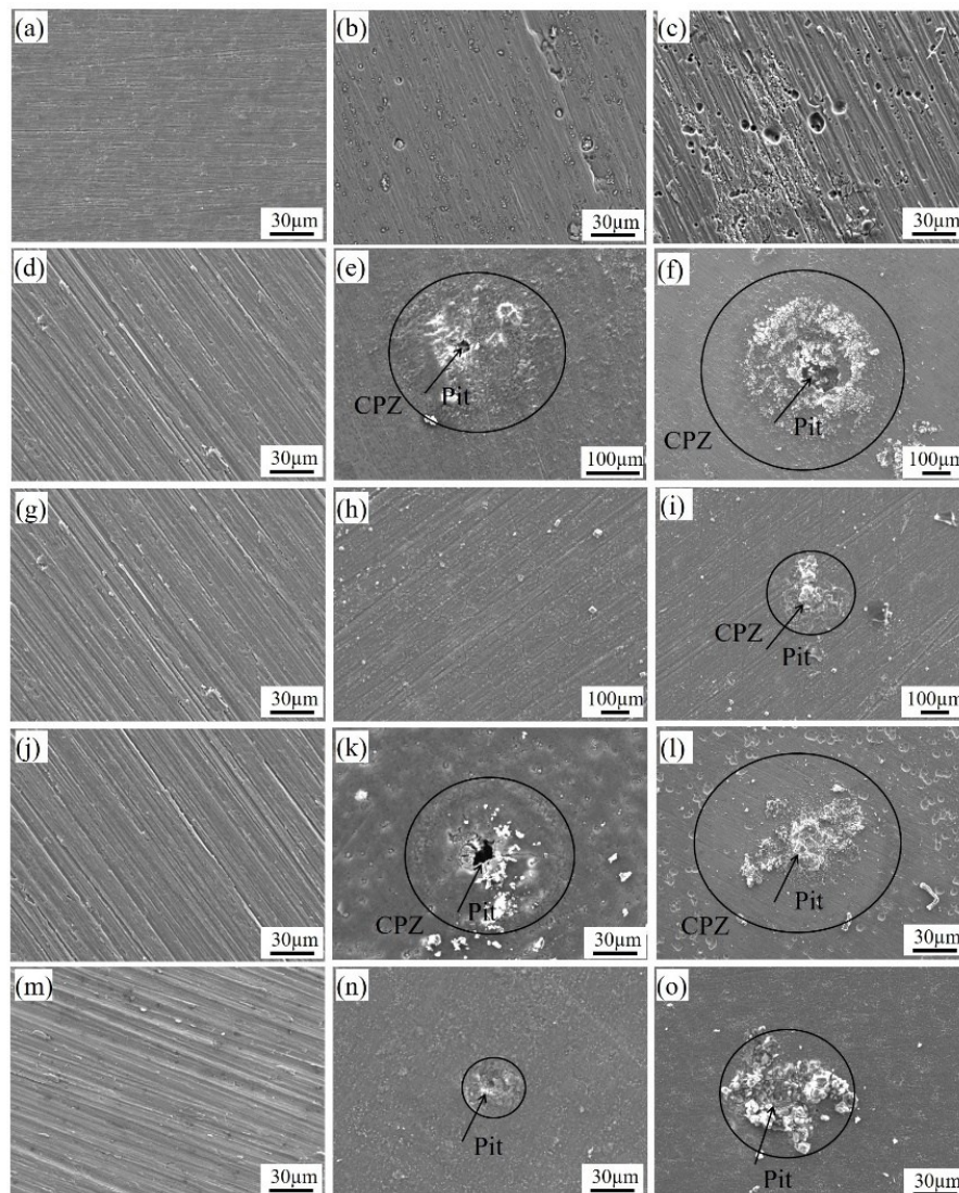
Figure 5-34 SEM images of the 7075Al bulk, 7075 Al and TiB_2/7075Al composite coatings before (first row) and after open circuit immersion in 0.1 M (middle row) and 0.6 M (third row) NaCl for 7 days: (a-c) 7075Al bulk; (d-f) 7075Al-C1; (g-i) TiB_2/7075Al -C1; (j-l) 7075Al-C3; (m-o) TiB_2/7075Al -C3.
