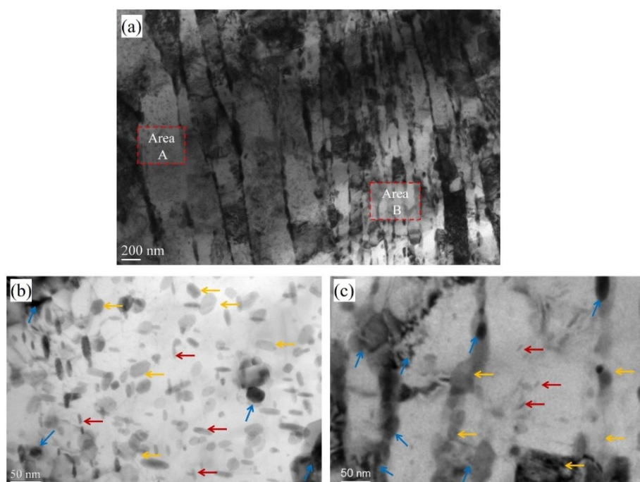
Figure 5-27 TEM micrographs of the TiB_2/7075Al-C3 deposit showing a pancake structure. (b) and (c) are the corresponding magnified micrographs of area A and B in (a), respectively.
