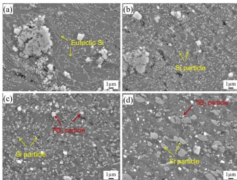
Figure 4-35 Magnified SEM images of the cross-section of the FSPed TiB_2/AlSi10Mg deposits in different regions corresponding to the A, B, C and D as marked in Figure 4-28a.
