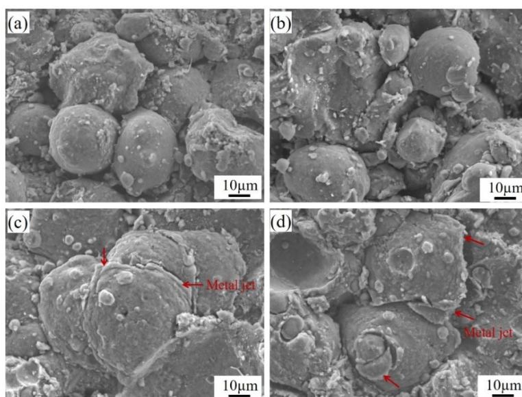
Figure 4-1 Surface morphologies of the as-sprayed AlSi10Mg and TiB_2/AlSi10Mg deposits obtained from different conditions: (a) AlSi10Mg-CT1 ; (b) TiB_2/AlSi10Mg-CT1 ; (c) AlSi10Mg-CT2 ; (d) TiB_2/AlSi10Mg-CT2 .
