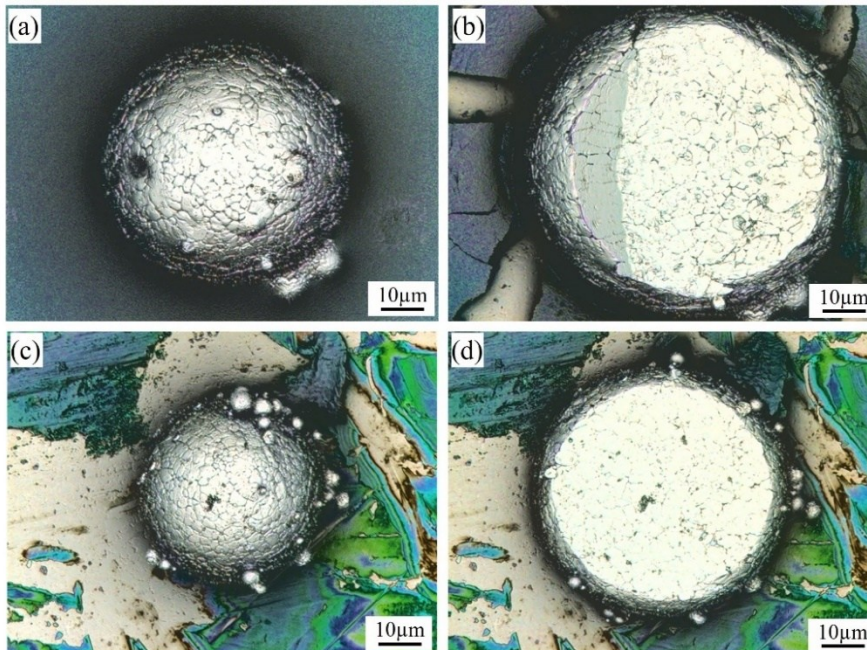
Figure 2-21 The particle morphologies before and after compression tests: (a, b) a 7075Al particle with a size of 51 \mu\text{m} before and after compression tests; (c, d) a \text{TiB}_2/7075\text{Al} composite particle with a size of 44 \mu\text{m} before and after compression tests.
