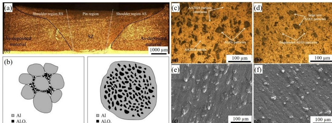
Figure 1-33 Microstructure modification for CSed AMCs coatings: (a) macroscopic cross-section of the FSPed \text{Al}_2\text{O}_3/2024\text{Al} [146]; (b) Schematic of reinforcing particle re-distribution in MMC coatings during FSP. [147]; Optical micrographs (c, d) and SEM (e, f) micrographs of CSed (c, e) and FSPed (d, f) \text{Al}_2\text{O}_3/2024\text{Al} [146].
