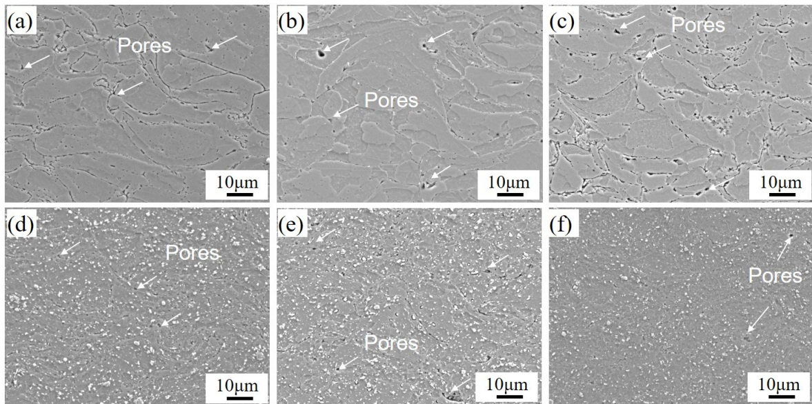
Figure 5-39 Cross-sectional SEM images of the pure 7075Al and TiB_2/7075Al composite deposits after T6 treatment: (a) 7075Al-C1, (b) 7075Al-C2, (c) 7075Al-C3, (d) TiB_2/7075Al -C1, (e) TiB_2/7075Al -C2, (f) TiB_2/7075Al -C3. The pores were indicated by white arrows.
