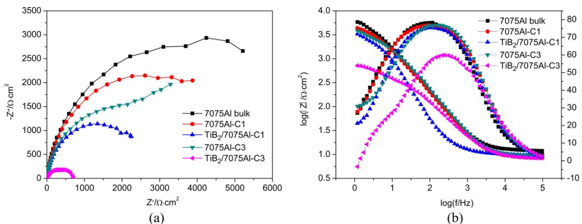
Figure 5-36 Experimental and simulated (a) Nyquist and (b) Bode plots of the bulk 7075Al, and CSed 7075Al and TiB_2/7075Al composite coatings.
