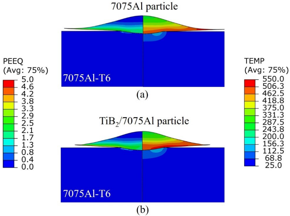
Figure 5-11 Distribution of PEEQ (on the left-hand side) and temperature (on the right-hand side) of the single (a) 7075Al and (b) TiB 2 /7075Al composite particles deposited onto 7075Al-T6 substrate in C2.
