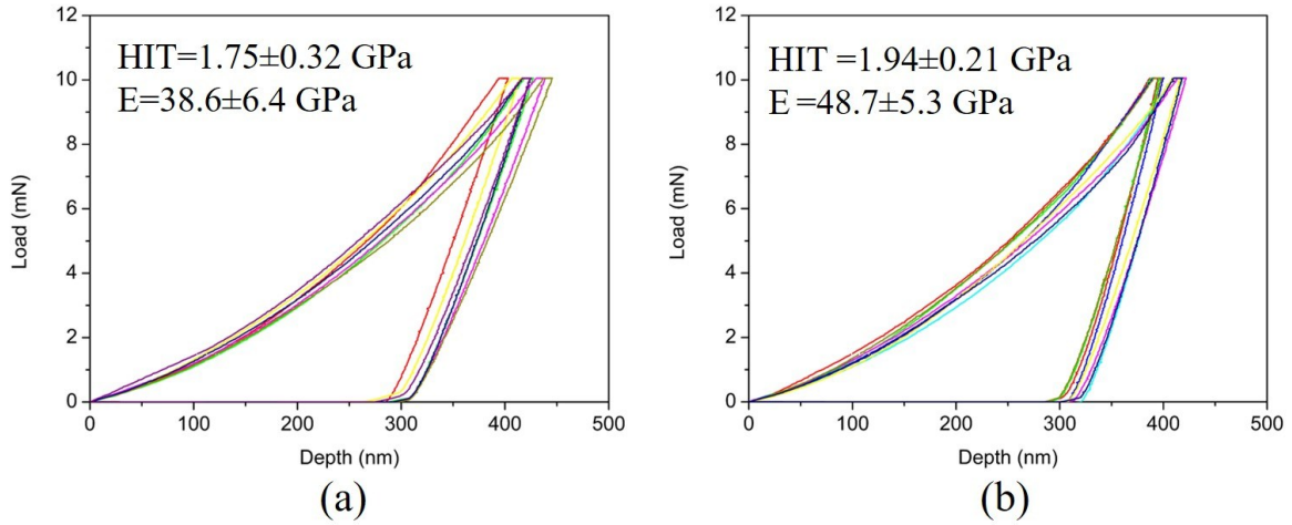
Figure 5-6 Nanoindentation performance of the (a) pure 7075Al particle and (b) TiB_2/7075Al composite particle.
