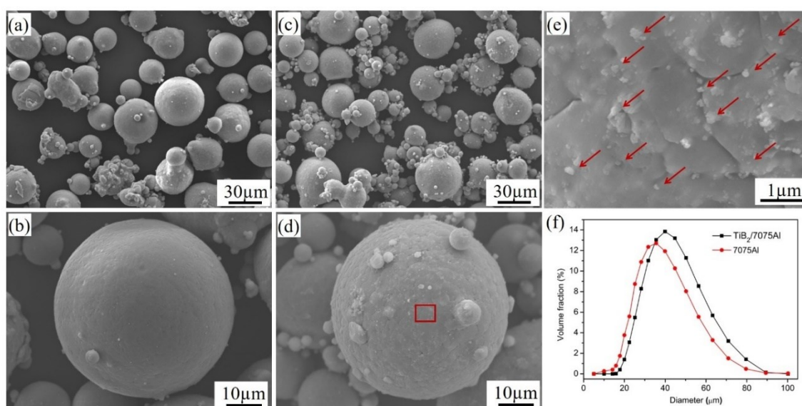
Figure 2-9 Particle morphologies of the (a, b) pure 7075Al powder and (c, d) \text{TiB}_2/7075\text{Al} composite powder in different magnifications; (e) Magnified view of the composite particle surface area marked in (d), showing uniform distribution of \text{TiB}_2 nanoparticles (indicated by red arrows) on the surface of an Al micro-particle; (f) displays the particle size distribution of the initial powder feedstocks.
