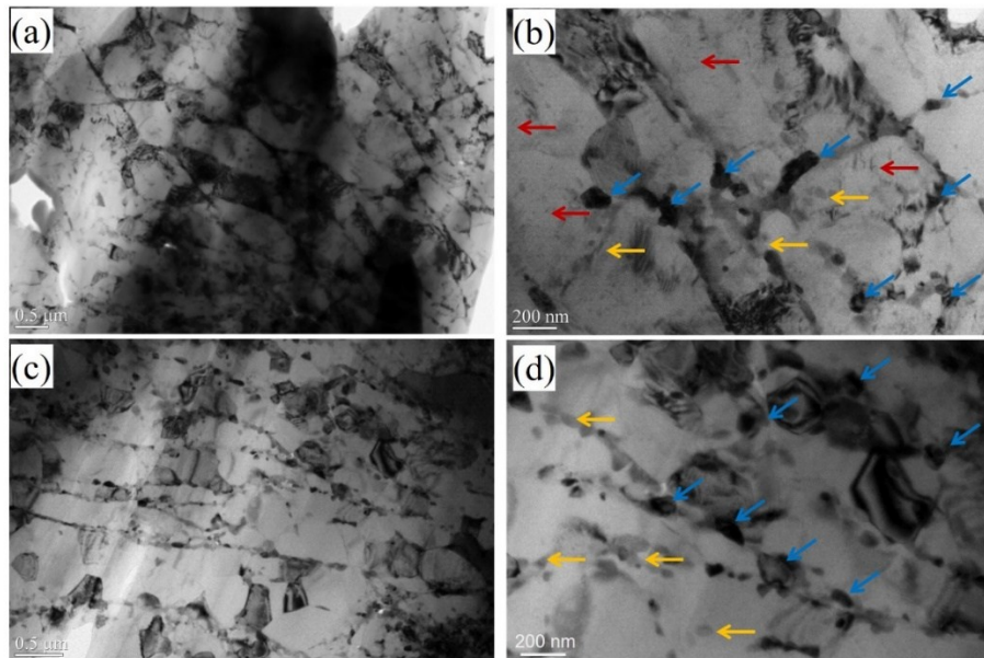
Figure 5-24 TEM micrographs of the TiB_2/7075Al-C1 deposit in different regions: (a) and (b) particle interior; (c) and (d) near interparticle boundaries. Red arrows show needle-like precipitates dispersed in the Al matrix, while the yellow arrows indicate the spherical precipitates. The blue arrows indicate the in-situ formed TiB_2 nanoparticles in the Al matrix.
