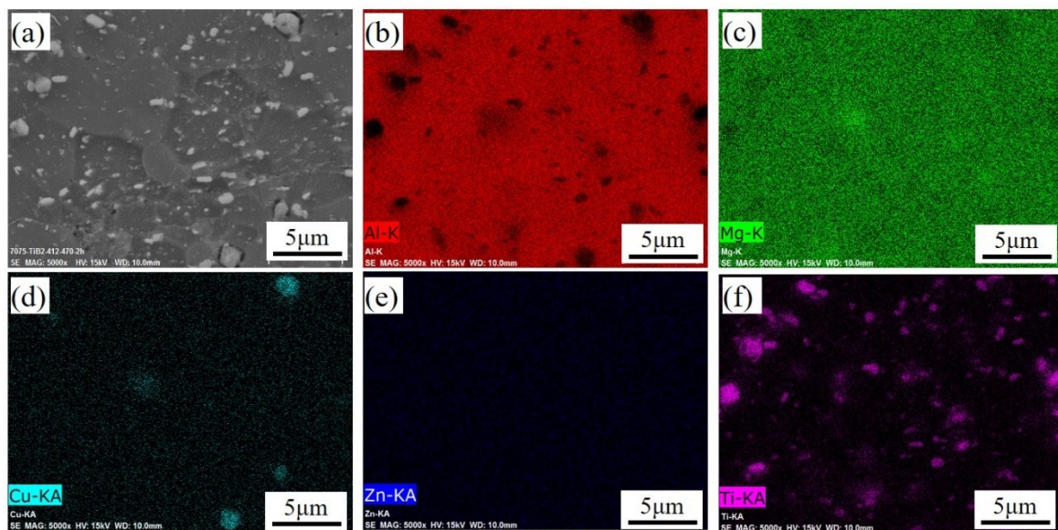
Figure 5-46 EDS mapping of the cross-section of the TiB_2/7075Al-C2 composite deposit after 412 °C/4 h + T6 treatment.
