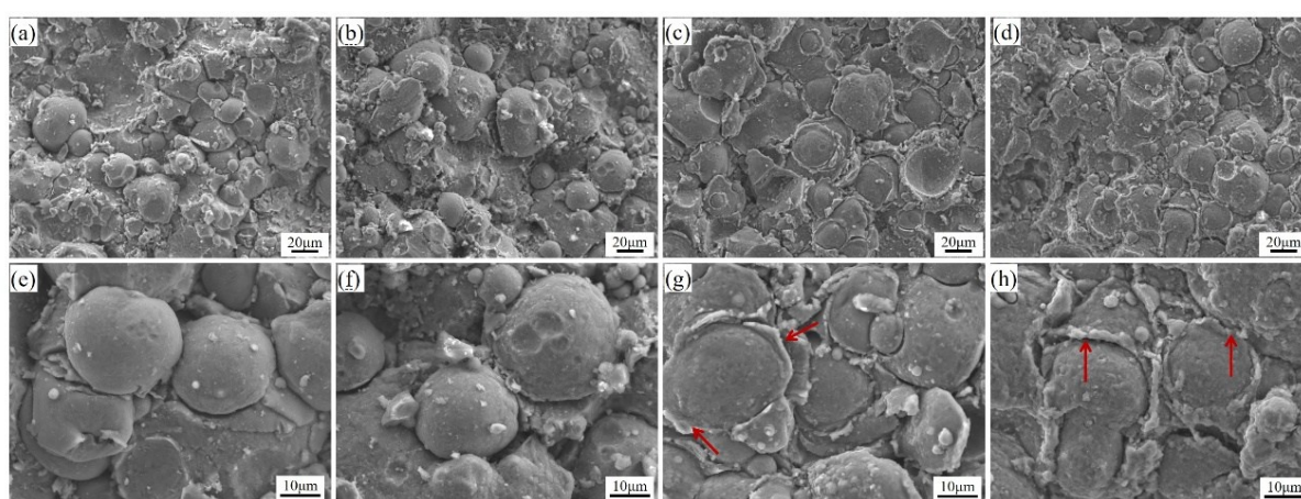
Figure 5-17 Surface morphologies of the 7075Al and TiB 2 /7075Al composite particles deposited at C1 and C3: (a) and (e) 7075Al-C1; (b) and (f) TiB 2 /7075Al-C1; (c) and (g) 7075Al-C3; (d) and (h) TiB 2 /7075Al-C3.
