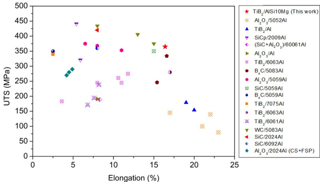
Figure 4-43 Comparison of the UTS and elongation of the FSPed TiB_2/AlSi10Mg composite deposits with other FSP fabricated Al matrix composites [21-26] [17, 20, 27-34].
