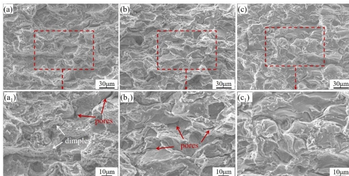
Figure 5-33 Fracture morphologies of the as-sprayed TiB_2/7075 Al composite tensile samples fabricated using different processing conditions: (a) C1; (b) C2; (c) C3. (a 1 ), (b 1 ) and (c 1 ) are the magnified images of the red dashed area in (a), (b) and (c), respectively.
