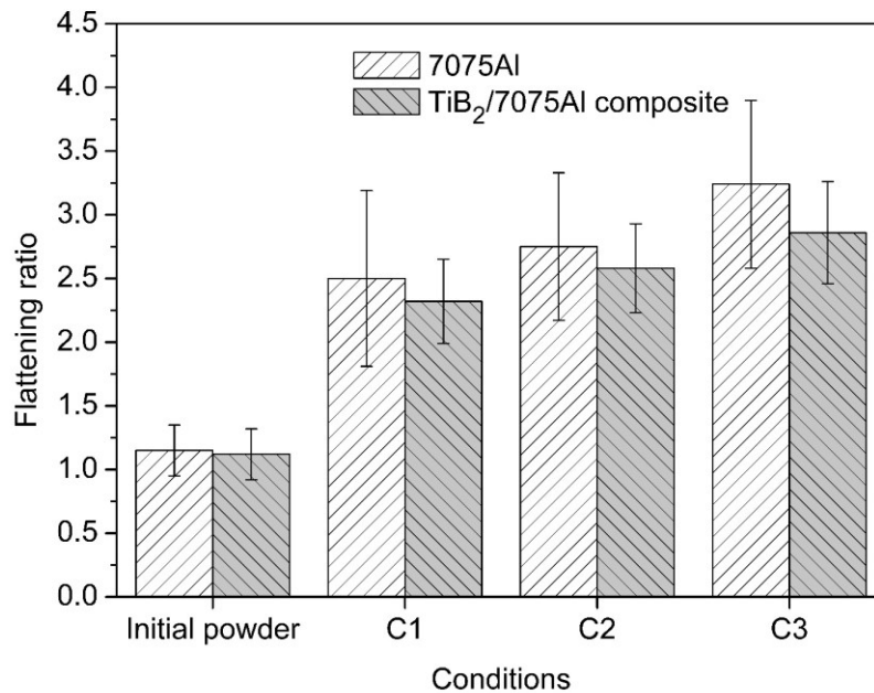
Figure 5-21 Particle flattening ratio evolution of the pure 7075Al and TiB_2/7075Al composite particle under different processing conditions.
