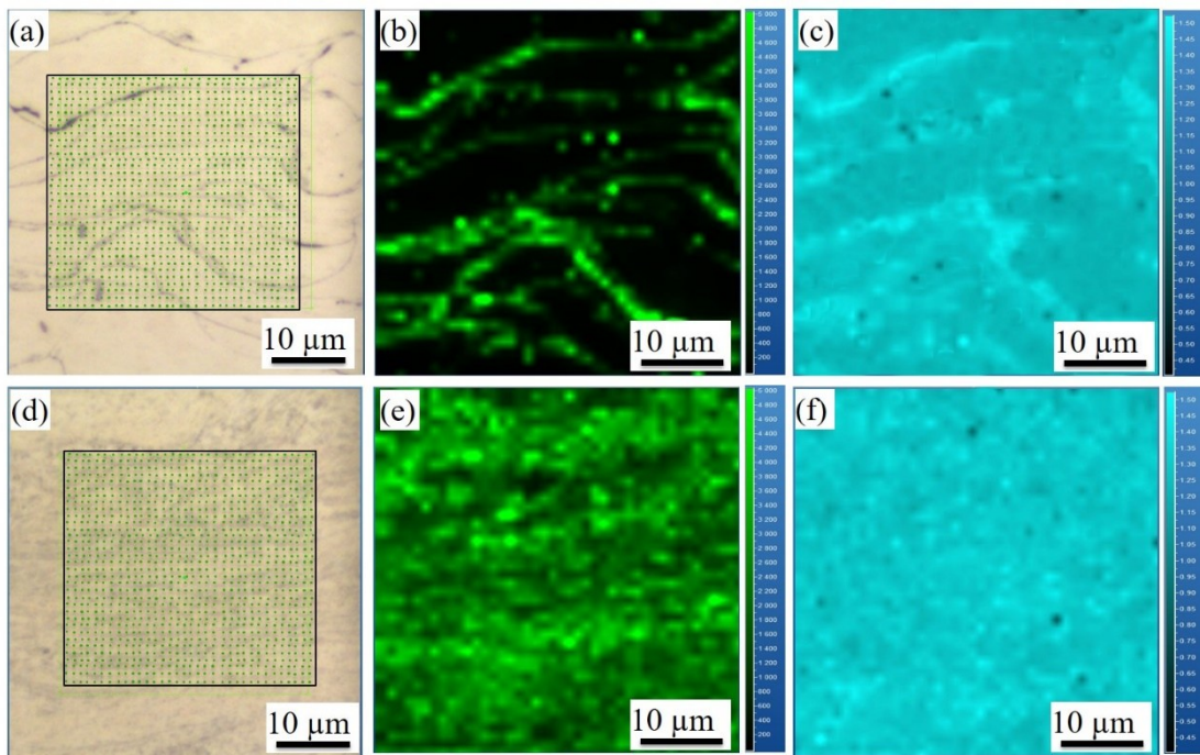
Figure 3-14 Raman spectra mapping of the (a-c) HSD coating and (d-f) SSBM coating fabricated at P_g=550 ^{\circ}\text{C} : (a) and (d) Optical micrographs; (b) and (e) Corresponding confocal Raman maps of G-band intensity ( 1520\text{--}1650 \text{cm}^{-1} ); (c) and (f) Maps of I_D/I_G ratio value.
