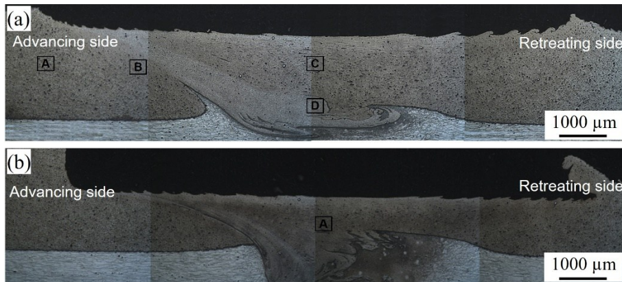
Figure 4-28 Optical micrographs showing the cross-section of the FSPed TiB_2/AlSi10Mg deposits: (a) 1 pass; (b) 3 passes.
