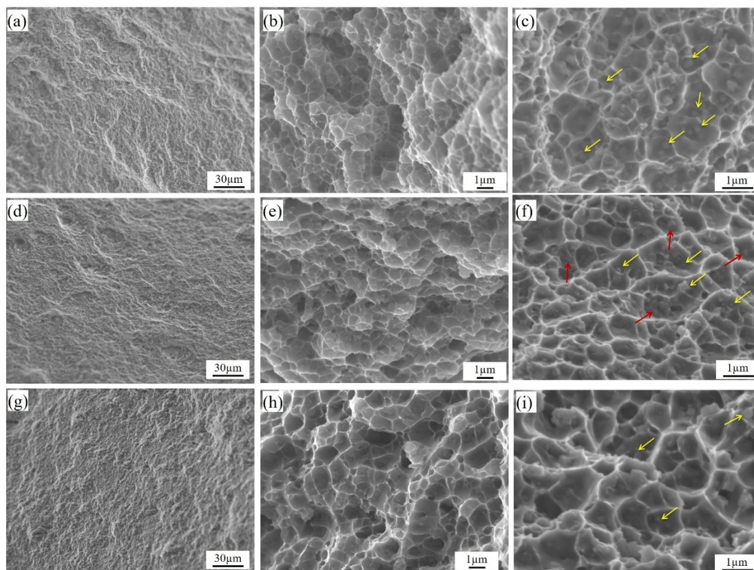
Figure 4-44 SEM micrographs of the tensile fracture surface of the FSPed AlSi10Mg and TiB_2/AlSi10Mg composites with different magnifications: (a-c) AlSi10Mg-FSP-1 pass; (d-f) TiB_2/AlSi10Mg -FSP-1 pass; (g-i) AlSi10Mg-FSP-3 passes.
