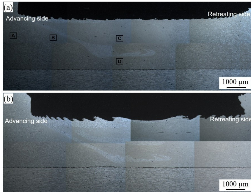
Figure 4-27 Optical micrographs showing the cross-section of the FSPed AlSi10Mg deposits: (a) 1 pass; (b) 3 passes.
