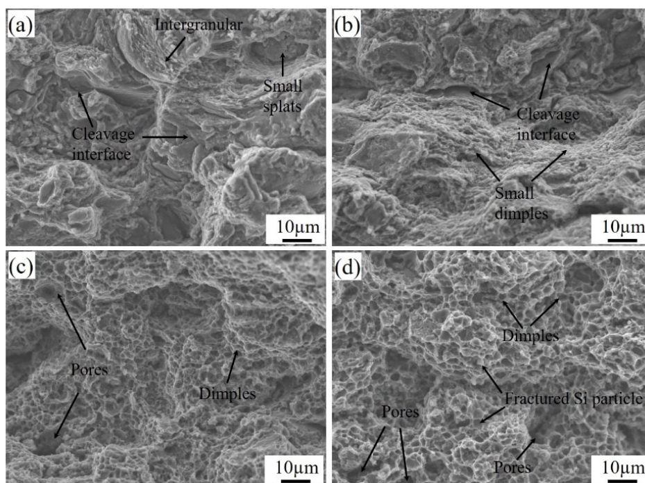
Figure 4-22 Fracture morphologies of the as-sprayed and annealed AlSi10Mg-CT2 deposits after the tensile test: (a) as-sprayed state; (b) 300 ^{\circ}C ; (c) 400 ^{\circ}C ; (d) 500 ^{\circ}C .
