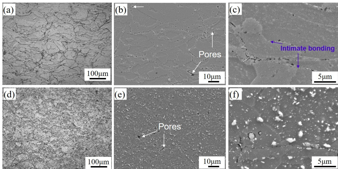
Figure 5-44 Optical and SEM micrographs of the etched cross-section of the (a-c) pure 7075Al-C2 and (d-f) TiB_2/7075Al-C2 composite deposits after 412\text{ }^\circ\text{C}/4\text{ h} + T6 treatment. (a) and (d) are the optical micrographs; (b, c) and (e, f) are the SEM images.
