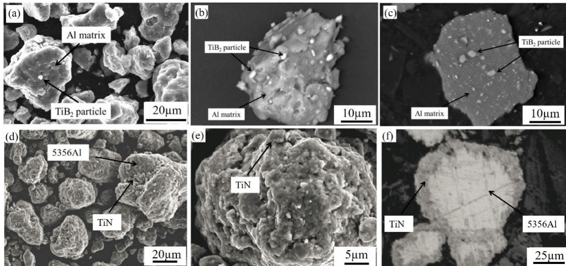
Figure 1-12 Surface morphologies and cross-section views of the ball-milled composite powder for CS deposition: (a-c) TiB 2 /Al [109]; (d-f) TiN/5356Al [110].
