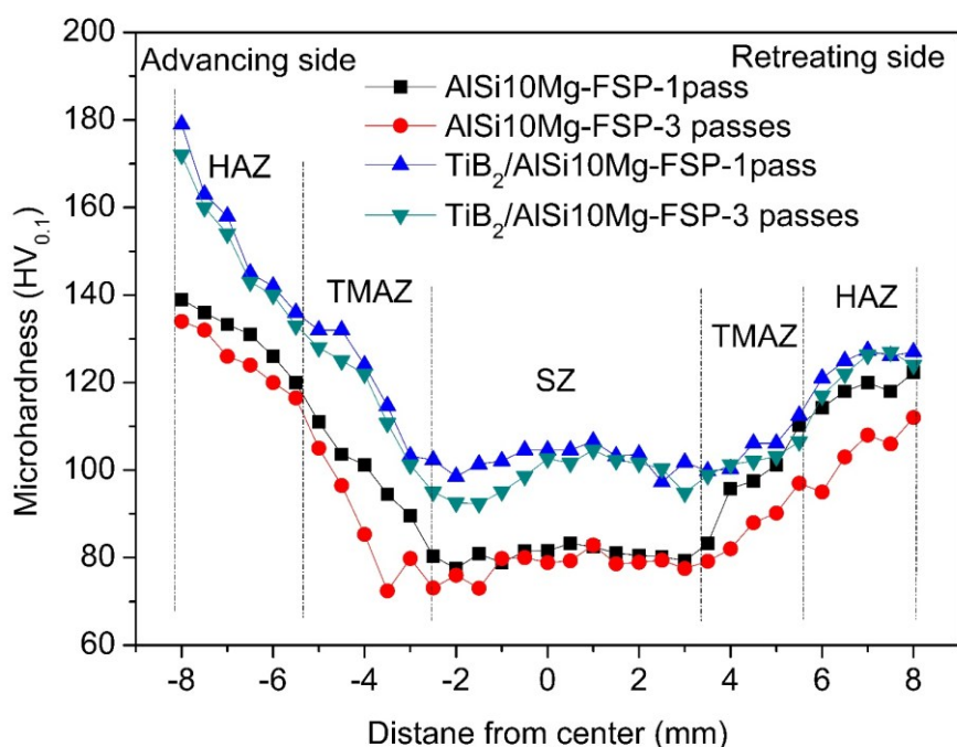
Figure 4-38 Microhardness values of FSPed AlSi10Mg and TiB_2/AlSi10Mg composite samples.
