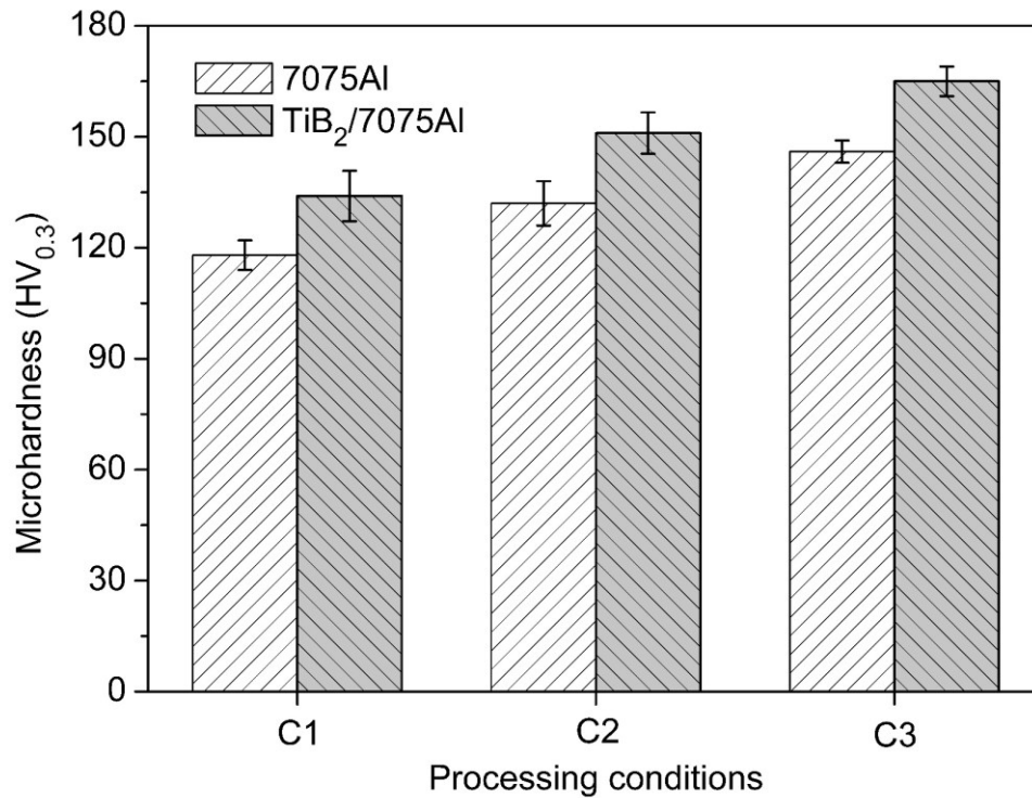
Figure 5-28 Microhardness evolution of the pure 7075Al and TiB_2/7075Al composite deposits in different processing conditions.
