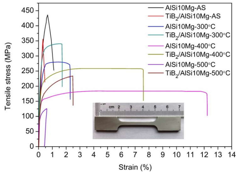
Figure 4-20 Tensile stress-strain curves for pure AlSi10Mg-CT2 and TiB_2/AlSi10Mg -CT2 composites in as-sprayed state and annealing treated at different temperatures.
