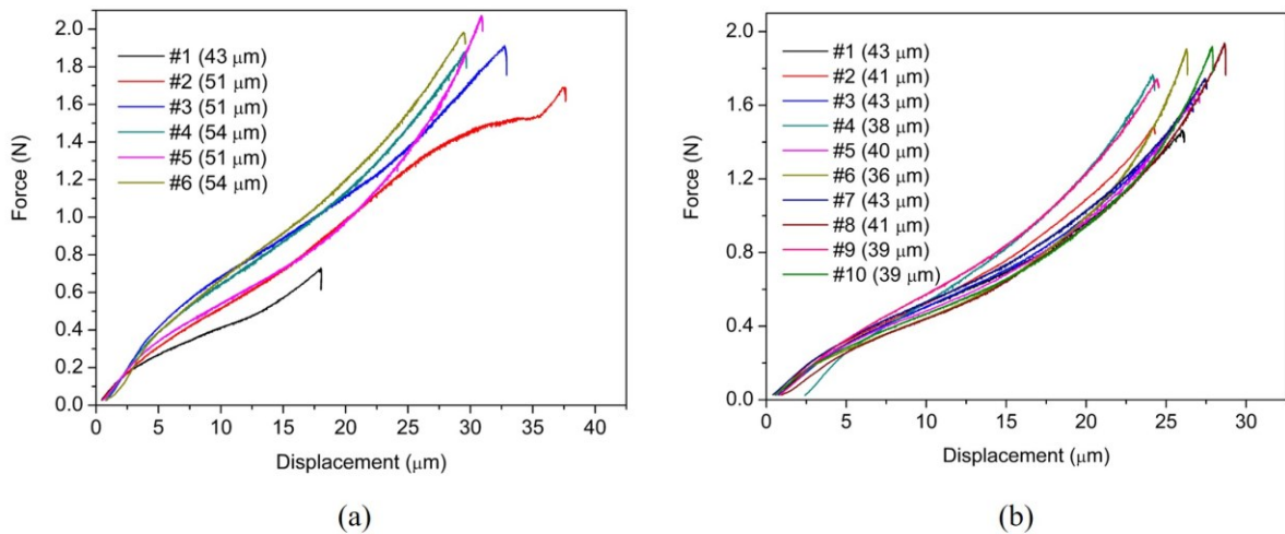
Figure 5-2 Raw force-displacement data of pure 7075Al particles and TiB_2/7075Al composite particles obtained from single particle compress experiment.
