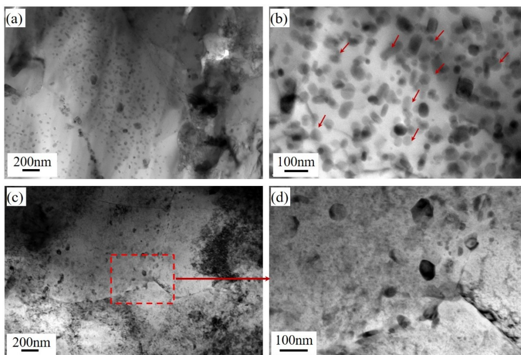
Figure 5-48 TEM micrographs of the (a, b) TiB_2/707Al-C1 and (c, d) TiB_2/707Al-C3 composite samples after T6 treatment.
