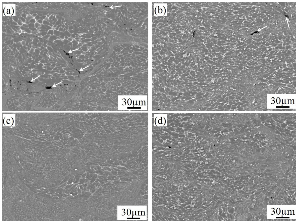
Figure 5-19 BSE/SEM micrographs of the microstructure of the (a, c) 7075Al and (b, d) TiB_2/7075Al composite coatings: (a) 7075Al-C1, (b) TiB_2/7075Al -C1, (c) 7075Al-C3, (d) TiB_2/7075Al -C3. The white arrows indicate pores in the coatings.
