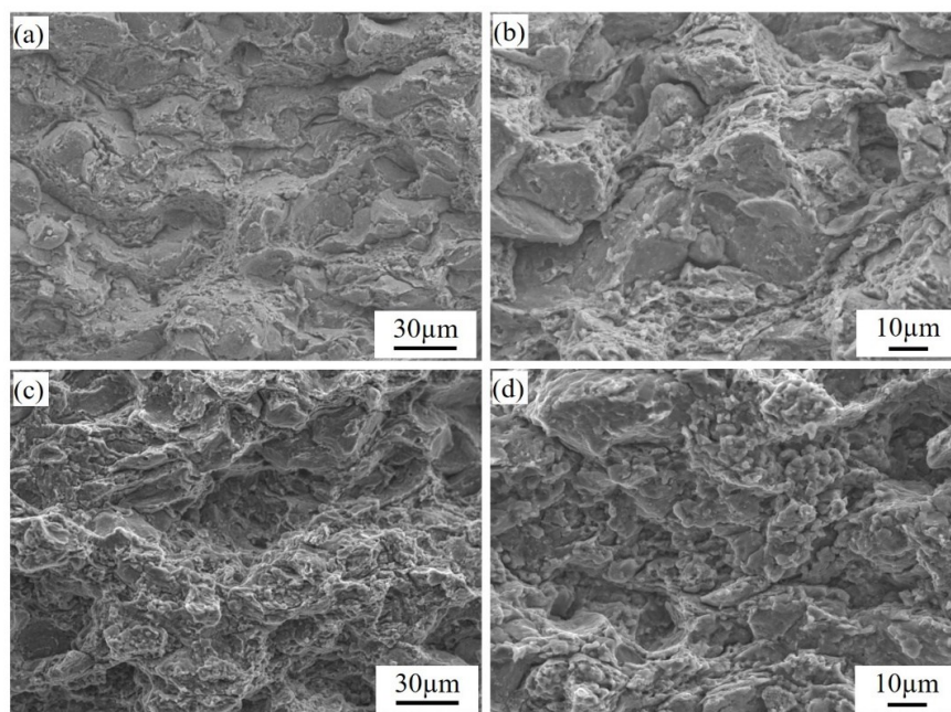
Figure 5-50 The fracture morphologies of the TiB_2/7075Al composite deposits after T6 treatment: (a) and (b) TiB_2/7075Al -C1; TiB_2/7075Al -C2.
