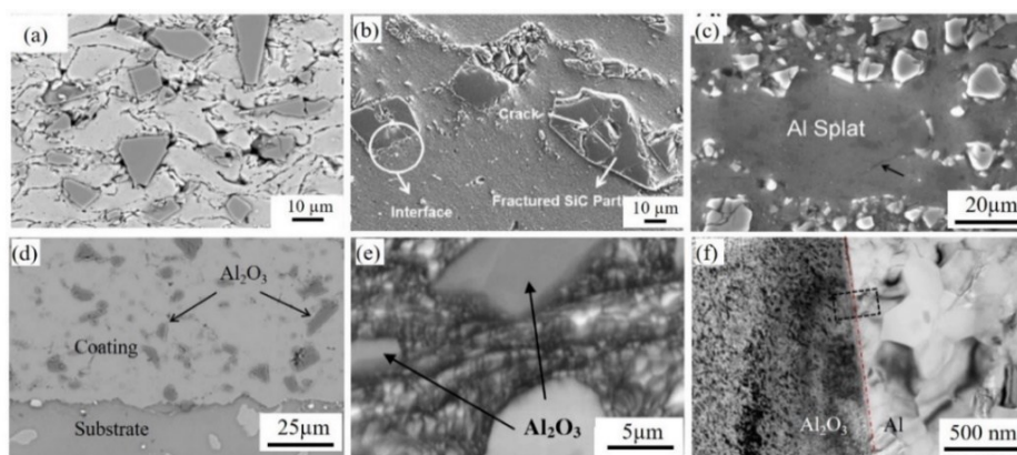
Figure 1-22 Microstructure of the as-sprayed composite coatings obtained from mechanical blending method: (a) Al_2O_3/Al coating [128]; (b) SiC/5056Al coating [122]; (c) SiC/Al coating [116]; (d) Al_2O_3/Al coating. (e) EBSD pattern quality map on the cross-plane of Al_2O_3/Al coating. (f) TEM micrographs showing the Al/Al_2O_3 interface [116].
