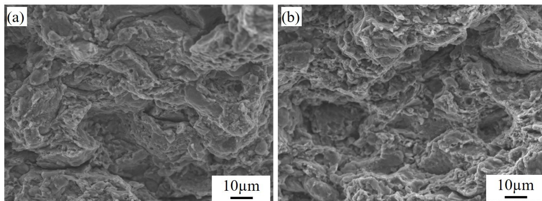
Figure 5-51 The fracture morphologies of the TiB_2/7075Al composite deposits after 412\text{ }^\circ\text{C}/4\text{ h} + \text{T6} treatment: (a) 7075Al-C2; (b) TiB_2/7075Al -C2.
