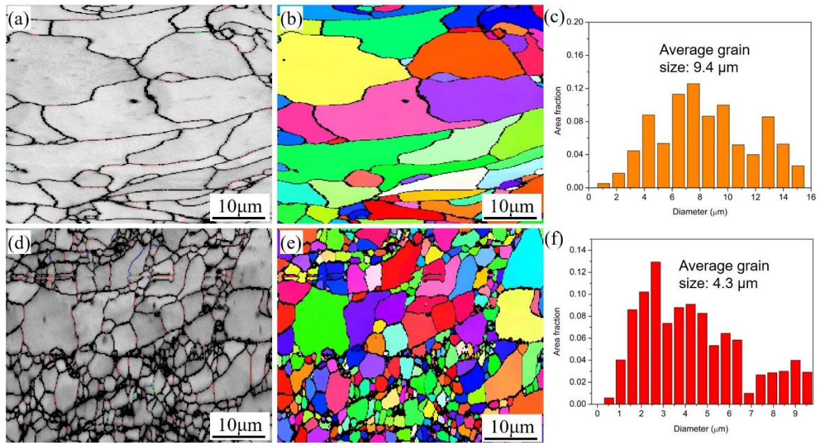
Figure 5-47 EBSD characterization of the (a-c) pure 7075Al-C1 and (d-f) TiB_2/7075Al-C1 composite deposits after T6 treatment: (a) and (d) band contrast; (b) and (e) IPF mapping; (c) and (f) grain size distribution.
