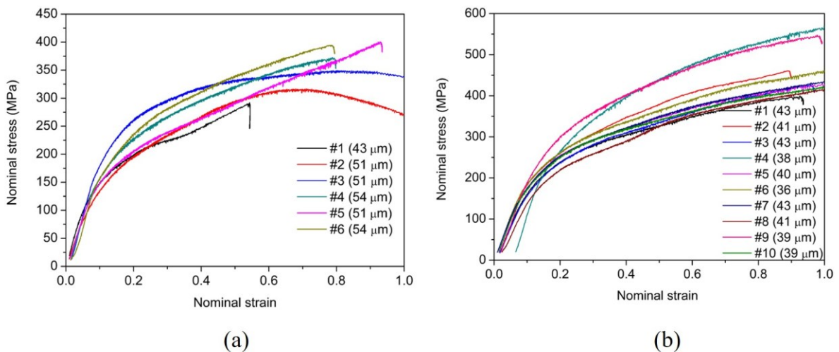
Figure 5-3 Nominal stress-strain converted from force-displacement data: (a) 7075Al particles; (b) TiB_2/7075Al composite particle.
