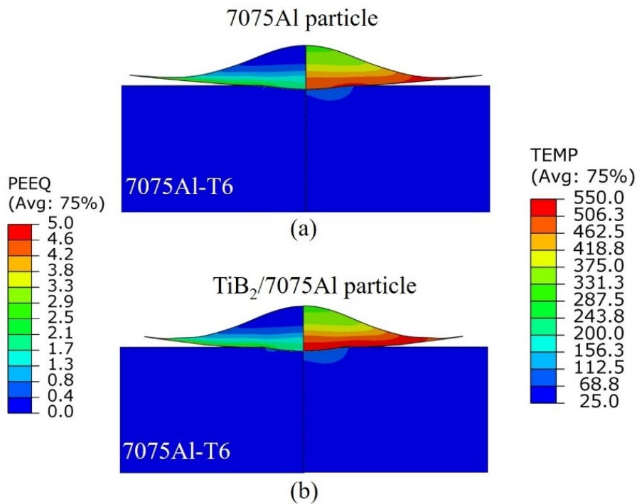
Figure 5-10 Distribution of PEEQ (on the left-hand side) and temperature (on the right-hand side) of the single (a) 7075Al and (b) TiB_2/7075Al composite particles deposited onto 7075Al-T6 substrate in C1.
