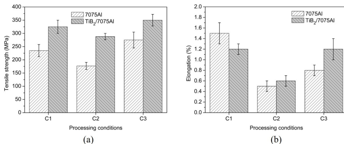
Figure 5-32 Variation of (a) tensile strength and (b) elongation of the as-sprayed 7075Al and TiB_2/7075Al composite samples in different processing conditions.
