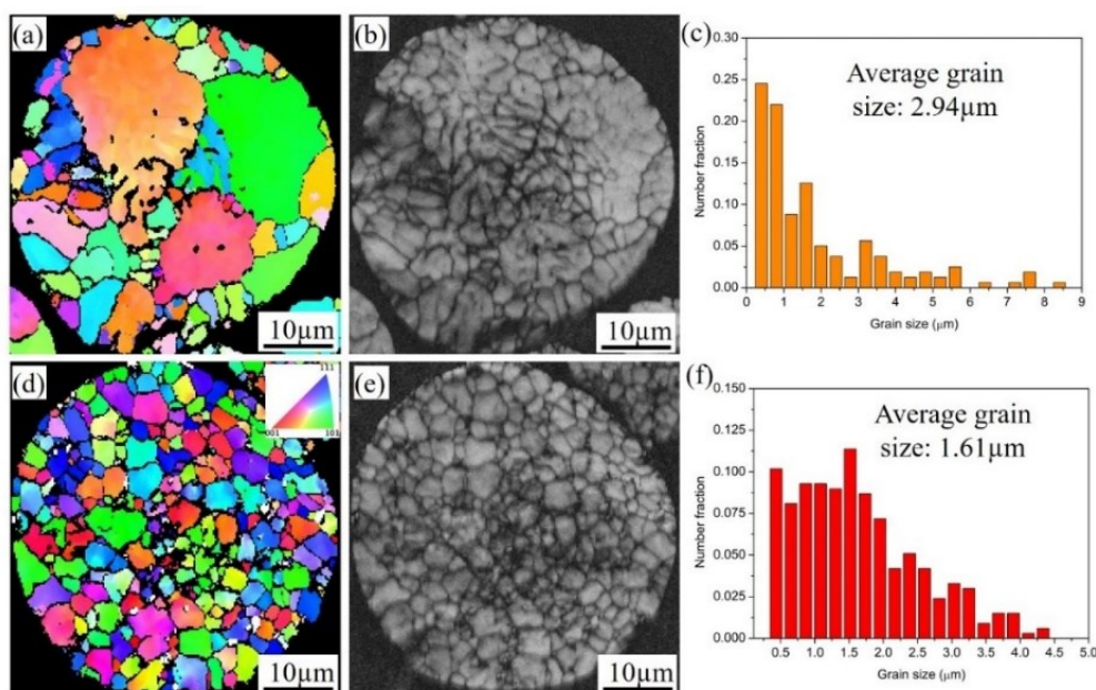
Figure 2-11 SEM/EBSD characterization of the cross-section of the gas-atomized (a-c) 7075Al particle and (d-f) \text{TiB}_2/7075\text{Al} composite particle: (a) and (d) IPF mapping images, (b) and (e) band contrast images, (c) and (f) Al grain size distributions. The image reveals the grains by cleaning up the nanoparticle \text{TiB}_2 phase.
