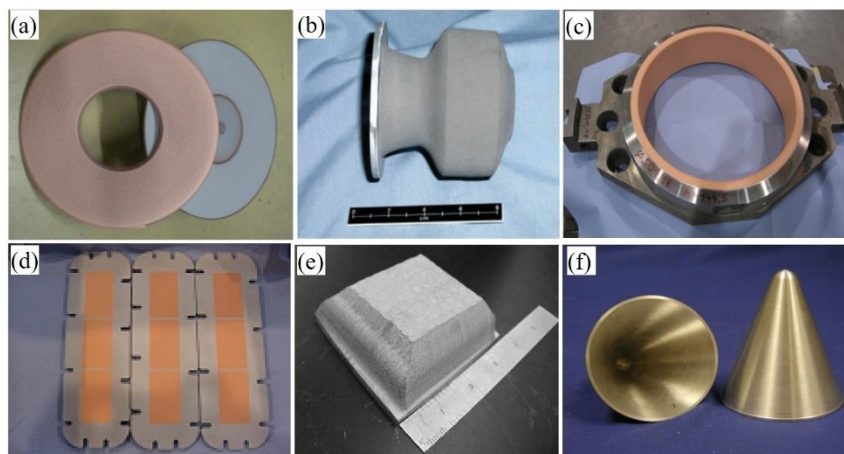
Figure 1-8 Application of cold spraying in net-shape forming: (a) high magnetic field magnets ; (b) rapid prototyping of Ti6Al4V axisymmetric bulk part [79]; (c) thick copper coating inside a pressure ring for food processing machine [82]; (d) electronic heat sinks [82]; (e) bulk Ni/Al energetic material [83]; (f) Cu/W cone structure [84].
