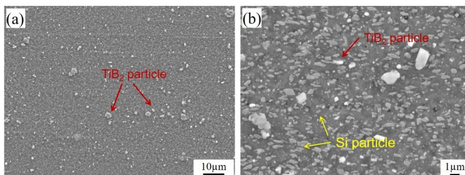
Figure 4-36 SEM images of the cross-section of the FSPed TiB_2/AlSi10Mg deposits in SZ as marked in Figure 4-28b.
