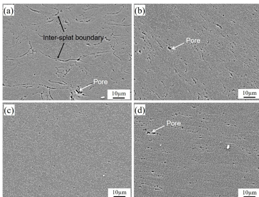
Figure 4-31 SEM images of the FSPed AlSi10Mg deposit in different regions corresponding to the A, B, C and D as marked in Figure 4-27.
