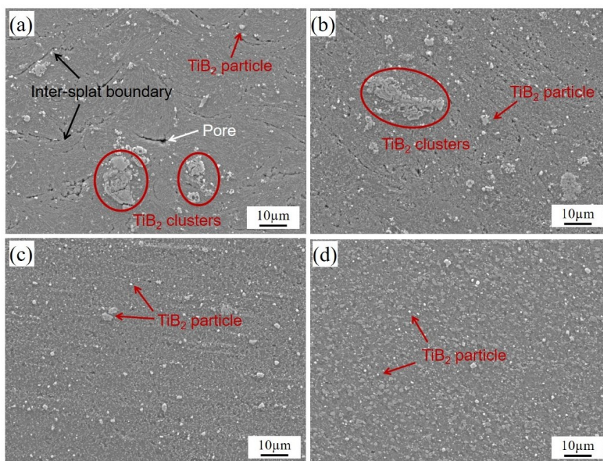
Figure 4-34 SEM images of the cross-section of the FSPed TiB_2/AlSi10Mg deposits in different regions corresponding to the A, B, C and D as marked in Figure 4-28a.
