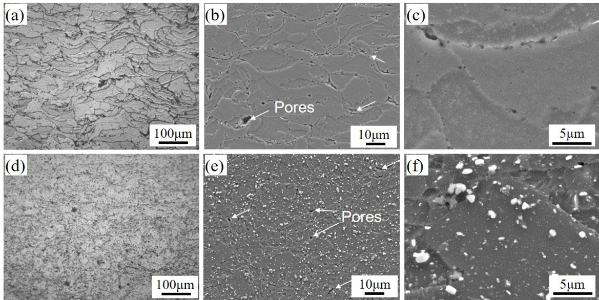
Figure 5-43 Optical and SEM micrographs of the etched cross-section of the (a-c) pure 7075Al-C2 and (d-f) TiB_2/7075Al-C2 composite deposits after 470\text{ }^\circ\text{C}/4\text{ h} (water quenching) + 121\text{ }^\circ\text{C}/24\text{ h} treatment. (a) and (d) are the optical micrographs; (b, c) and (e, f) are the SEM images.
