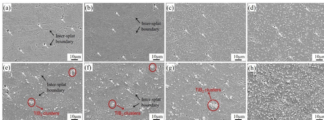
Figure 4-9 SEM micrographs of the etched cross-sections of the annealed (a-d) AlSi10Mg-CT2 and TiB_2/AlSi10Mg -CT2 composite samples at a lower magnification: (a) and (e) 200 °C; (b) and (f) 300 °C; (c) and (g) 400 °C; (d) and (h) 500 °C.
