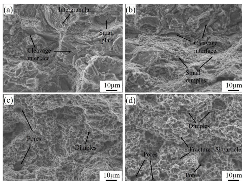
Figure 4-22 Fracture morphologies of the as-sprayed and annealed AlSi10Mg-CT2 deposits after the tensile test: (a) as-sprayed state; (b) 300 °C; (c) 400 °C; (d) 500 °C.
