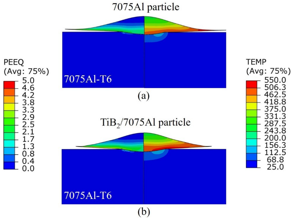
Figure 5-11 Distribution of PEEQ (on the left-hand side) and temperature (on the right-hand side) of the single (a) 7075Al and (b) TiB_2/7075Al composite particles deposited onto 7075Al-T6 substrate in C2.
