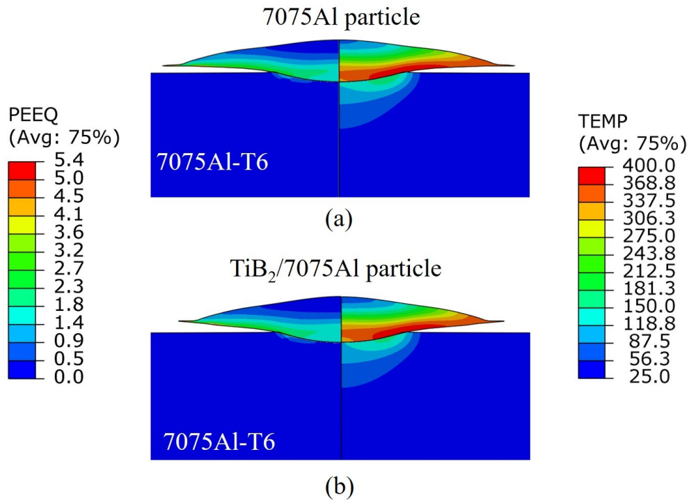
Figure 5-12 Distribution of PEEQ (on the left-hand side) and temperature (on the right-hand side) of the single (a) 7075Al and (b) TiB_2/7075Al composite particles deposited onto 7075Al-T6 substrate in C3.
