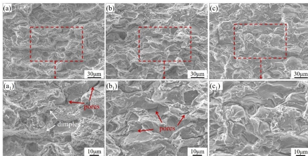
Figure 5-33 Fracture morphologies of the as-sprayed TiB_2/7075 Al composite tensile samples fabricated using different processing conditions: (a) C1; (b) C2; (c) C3. (a 1 ), (b 1 ) and (c 1 ) are the magnified images of the red dashed area in (a), (b) and (c), respectively.
