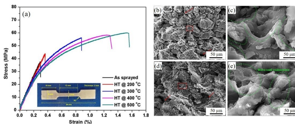
Figure 1-31 Tensile stress-strain plots of as-sprayed and heat-treated B 4 C/Al composite samples. Fracture morphologies of (b and c) as-sprayed and heat-treated (500 °C) B 4 C/Al composite samples [101].
