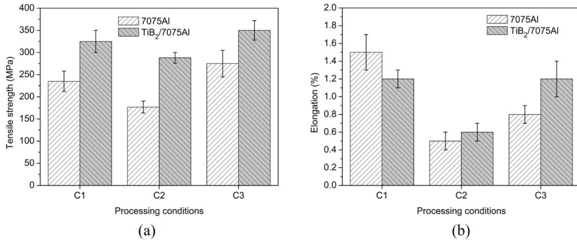
Figure 5-32 Variation of (a) tensile strength and (b) elongation of the as-sprayed 7075Al and TiB_2/7075Al composite samples in different processing conditions.
