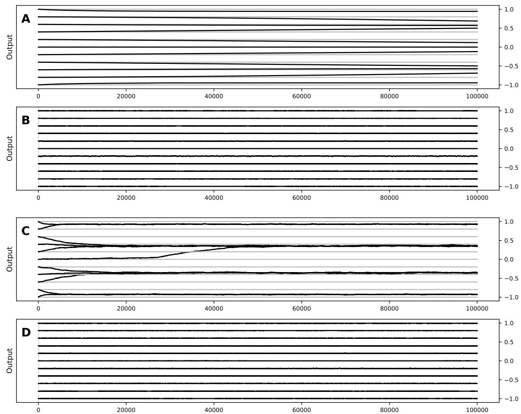
FIGURE 6.5: Stability comparison with or without concepton, with or without noise. Black: Evolution of the readout y . lines: the discrete value considered. Light areas: time when conceptons are computed for the current value. A-B No noise. C-D 0.0001 noise. A and C No concepton used. B and D Discrete concepton are applied.
