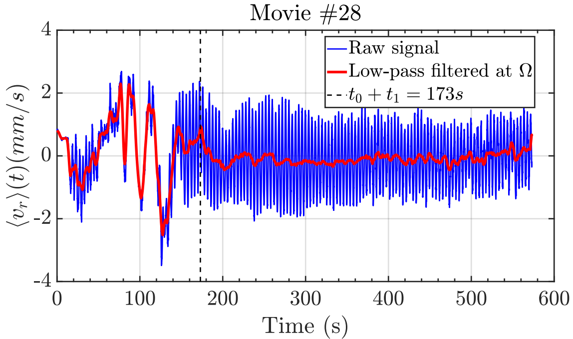
Figure 4.10: On each frame, the average of the horizontal velocity of all the tracked particles is computed: \langle v_r \rangle(t) . The first 173s of this data set have been recorded during a transient state, hence the irregular shape of the signal. After these 173s, the particles oscillate all together in phase with the cryostat rotation. When using a filter which cuts off frequencies above \Omega , the red signal is obtained. Its constancy indicates that no frequencies below \Omega are excited in the steady state, allowing phase detection for the figure 4.12.
