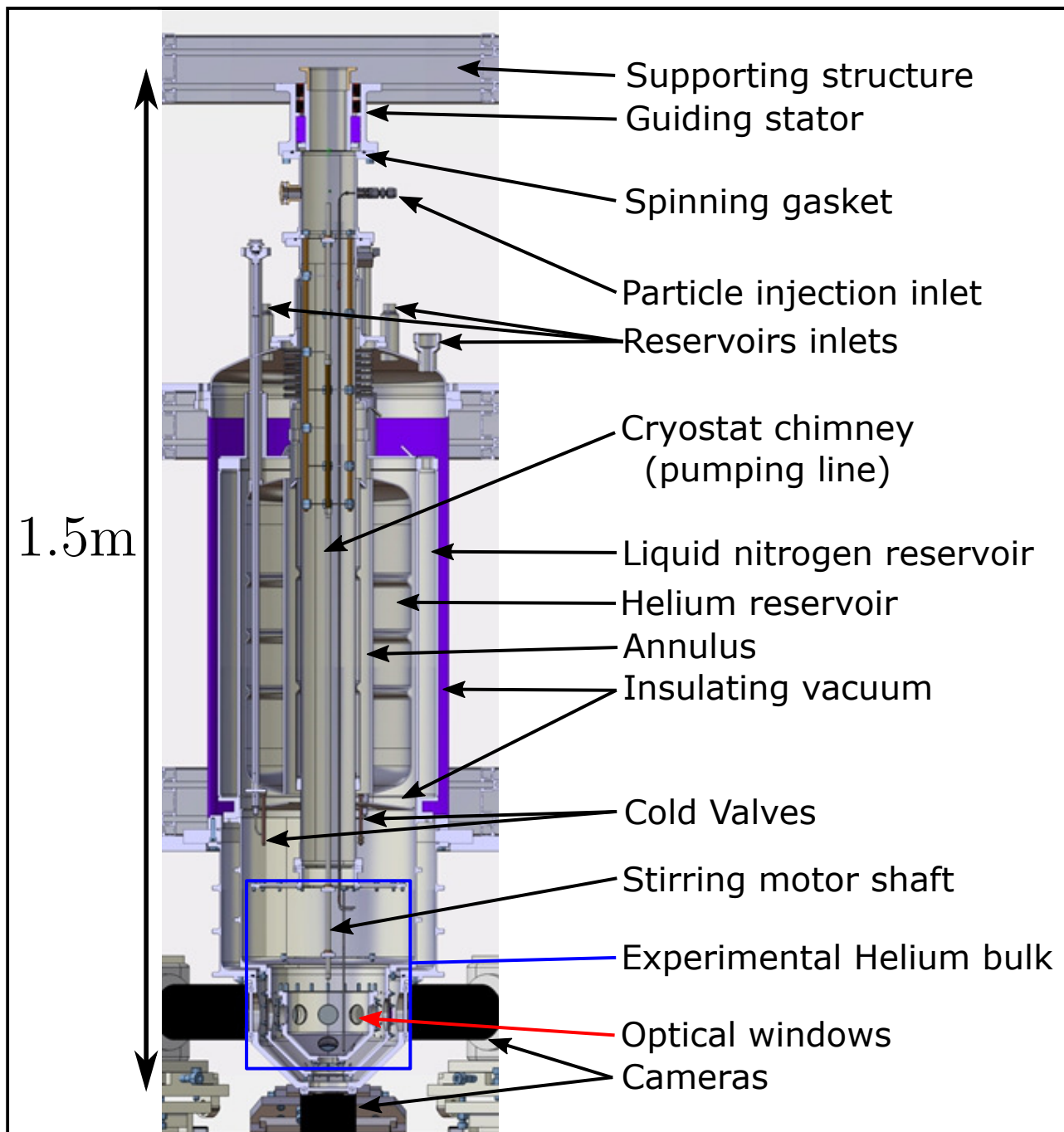
Figure 2.4: Overall labelled drawing of the cryostat
