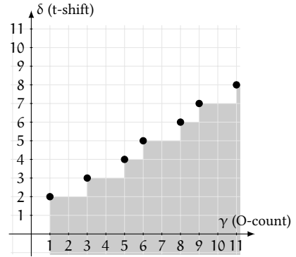
(b) The (O-count/t-shift)-plane for the I-count value 0
