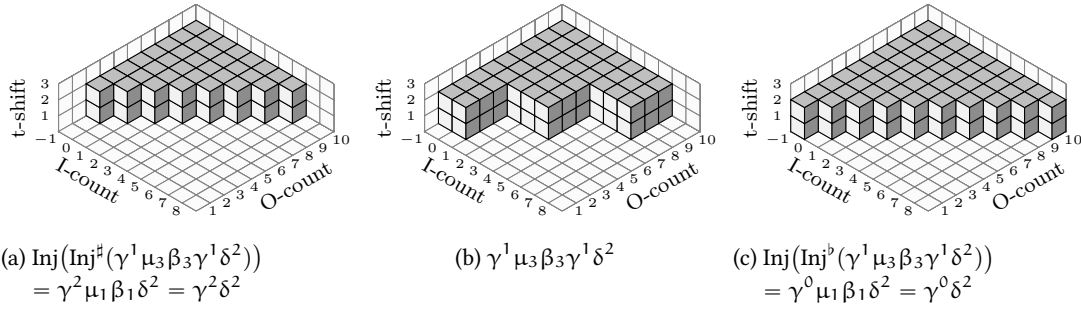
Figure 3.10. – Graphical comparison of \gamma^1 \mu_3 \beta_3 \gamma^1 \delta^2 , \text{Inj}(\text{Inj}^{\#}(\gamma^1 \mu_3 \beta_3 \gamma^1 \delta^2)) and \text{Inj}(\text{Inj}^{\flat}(\gamma^1 \mu_3 \beta_3 \gamma^1 \delta^2)) . For all t \in \mathbb{Z} the slices in the (I/O-count)-planes of \gamma^1 \mu_3 \beta_3 \gamma^1 \delta^2 cover the slices of \text{Inj}(\text{Inj}^{\#}(\gamma^1 \mu_3 \beta_3 \gamma^1 \delta^2)) , but are covered by the slices of \text{Inj}(\text{Inj}^{\flat}(\gamma^1 \mu_3 \beta_3 \gamma^1 \delta^2)) , see Figure 3.11.
