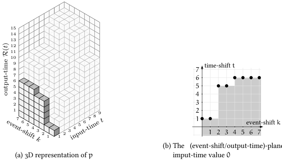
Figure 4.10. – Illustration of the Projection \Psi_4(p) .
