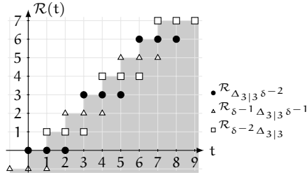
Figure 4.3. \mathcal{R}_e(t) is equal to \max(\mathcal{R}_{\Delta_{3|3} \delta^{-2}}(t), \mathcal{R}_{\delta^{-1} \Delta_{3|3} \delta^{-1}}(t), \mathcal{R}_{\delta^{-2} \Delta_{3|3}}(t)) .
