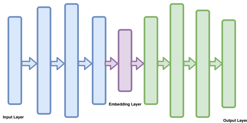
Figure 2.1: An example of Undercomplete Autoencoders. Blue layers represent the encoder and green layers represent the decoder while the purple layer represents the embedding layer.
