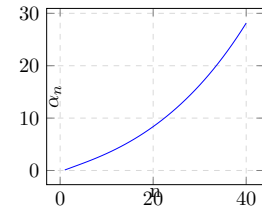
Figure 4.3: Annealing scheme for inverse temperature \alpha , following the sequence \alpha_{n+1} = 2^{1/\log(n)^2} \times \alpha_n ; \alpha_1 = 0.1 .
