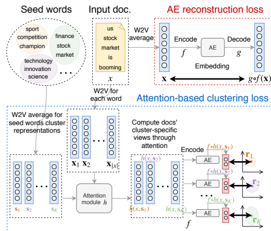
Figure 5.3: Illustration of SDC2-Att. The function h denotes the seed words-based attention module applied to the documents' input representations. Thick double arrows indicate the computation of a distance between two vectors.
