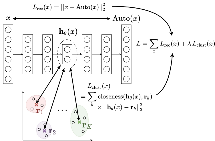
Figure 4.1: Overview of our Deep k -Means approach instantiated with losses based on the Euclidean distance.
