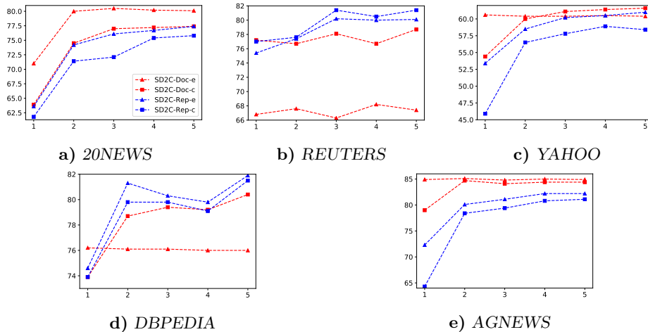
Figure 5.4: Clustering results in terms of ACC for SD2C-Doc-e, SD2C-Doc-c, SD2C-Rep-e and SD2C-Rep-c with 1 to 5 seed words.
