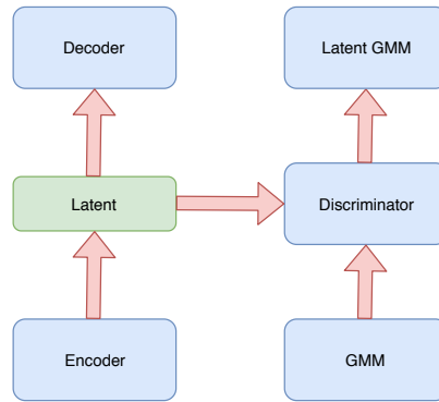
Figure 3.2: AAE architecture.
