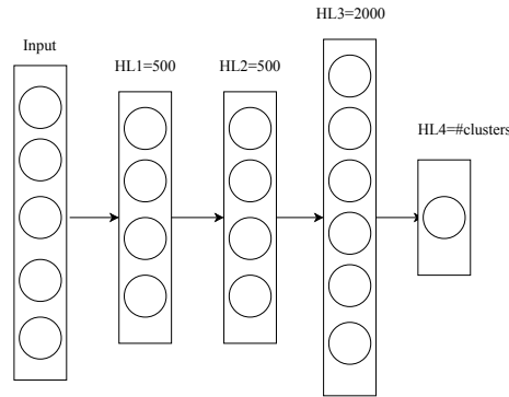
Figure 4.4: The architecture of the encoder part of the Autoencoder.
