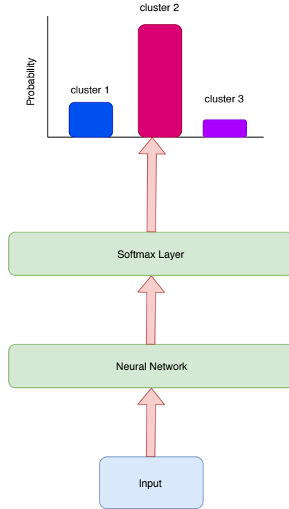
Figure 3.4: Pairwise Clustering Architecture.
