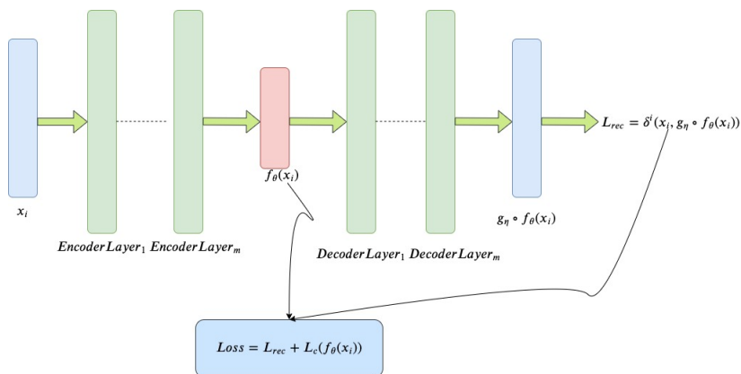
Figure 3.1: General DC architecture.
