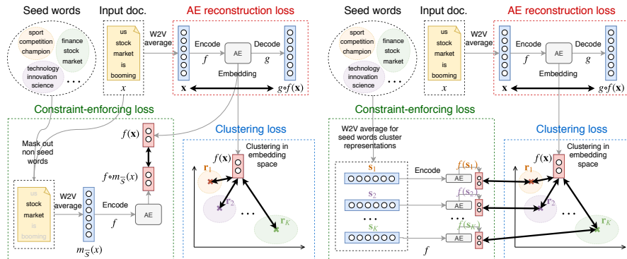
Figure 5.2: Illustration of SD2C-Doc (left) and SD2C-Rep (right). Thick double arrows indicate the computation of a distance between two vectors.
