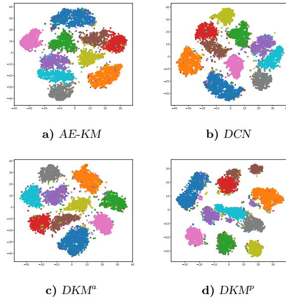
Figure 4.10: t-SNE visualization of the embedding spaces learned on USPS.
