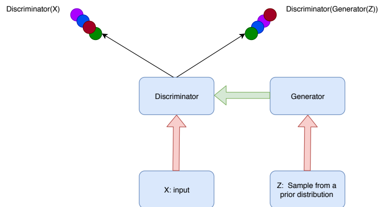
Figure 3.3: CATGAN architecture.
