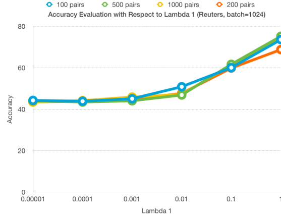
Figure 5.5: Evolution of PCD2C in the case of clustering accuracy (ACC) for REUTERS with respect to different values for \lambda_1 for different number of pairs—when pairwise constraints are used.
