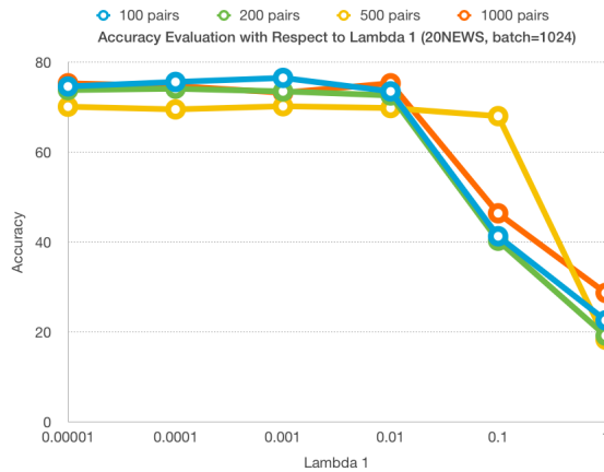
Figure 5.6: Evolution of PCD2C in the case of clustering accuracy (ACC) for 20NEWS with respect to different values for \lambda_1 for different number of pairs—when pairwise constraints are used.
