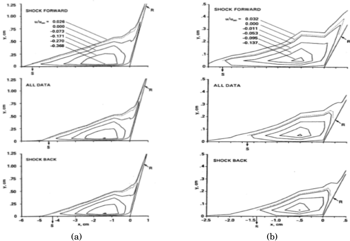
Figure 1.16: The contours of the mean velocity at two different shock angle 23^\circ (a) and 5^\circ (b). From [94].
