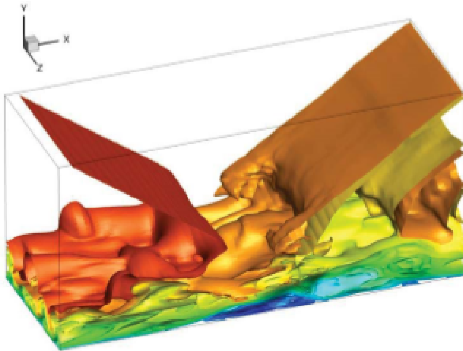
Figure 1.31: Isosurface of instantaneous streamwise velocity in the interaction region. From [85].
