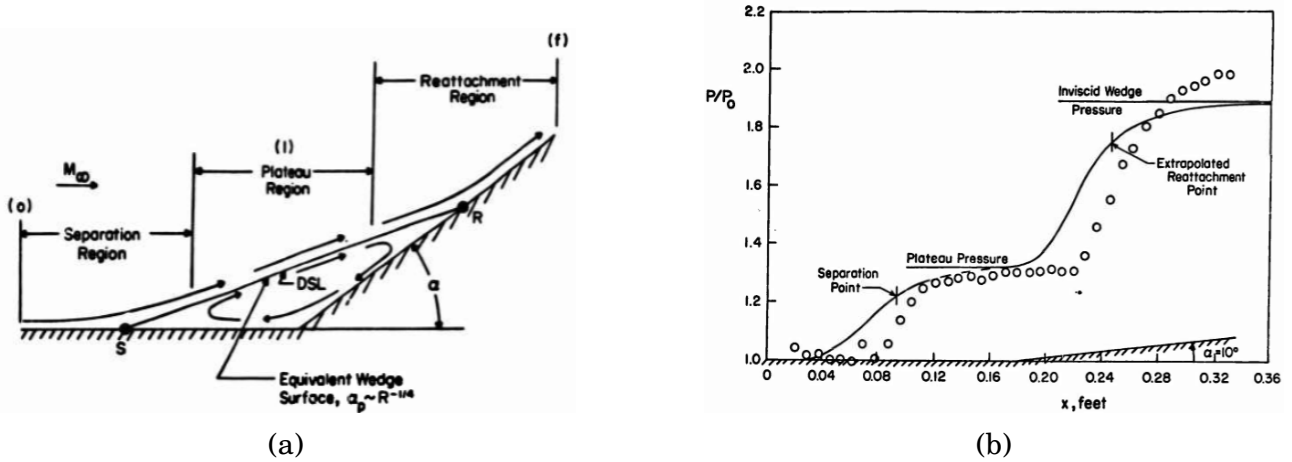
Figure 1.11: Laminar separation in compression ramp (a) and the theoretically calculated overall pressure distribution (b) at ramp angle 10^\circ . From [25].
