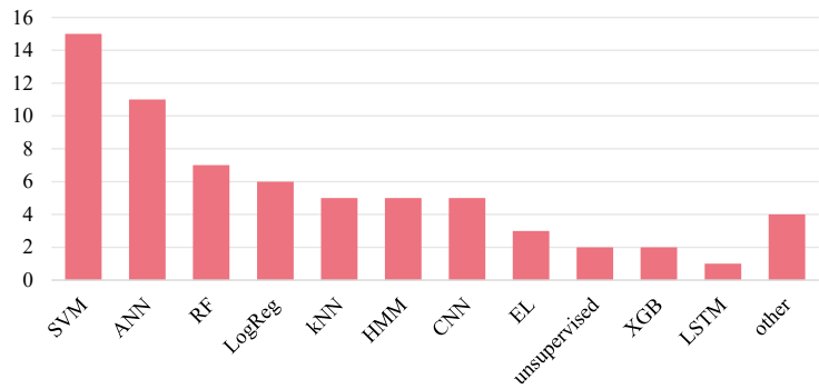
(b) Main ML model used.
