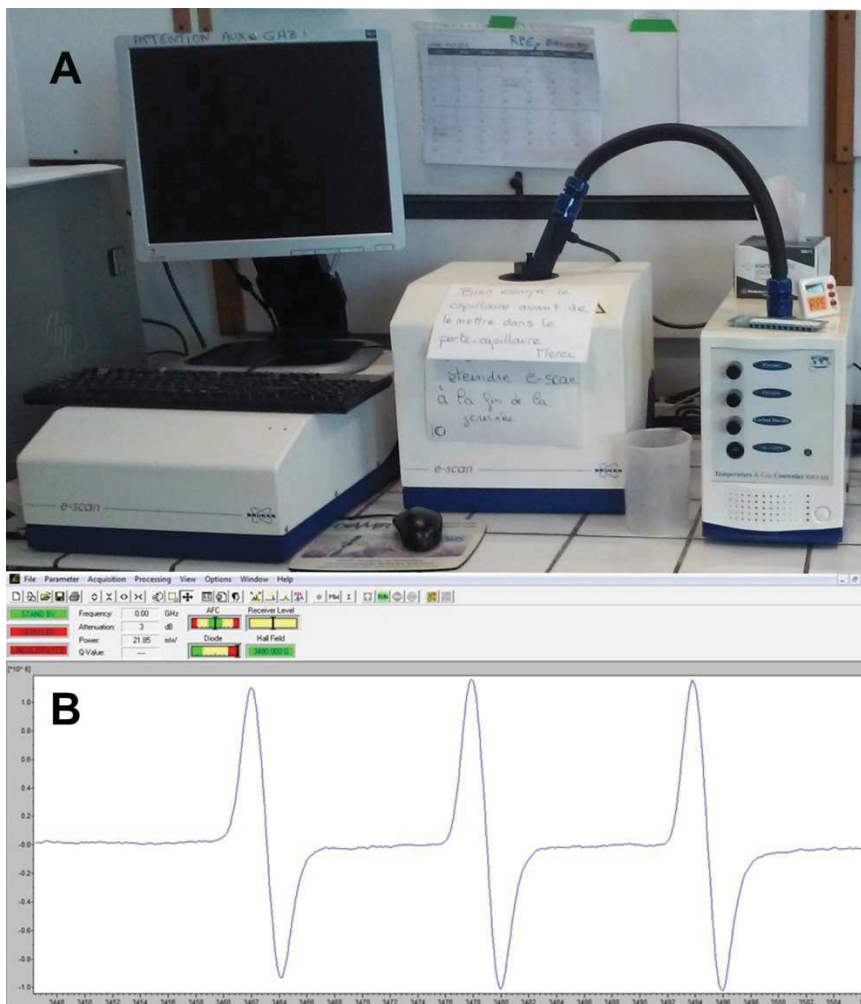
Fig. 18. EPR device (A) with analyzing software (B).
