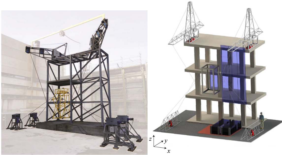
Figure 1.5 – Hephaestus prototype and an illustration of its main application, the installation of curtain wall modules.
