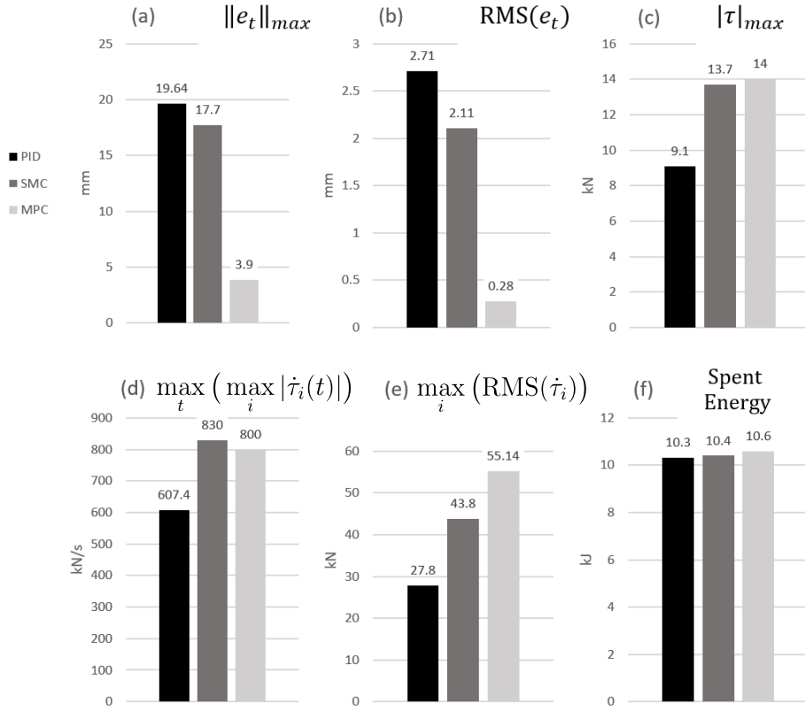
Figure 3.4 – Comparative results: (a) maximal errors, (b) RMS errors, (c) maximal cable tensions, (d) maximal cable tension derivatives, (e) RMS of cable tension derivatives, and (f) consumed energy.
