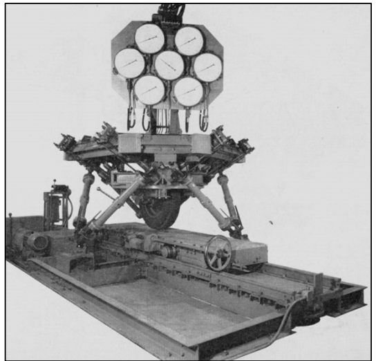
Figure 3: Figures showing the first designs of hexapod proposed by D. Stewart (left) and V. E. Gough (right) [Stewart, 1965]
