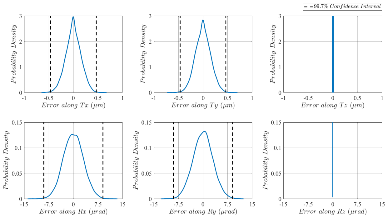
Figure D.4: Probability density functions of the output errors (compensation errors)
