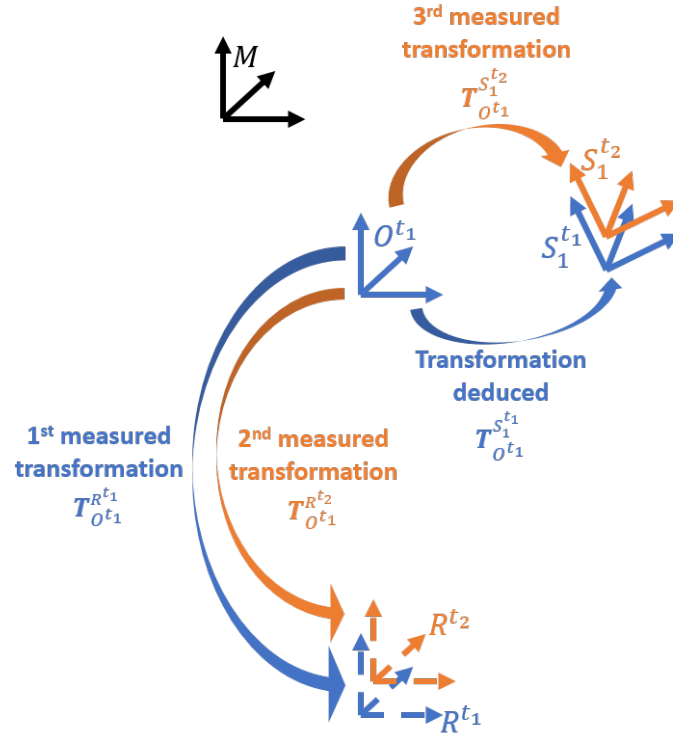
Figure H.2: Illustration of the thermal deflection decoupled pose measurement method to measure the pose of an arbitrary coordinate frame S_1 with respect to a coordinate frame O
