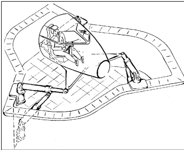
Figure 3: Figures showing the first designs of hexapod proposed by D. Stewart (left) and V. E. Gough (right) [Stewart, 1965]
