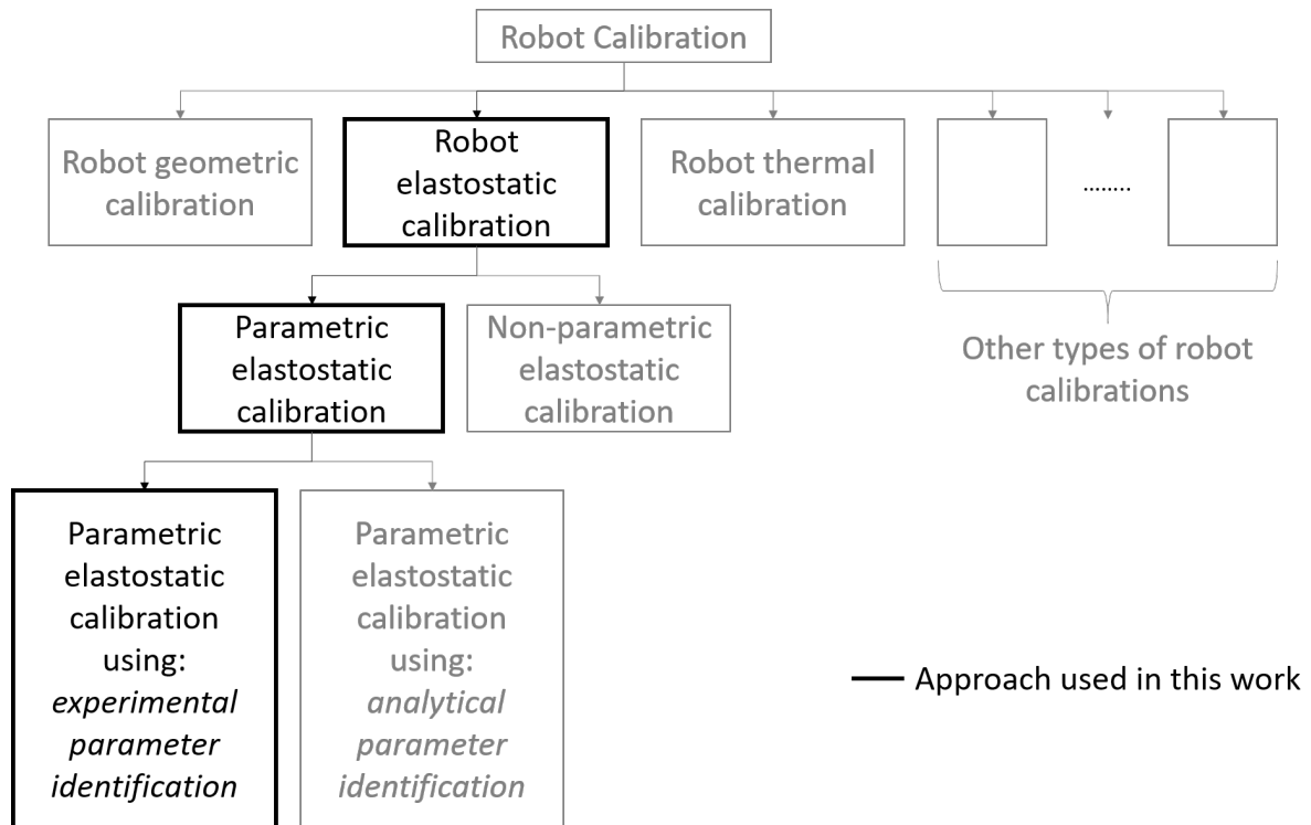
Figure 1.4: Classification of robot calibration approaches
