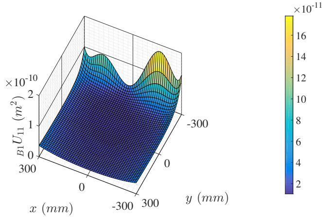
Figure 3.3: Plot showing values of DUIR criterion ( {}_{B1}U_{11} ) for the elastostatic calibration of simulation study 1 (position having the lowest value of {}_{B1}U_{11} is the best position for stiffness identification as per DUIR criterion in this case)
