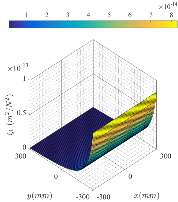
Figure 3.8: \zeta_1 values for different identification positions across the workspace of the bipod
