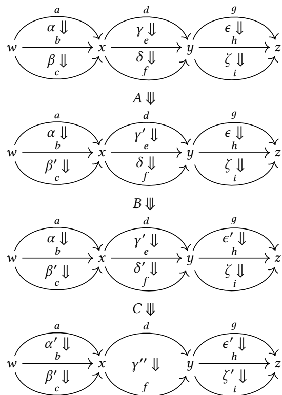
Figure 3.8 – The \omega -hypergraph P
