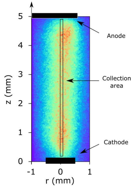
Figure 8.21 Collection area compared to the typical emission of the nanosecond discharge under the PASTEC conditions ( \Phi = 0.8, f = 20 \text{ kHz}, E_{pulse} = 2 \text{ mJ} ).
