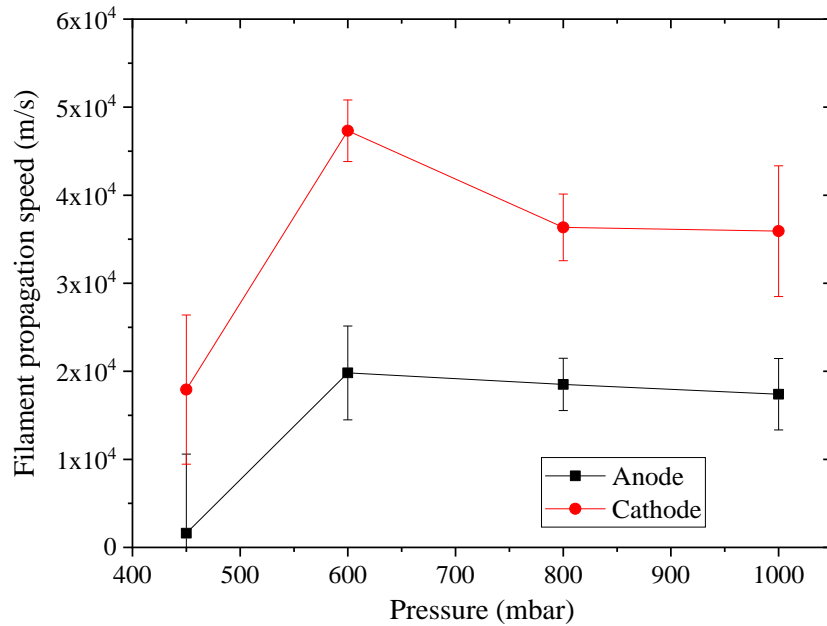
Figure 4.5 Propagation speed of the filaments from 400 mbar to 1 bar. At the anode, the speed is relatively constant \approx 20 \mu\text{m} \cdot \text{ns}^{-1} . The speed of propagation of the cathode filament is of the same order of magnitude, with a peak at 5 \times 10^4 \text{ m} \cdot \text{s}^{-1} = 50 \mu\text{m} \cdot \text{ns}^{-1} .
