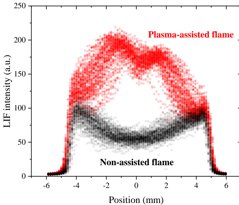
Figure 8.13 LIF signal along the bluff-body under the PASTEC conditions ( \Phi = 0.8, f = 20 kHz, E_{pulse} = 2 mJ). The data are acquired before the application of the NRP discharges (black dots) and when the NRP discharges are applied at steady state (red dots). Each set comprises 100 shots.
