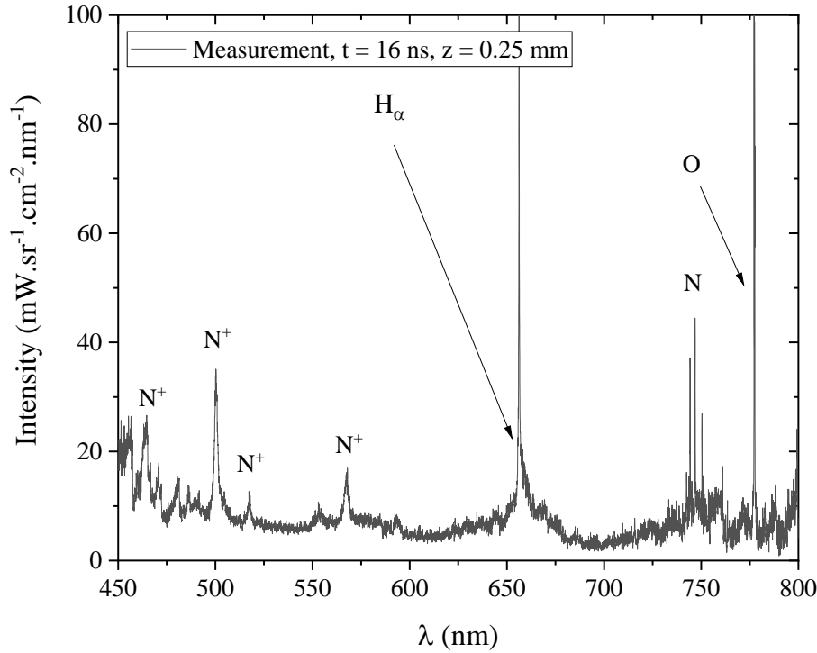
Figure 8.43 Near-cathode emission ( z = 0.25 mm) at t = 16 ns under the PASTEC conditions ( \Phi = 0.8 , f = 20 kHz, E_{pulse} = 2 mJ). The N_2(B) spectrum is not visible due to the intense atomic and continuum emission.
