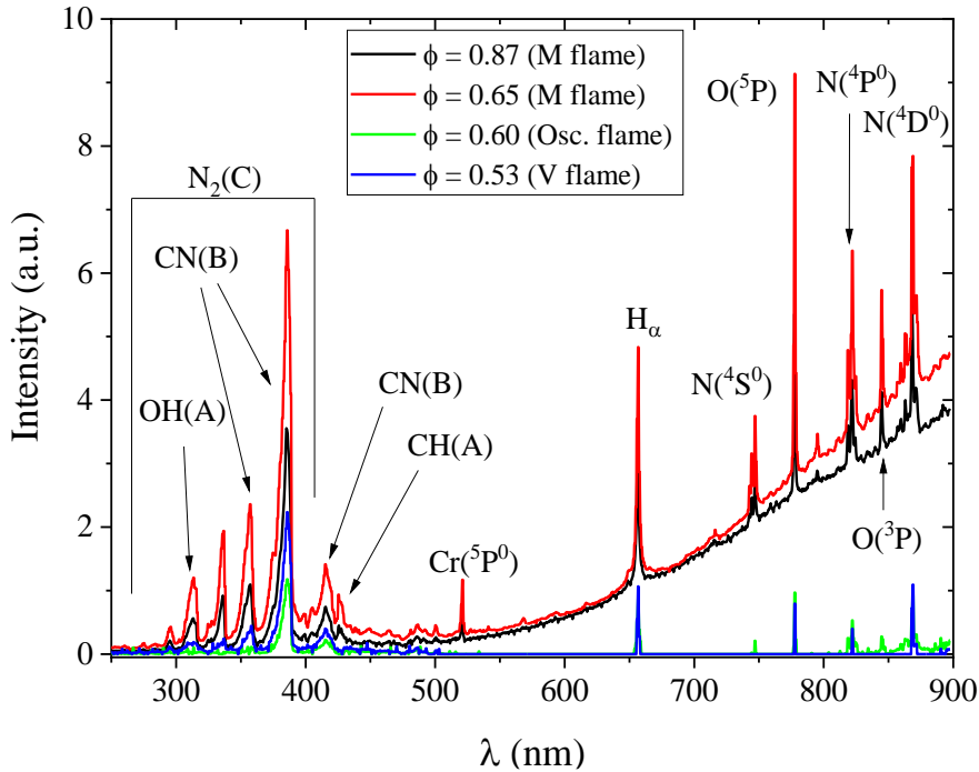
Figure 9.4 Typical emission spectra recorded in a dodecane flame assisted by NRP discharges. In the four regimes (corresponding to \phi = 0.87, 0.65, 0.60, and 0.53 ), the emissions of \text{N}_2(\text{C}) , \text{CH} , \text{CN} , \text{OH} , \text{O} , \text{H} , and \text{N} are visible.
