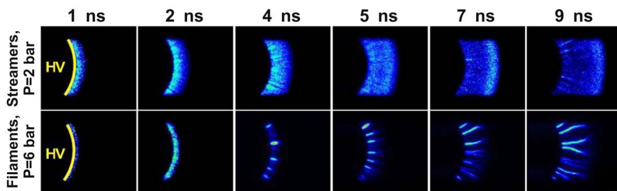
Figure 3.2 Formation of a SDBD streamer by a nanosecond discharge (top). The increase of pressure induced the formation of filaments (bottom). Reproduced with permission from (Shcherbanev et al. , 2019)
