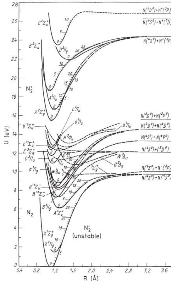
Figure 1.4 Energy diagram (Gilmore, 1965; Radzig and Smirnov, 1985, p. 370) of N 2 , N 2 + , and N 2 + including the vibrational structure of each electronic state.
