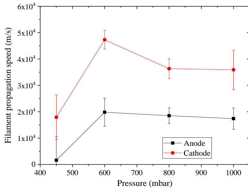
Figure 4.5 Propagation speed of the filaments from 400 mbar to 1 bar. At the anode, the speed is relatively constant \approx 20 \mu\text{m}\cdot\text{ns}^{-1} . The speed of propagation of the cathode filament is of the same order of magnitude, with a peak at 5 \times 10^4 \text{ m}\cdot\text{s}^{-1} = 50 \mu\text{m}\cdot\text{ns}^{-1} .
