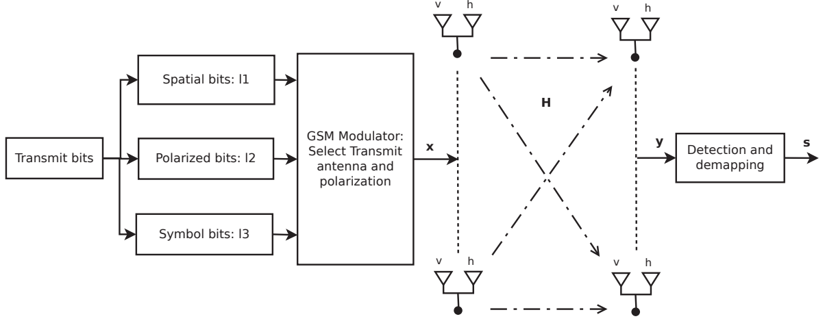
Figure 3.28 – N_r \times N_t DP-GSM system model.
