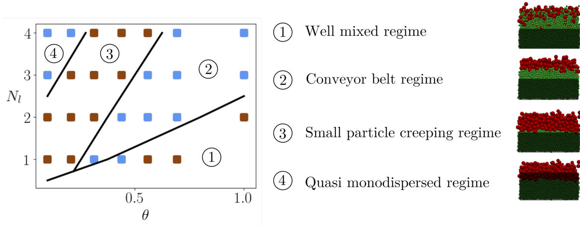
Figure 5.10: Mapping of the four different observed phenomenologies in the bidisperse transport process. Each regime is illustrated with a typical simulation picture where the creeping flow has been shaded in gray. Results are plotted in colored squares and split into two classes : blue (predicted transport error less than 10%) and brown (larger error).
