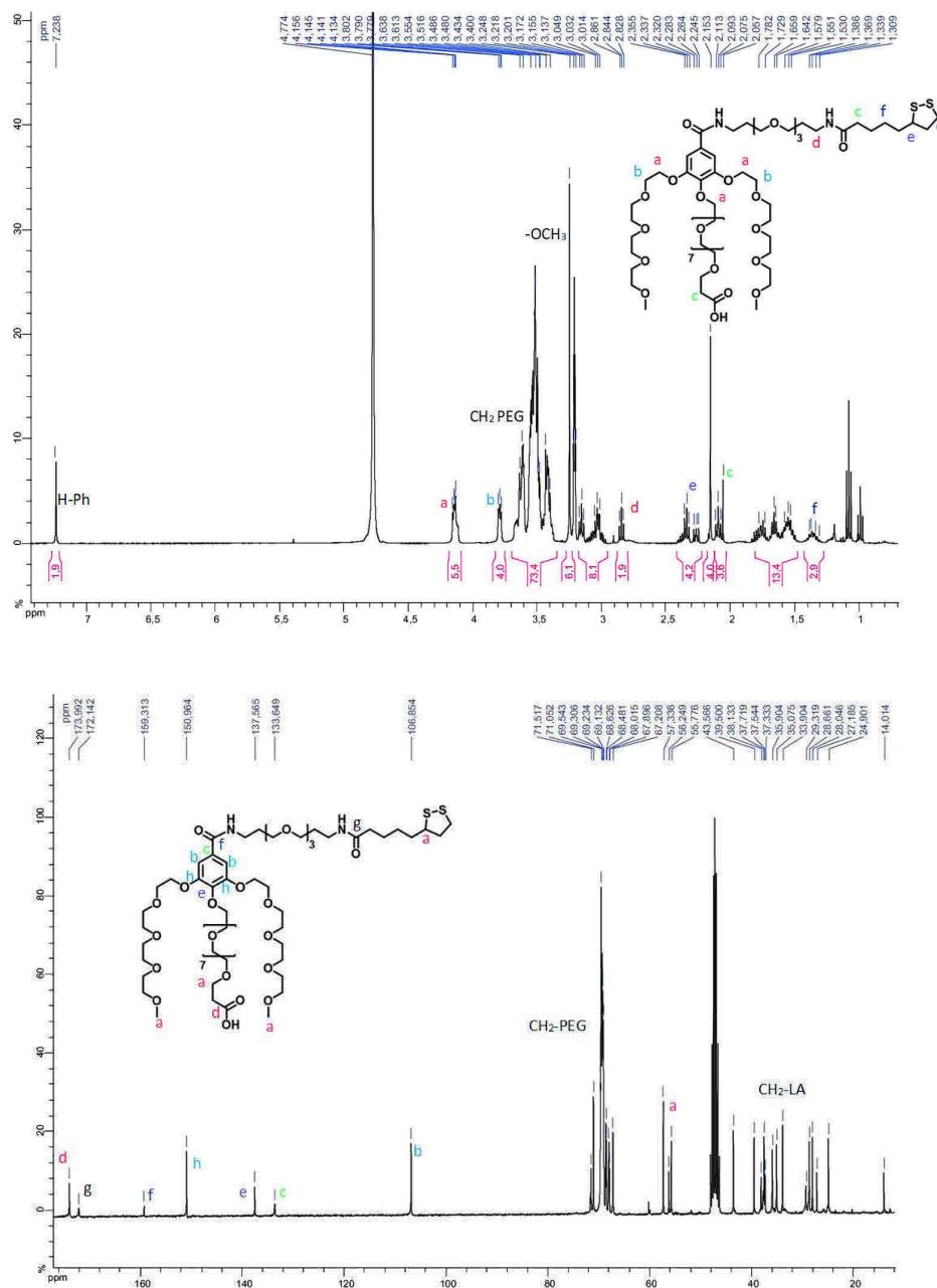
Figure 50: ^1\text{H} (top) and ^{13}\text{C} (down) NMR (MeOD, 300MHz) profiles of compound 43.
