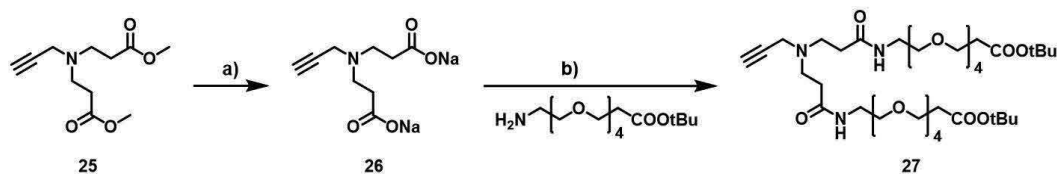
Figure 41: Introduction of functional PEG chains into a poly(amido)-amine monomer 27 : a) TMSO Na 1M, CH 2 Cl 2 , rt, 16 h, quant.; b) EDCI, HOBT, DIPEA, CH 3 CN, rt, 16 h, 67%.
