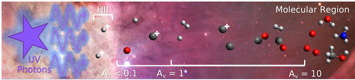
Figure 1.2: Schematic of a typical photodissociation region. The PDR is illuminated by UV photons from the left and extends from where atomic matter dominates to where the photodissociation of O_2 is negligible, at A_V \approx 10 . This is where, what we consider, the molecular region starts. Credit for the original image of the Orion Nebula to Hubble/ESA/NASA.
