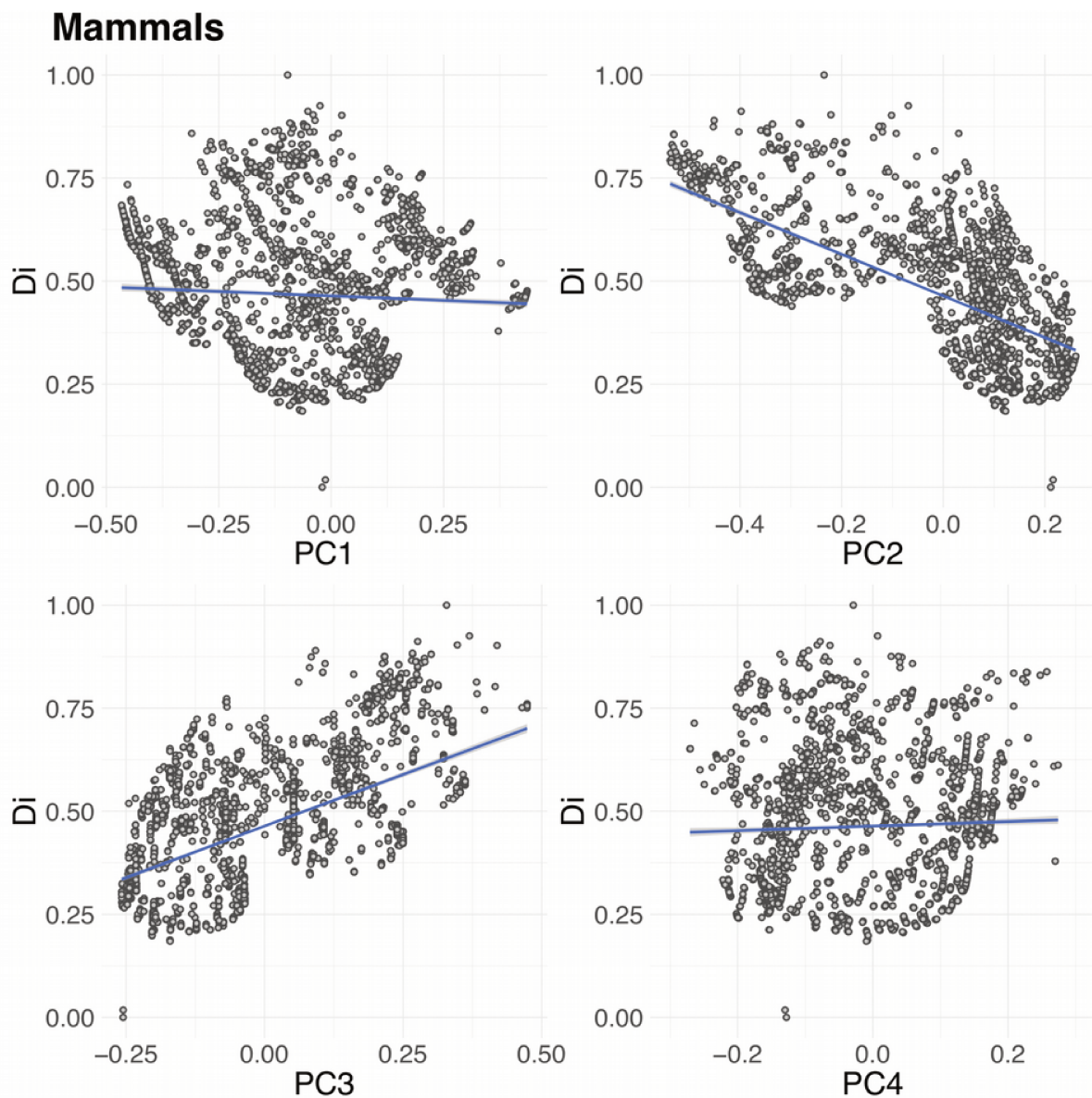
Supplementary Figure 2: Relation between functional distinctiveness ( D_i ) and the four axes of the functional traits PcoA for mammals. Blue line represents the linear model between D_i and PcoA axes. Distinctiveness was mainly correlated with axes 2 and 3 of the PcoA ( R^2 = 0.51 , R^2 = 0.31 , p -values < 0.001 ).
