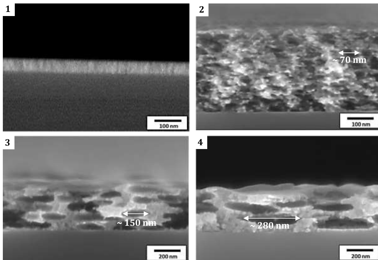
Figure IV-11: SEM images showing the pores shapes on section of the \text{TiO}_2 layers obtained after the molding with sol-gel and the annealing process at high temperature 1) no PMMA 2) P50+ 3) P100+ 4) P200+
