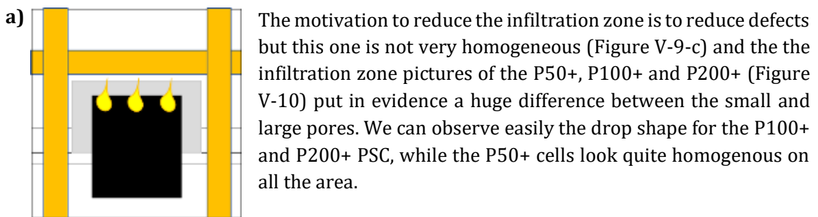
Figure V-9: a) Drop-casting illustration on the P100+ PSC with less delimiting zone b) Picture of the PSC from the top view and c) view from the glass side
