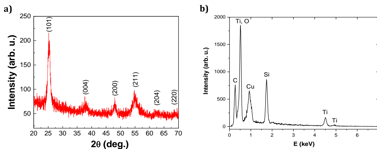
Figure IV-13: a) XRD diffractogram showing the presence of the \text{TiO}_2 anatase phase in the scaffold layer obtained after annealing at 500 °C (JCPDS 00-021-1272) b) EDX spectrum recorded on the \text{TiO}_2 porous layer
