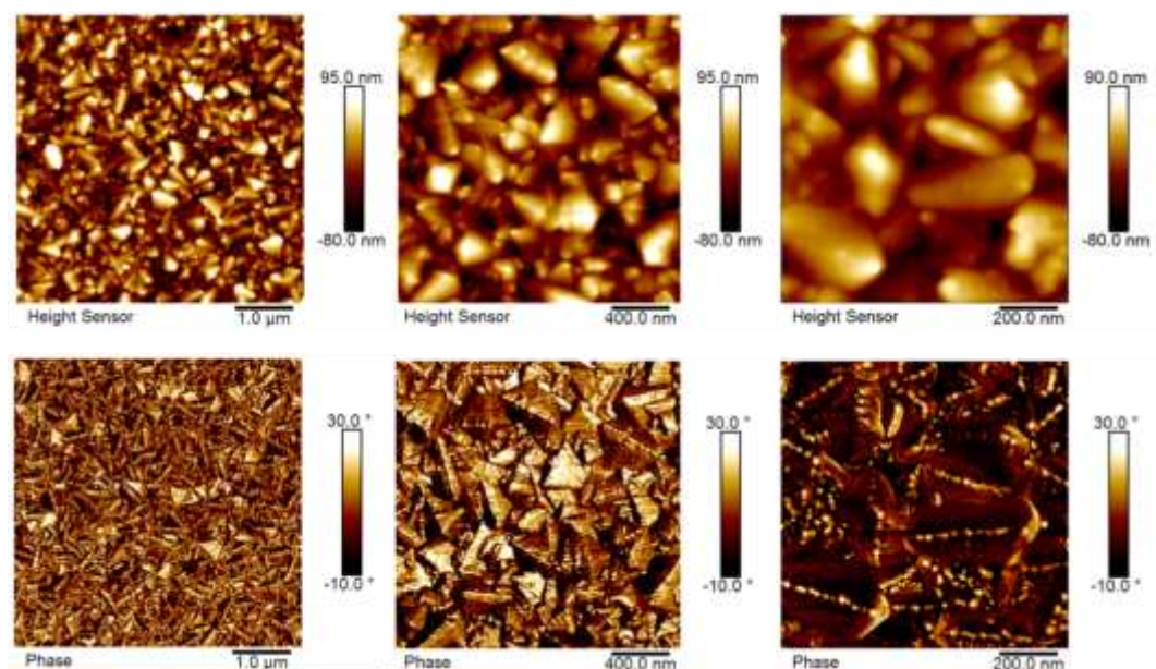
Figure III-10: AFM topography (top images) and phase images (bottom images) of c\text{-TiO}_2 deposited by SPD on FTO substrate at different scale barre
