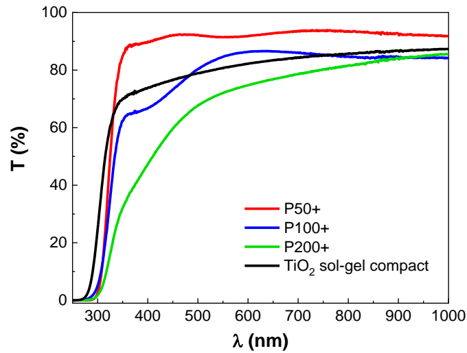
Figure IV-14: Transmittance graph of the different \text{TiO}_2 porous layers
