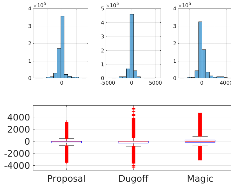
Figure 6.13 – Mission No. 2 Lateral TGFs comparison. Analysis made using our proposal, the Dugoff’s model and magic tire model. Up: Distribution of the estimation error. Down: Boxplot graph obtained from the estimation error for the TGFs.
