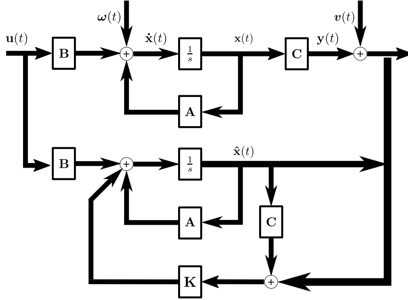
Figure 3.3 – Kalman Filter
