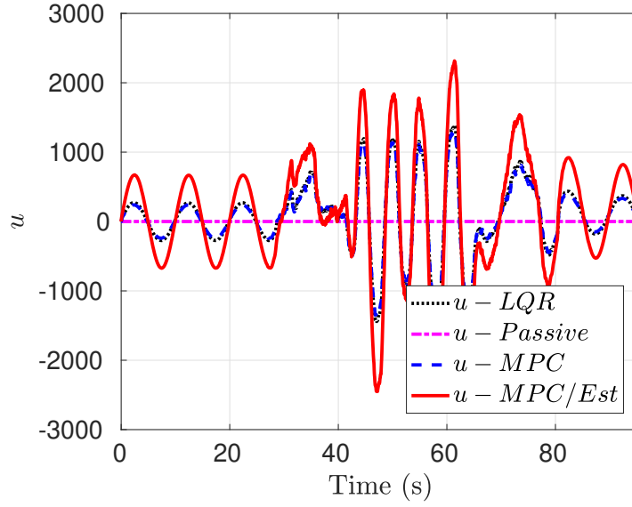
Figure 7.9 – Control input comparison between the four closed loop systems
