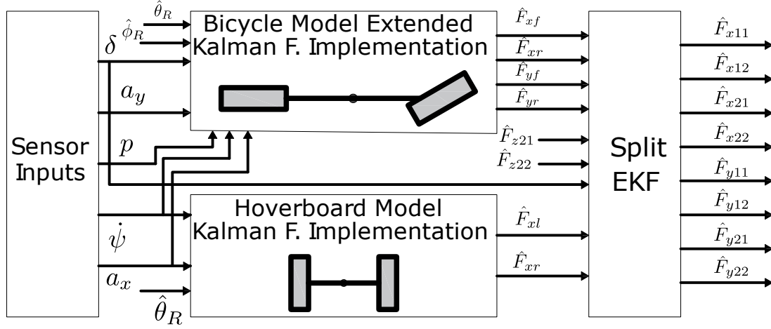
Figure 5.1 – Longitudinal/Lateral TGFS estimation scheme
