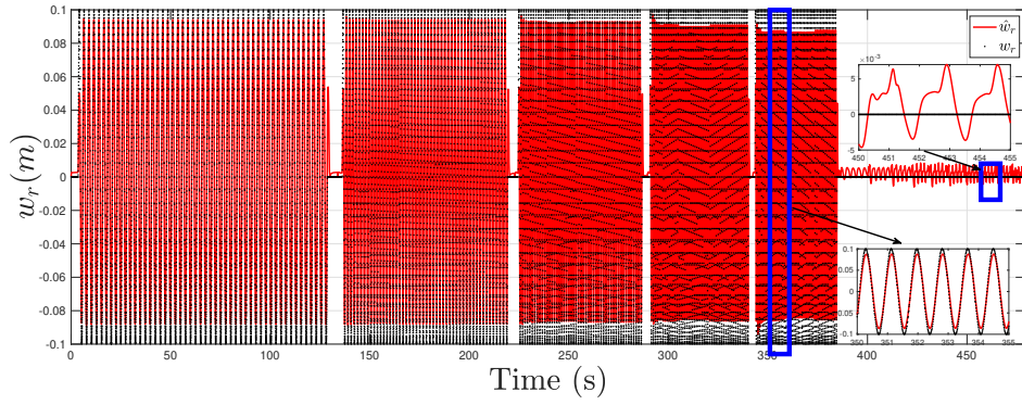
Figure 7.4 – Road profile estimation, \hat{z}_{rij} against the actual road profile, z_{rij} . The first 134 seconds the vehicle speed is 10 km/h, from 134 to 222 seconds the velocity is 15 km/h, from 222 to 289 s. v = 20 km/h, from 289 to 342 s. the vehicle speed is 25 km/h, from 340 to 386 s. the velocity is 30 km/h. Until second 386 the road is described by z_r = 0.1 \cdot \sin\left(\frac{1}{7} \cdot 2 \cdot \pi \cdot x_{pos}\right) where x_{pos} . From 386 to 480 seconds, the road profile is zero and the vehicle is performing the slalom maneuvers at different speeds from 50 to 100 km/h.
