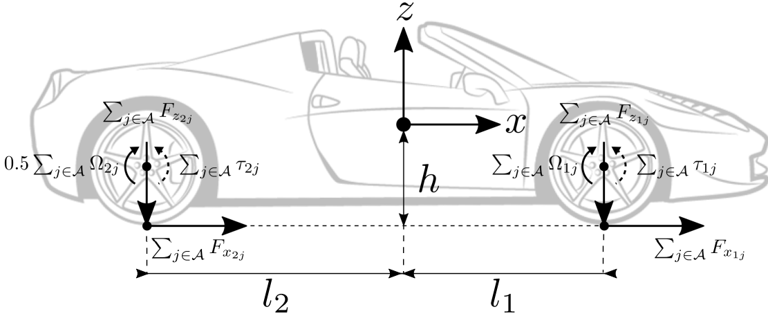
Figure 2.13 – Double-corner model
