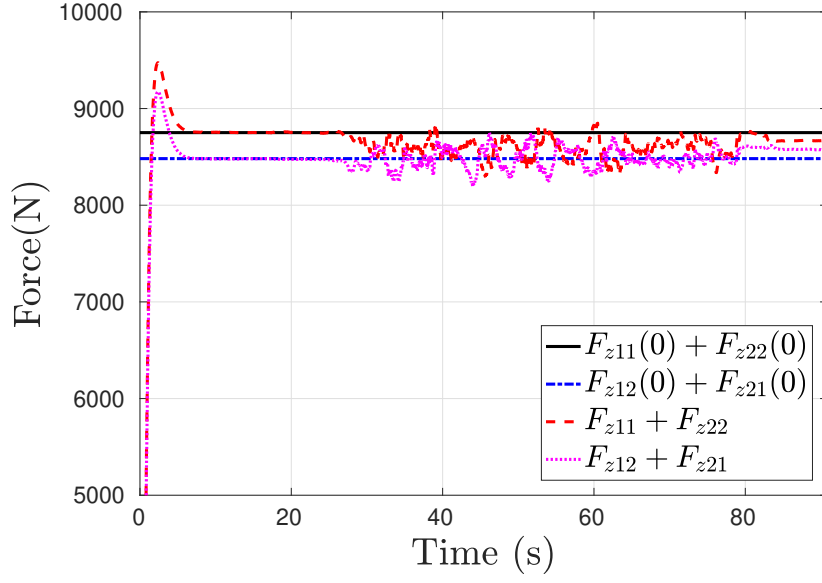
Figure 4.2 – Comparison between real and estimation of vertical forces addition ( \hat{F}_{z11} + \hat{F}_{z22} ; \hat{F}_{z12} + \hat{F}_{z21} ) developed in equation (4.19), experimental measures are provided by dynamometric wheels installed on the experimental vehicle.
