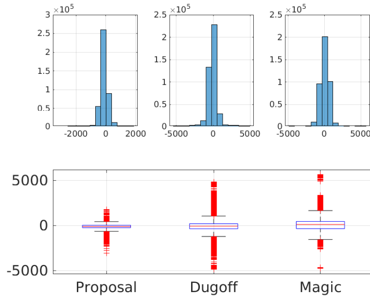
Figure 6.14 – Mission No. 3 Lateral TGFs comparison. Analysis made using our proposal, the Dugoff’s model and magic tire model. Up: Distribution of the estimation error. Down: Boxplot graph obtained from the estimation error for the TGFs.
