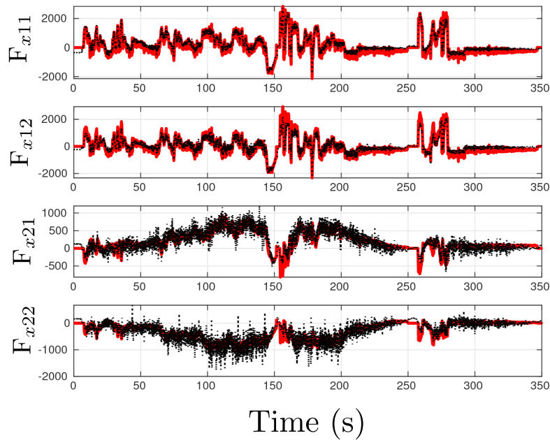
Figure 5.10 – Estimated Longitudinal TGFs, \hat{F}_{xij} , response compared against the actual measurement given by Kysler dynamometers during test No. 3. Red-Solid line: \hat{F}_{xij} - Proposal. Black-Pointed line: F_{xij} - Sensor Measurement
