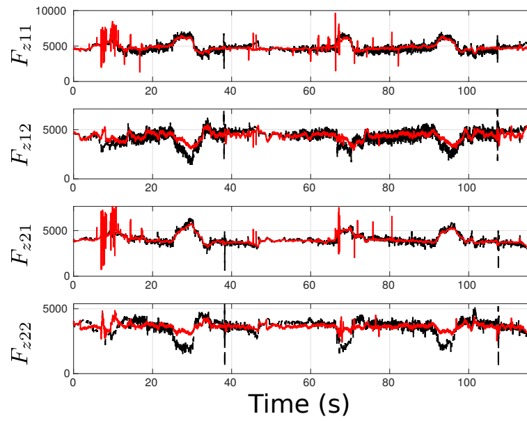
Figure 4.17 – Low Friction Mission. Normal TGFs comparison. Model Fusion Proposal: red-solid line. Sensor measurement: black-dashed line.
