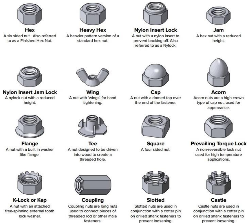
Figure 27: Different type of nuts 17
