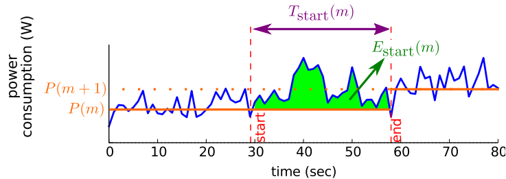
Figure II.8 – Power consumption when starting a VM.
