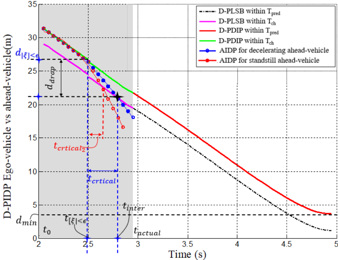
Figure 6.6: Definition of a_{req} based on the D-PIDP
