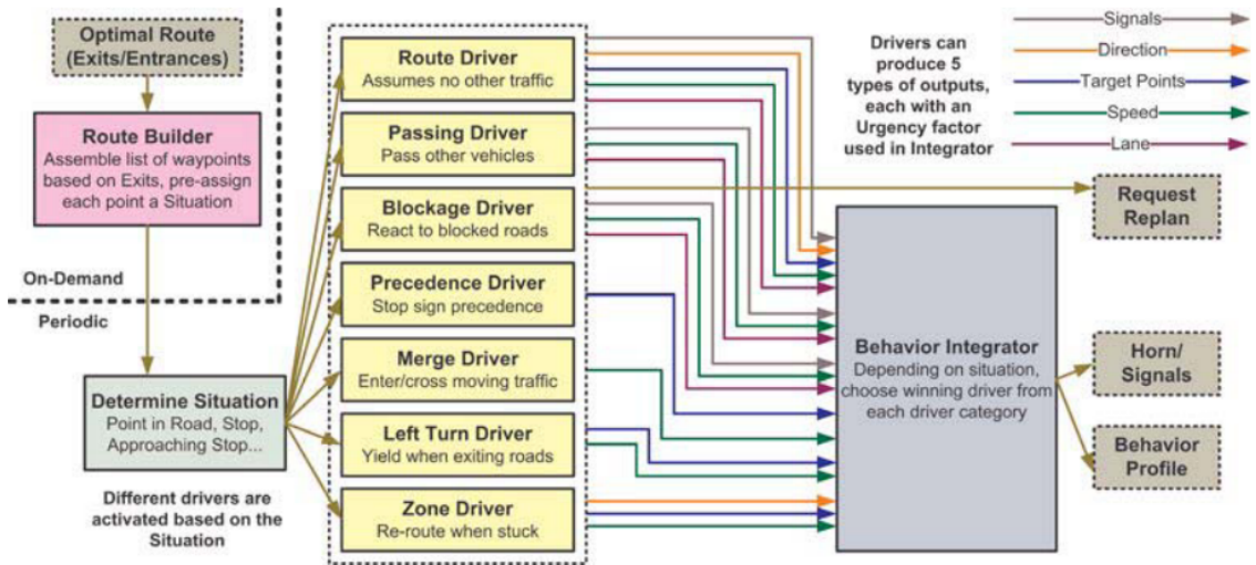
Figure 2.7: Flow diagram of the Behavior-Based architecture and the Action-Selection Mechanism (Image credit: [45])
