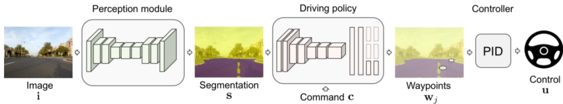
Figure 2.11: System architecture composed of a perception module implemented by an encoder-decoder network, a command driving policy implemented by a branched convolutional network and a low-level PID controller (Image credit [158]).
