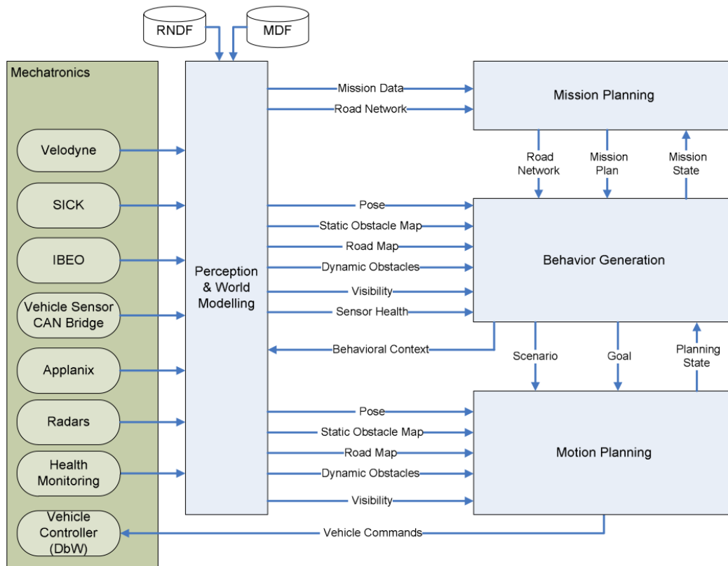
Figure 2.5: Boss's Overall Architecture (Image credit: [210]). Composed into: Mission Planning, Motion Planning, Behavior Generation, Perception and World Modeling, and Mechatronics. The RNDF and the MDF are respectively the Road Network Definition File and the Mission Data File
