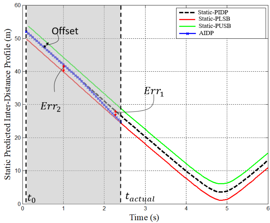
Figure 5.16: The lateral error definition of the S-PIDP between ego-vehicle and surrounding obstacle-vehicle
