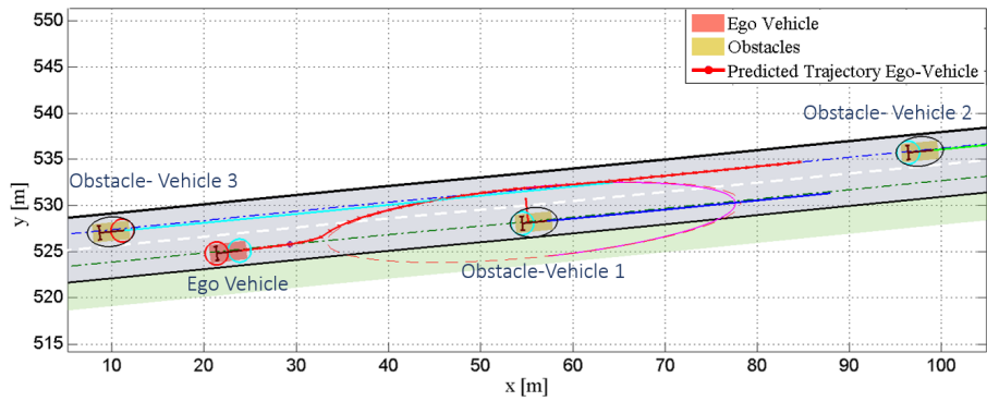
Figure 5.21: Car Simulator: Predicted Trajectories
