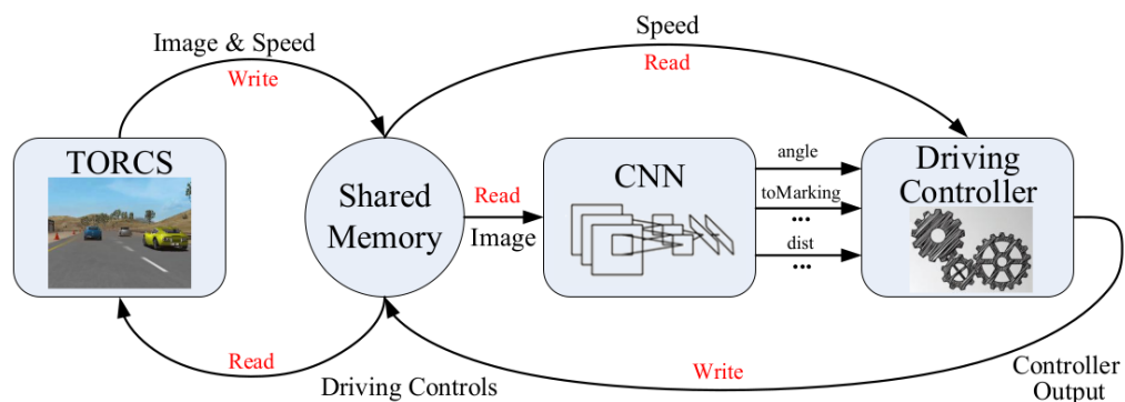
Figure 2.10: System architecture of a direct perception approach by Chen et al., (Image credit [52]).
