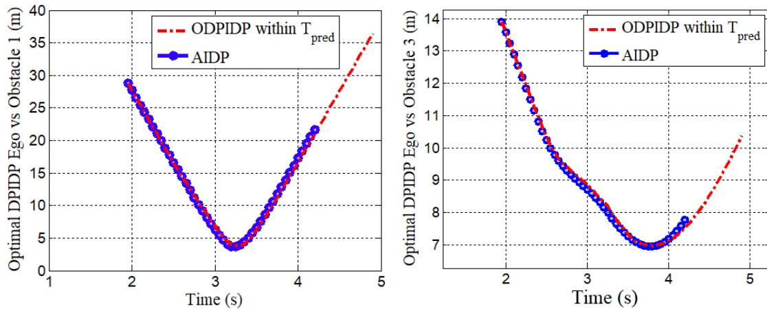
(a) Optimal D-PIDP: Ego vs. Obstacle-Vehicle 1 (b) Optimal D-PIDP: Ego vs. Obstacle-Vehicle 3
