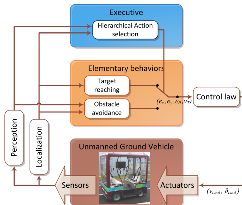
Figure 5.1: Vilca's Control Architecture [Image credit: [219, Chapter 3]]
