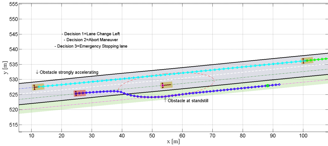
Figure 6.16: Evasive trajectory involving swerving to the shoulder lane for Scenario 2
