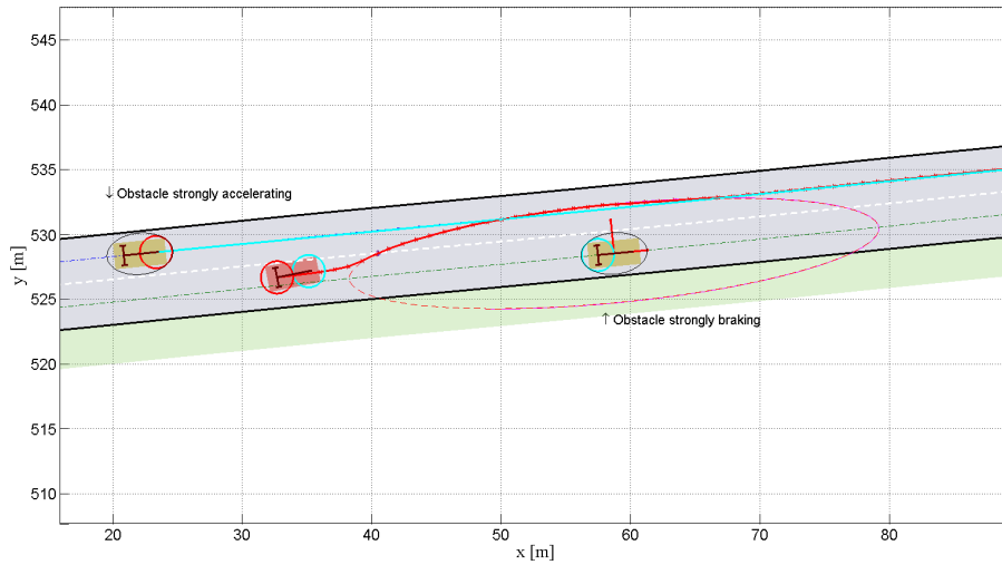
Figure 5.23: Example of a navigation in emergency situations (cf. Simulation Video - https://shorturl.at/qstLX )
