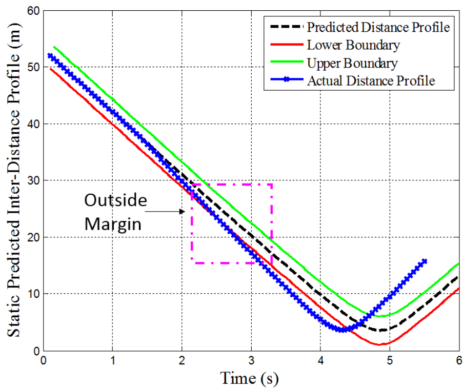
Figure 5.17: S-PIDP during a change in the dynamic of progression of the ahead-vehicle
