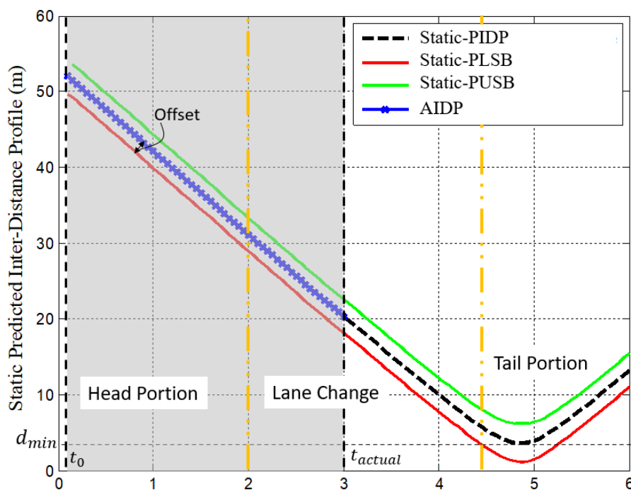
Figure 5.15: Static Predicted Inter-distance Profile (S-PIDP)
