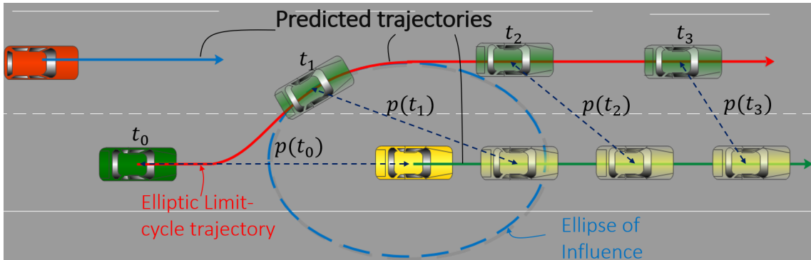
Figure 5.14: Predicted Trajectories during lane change maneuver
