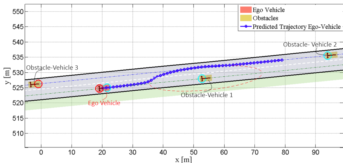
Figure 6.9: Setup of the simulation environment
