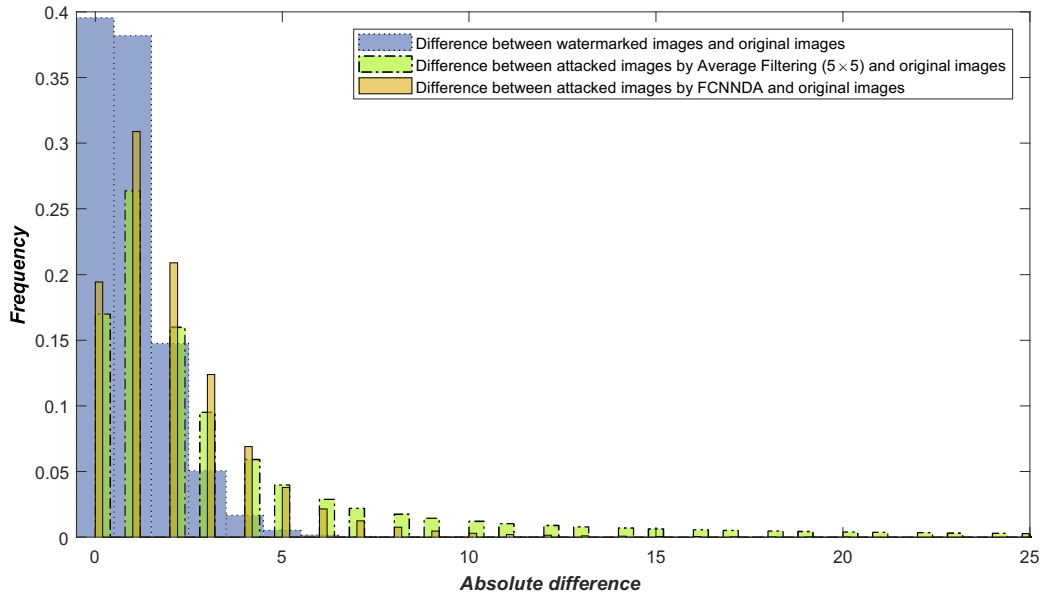
Figure 6.13: Comparing the pixels values of the original images to the watermarked images, and the attacked images by FCNDA and Average filtering ( 5 \times 5 ), when random bits are embedded per image, and STDM with DCT is used as watermarking scheme
