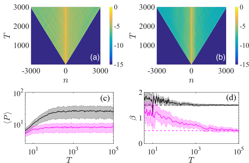
Fig. 5.4. Spatiotemporal evolution of the energy density for a representative realization with (a) momentum and (b) displacement single site initial excitation. The colorbars in (a) and (b) are in log-scale. (c) Mean time evolution of \langle P \rangle , (d) estimation of the exponent \beta , related to the time evolution of the average second moment through \langle m_2 \rangle \propto T^\beta . The mean values \langle \cdot \rangle are calculated from 100 disorder realizations and the shaded areas represent the statistical error. The dashed lines in (d) indicates \beta = 1.5 (top) and \beta = 0.5 (bottom) and the system energy for all realizations was H = 10^{-4} .
