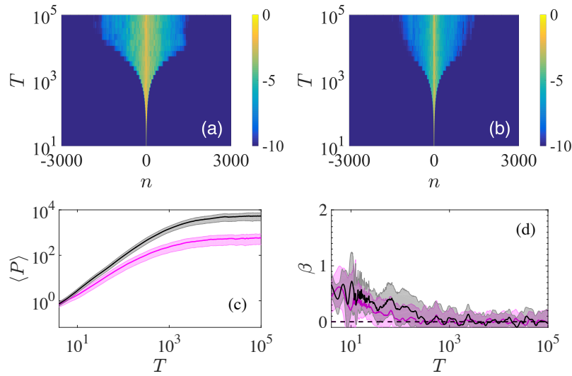
Fig. 5.5. Similar to Fig. 5.4 but for rotational excitations.
