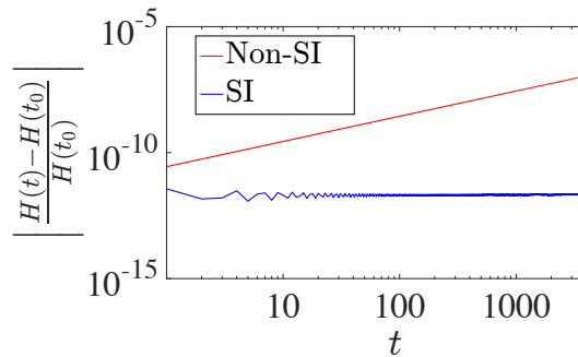
Fig. 2.1. Symplectic integration vs non-symplectic integration of the mass spring system to compare energy conservation for the two methods. For both schemes, the total system energy was H = 0.5 and a time step of \tau = 0.01 was employed.
