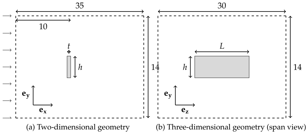
FIGURE 7.1: Two-dimensional and three-dimensional flow configurations. Sketch of the computational domains used for (a) the two-dimensional plate of height h = 1 and thickness t = 1/6 and (b) the three-dimensional plate of span L = 2.5 immersed in an upstream uniform streamwise flow U_\infty .
