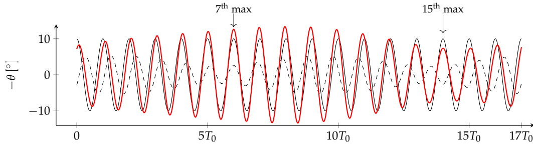
FIGURE 6.12: Reconstruction of the full perturbed pitching solution \theta_0(t) + \epsilon\theta'(t) (red line). For comparison, the LCO component \theta_0(t) is shown with thin black solid line, whereas the perturbation component \epsilon\theta'(t) is shown with thin black dashed line. The perturbation amplitude \epsilon is arbitrary, for easy visualization.
