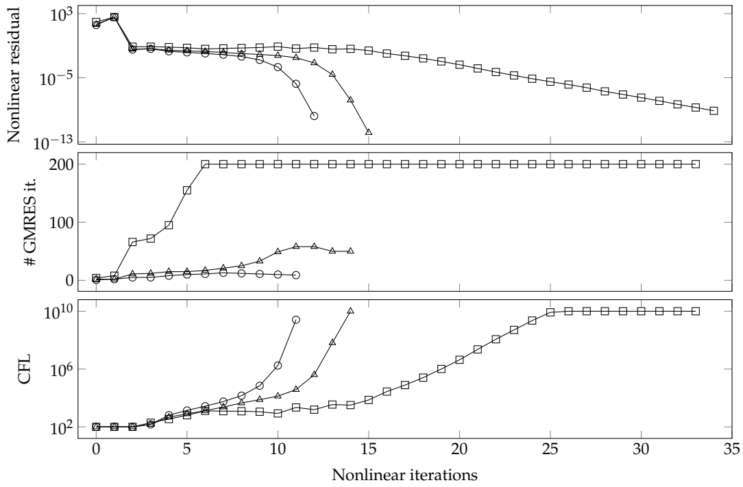
FIGURE 3.6: Performance of the Newton–Krylov approach different reduced frequencies: \omega = 0.4 (circles), \omega = 1 (triangles), \omega = 3.6 (squares). The number of harmonics is N = 20 .
