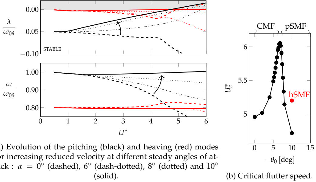
FIGURE 4.7: Transition from coupled-mode flutter (CMF) to pitching single-mode flutter (pSMF) as the steady angle of attack increases. When the steady solution is stalled ( -\theta_0 > 9^\circ ), a single-mode flutter on the heaving mode (hSMF) is also triggered. ( Re = 500, \tilde{m} = 10^3 )
