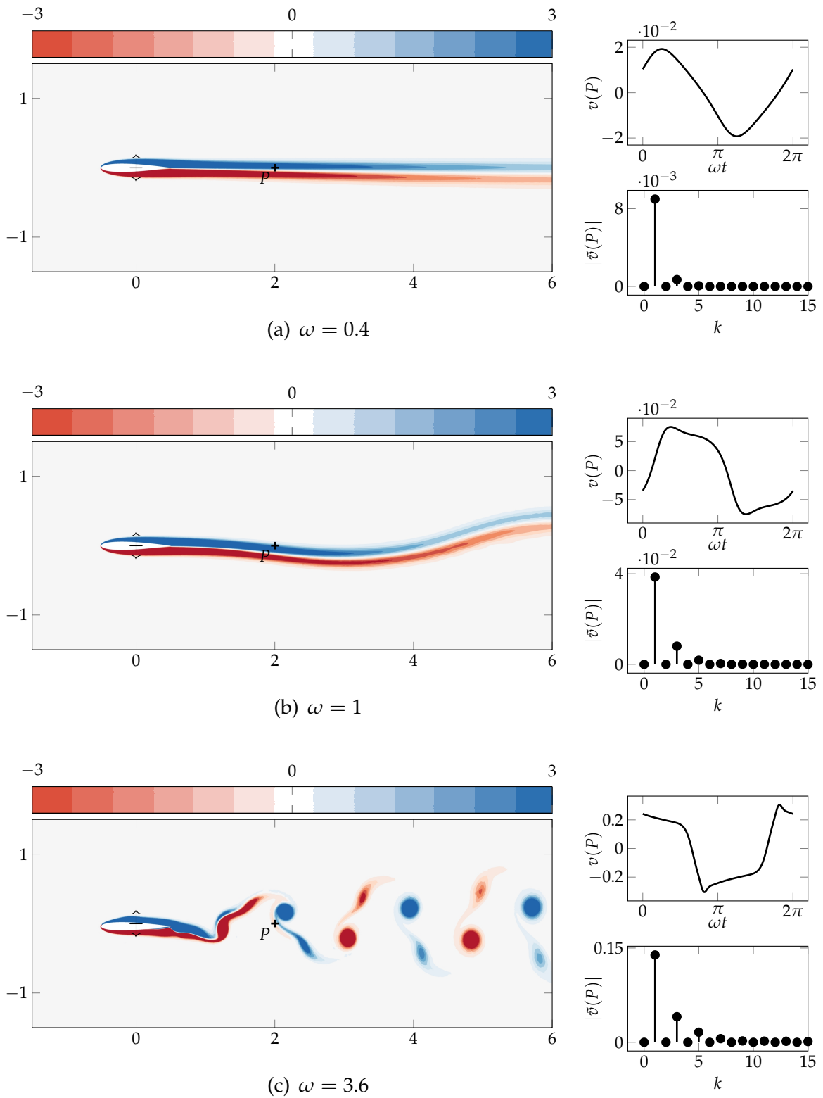
FIGURE 3.2: NACA0012 airfoil forced in plunging motion at different frequencies \omega . Vorticity snapshots are shown on the left whereas the time signal of vertical velocity at point P is shown on the right (top: temporal series, bottom: Fourier spectrum).
