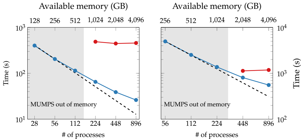
(a) Nonlinear solver (average time per New- (b) Eigensolver (overall time for 5 eigenval- ton iteration) ues, s = 0.6i )
