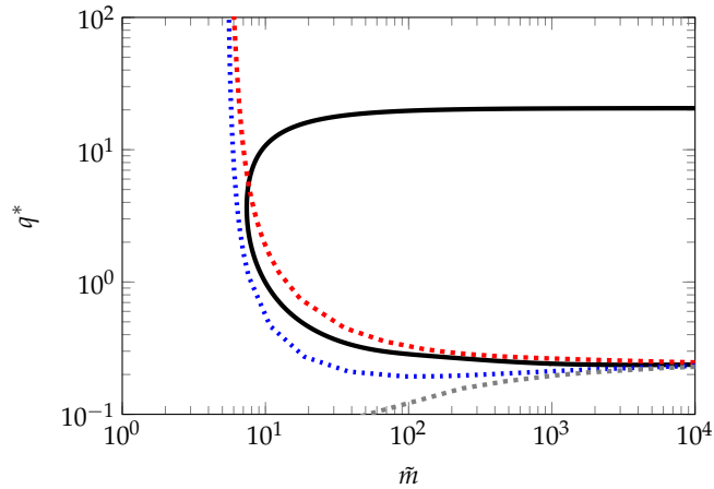
FIGURE 4.15: Comparison of the neutral curves in the (\tilde{m}, q^*) plane at Re = 2900 given by the Navier–Stokes (solid line), Theodorsen (dotted red) and quasi-steady (QSM1 in dotted gray and QSM2 in dotted blue) flow models.
