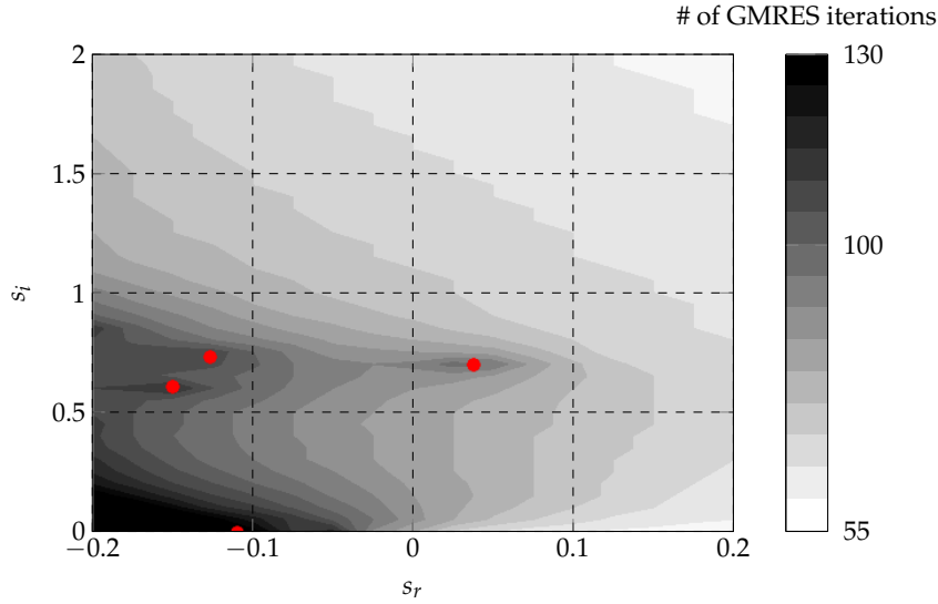
FIGURE 7.4: Influence of the complex shift. Isocontours represent the number of GMRES iterations needed to solve the linear system (7.13) with the mAL preconditioner, depicted in the complex plane (s_r, s_i) , and computed for Re = 40 and \gamma = 0.7 . The red circles are the eigenvalues of the Jacobian matrix (7.6).
