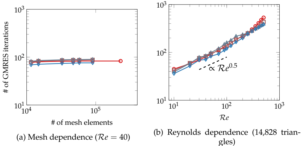
FIGURE 7.5: Effect of mesh refinement (a) and Reynolds number (b) on mAL preconditioning efficiency. The GMRES iteration count for solving eq. (7.12) to a relative tolerance of 10^{-6} is presented for different shifts: s = 0 ( \circ ), s = 0.3i ( \square ), s = 0.6i ( \triangle ) and s = 1i ( \diamond )
