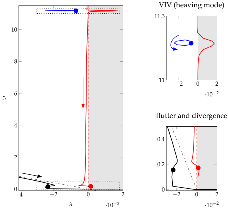
FIGURE 4.3: Loci of the three leading eigenvalues represented by disks in fig. 4.1b, as the reduced velocity varies ( U^* \in [0.05, 8] ). The dashed straight lines indicate the loci of the uncoupled (solid-only) solid modes (heaving in red, pitching in black). The arrows indicate the direction of increasing U^* . The dotted rectangles materialize the zones of VIV type and flutter/-divergence type instabilities, of which zoomed views are exposed in the right part of the figure. The filled gray area represents the unstable half plane.
