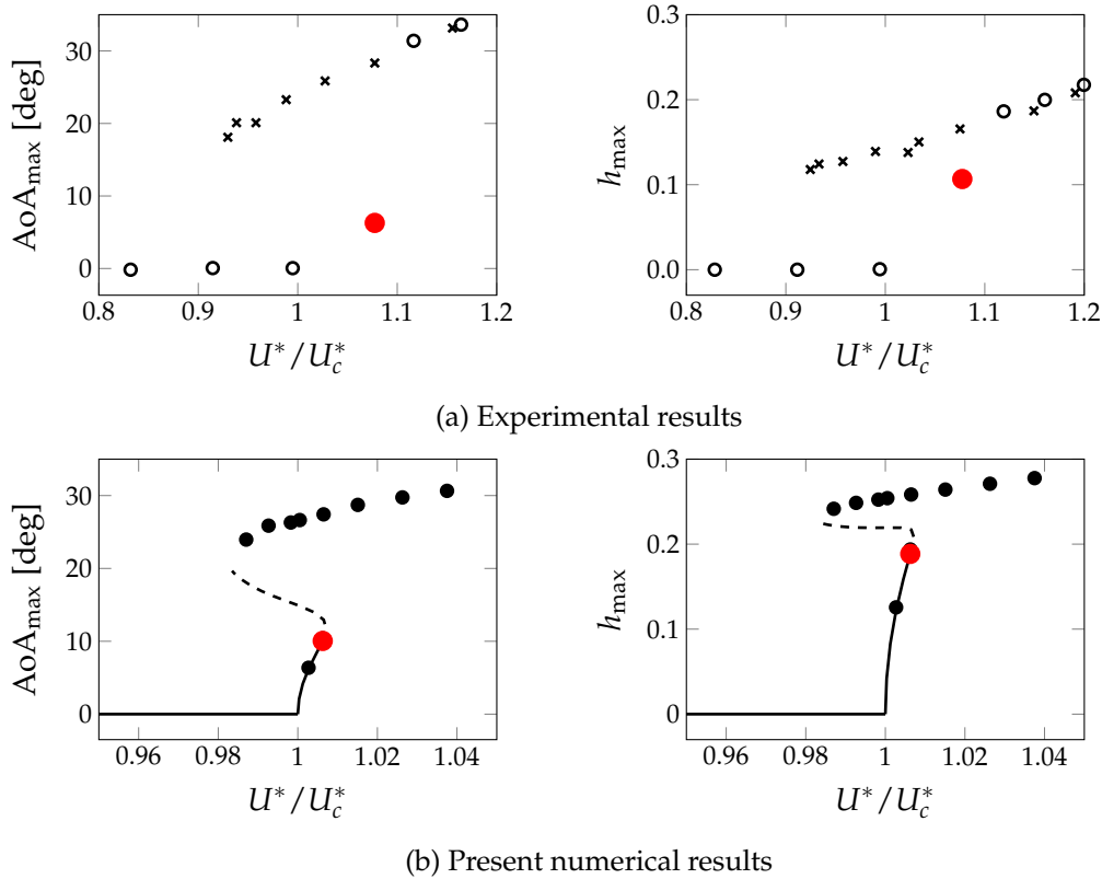
FIGURE 5.19: Qualitative comparison of the supercritical double-fold scenario exposed in fig. 5.18 with wind-tunnel data from [Amandolese et al. 2013]. Pitching (left) and heaving (right) amplitude results are given for (a) the experimental results ( \tilde{m} = 2100 , \mathcal{Re} \simeq 30000 ) and (b) the present numerical results ( \tilde{m} = 120 , \mathcal{Re} = 500 ). For the description of (a), see fig. 5.18. In (b), circles (resp. crosses) mark increasing (resp. decreasing) wind velocity.
