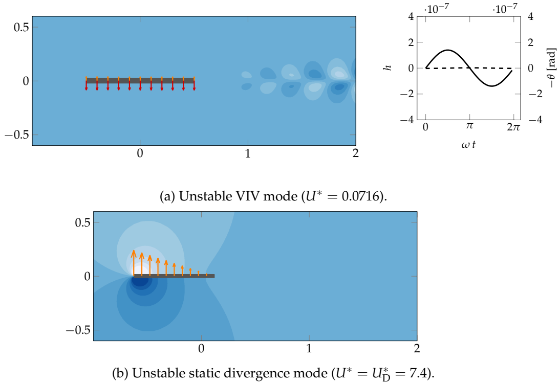
FIGURE 4.4: Eigenmodes corresponding to the (heaving) VIV and divergence instabilities observed in fig. 4.3. The orange (resp. red) arrows represent the displacement (resp. velocity) vectors whereas the pressure field is visualized by the blue colormap.
