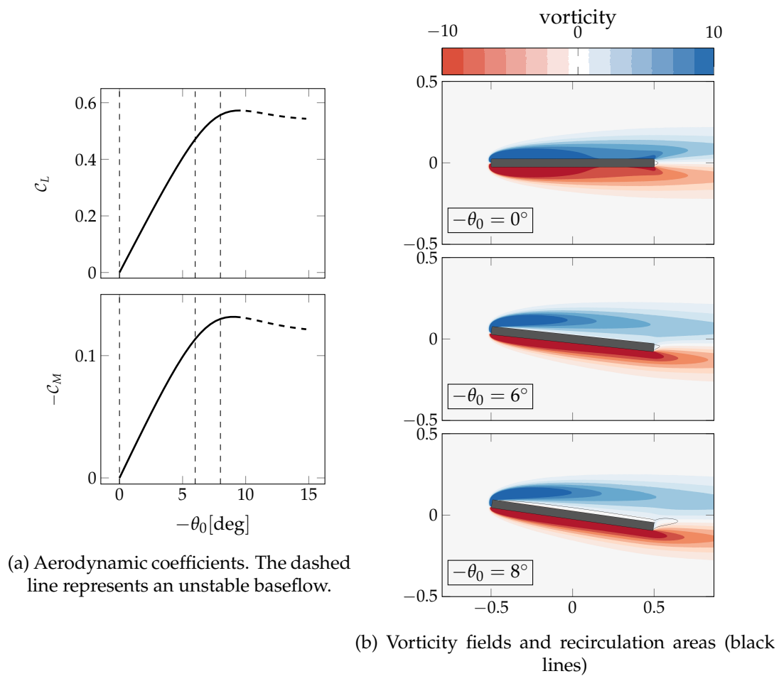
FIGURE 4.6: Features of the steady flow around the fixed plate at different angles of attack ( Re = 500 ).
