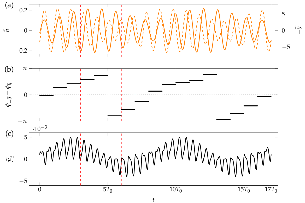
FIGURE 6.9: Time representation of the oscillating part, \tilde{\mathbf{q}} = \mathbf{q}^\circ(t)e^{i\omega t} + \text{c.c.} , of the perturbation generated by the pair of unstable Floquet modes at U^*/U_c^* = 1.10 . (a) Heaving (solid line) and pitching (dashed line) signals. (b) Average phase shift between pitching and heaving over each fast period T_0 . (c) Power transmitted by the fluid to the solid. In all figures, the vertical dashed lines materialize the periods of maximal fluid energy extraction by the solid and maximal solid energy dissipation by the fluid.
