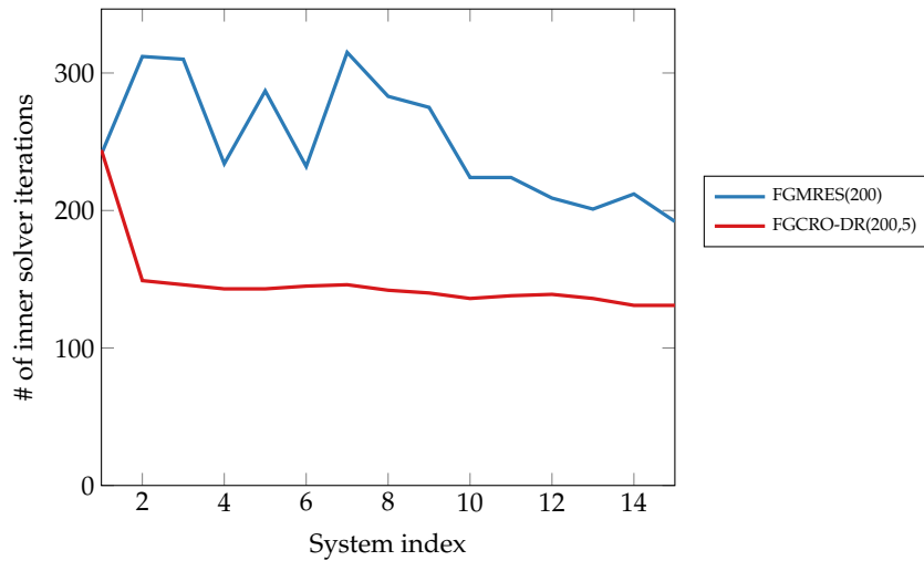
FIGURE 7.10: Effect of a recycled Krylov method on the performance of the eigensolver. The number of mAL-preconditioned inner iterations for the flexible GMRES and GCRO-DR algorithms is compared for each linear solve of a Krylov–Schur iteration.
