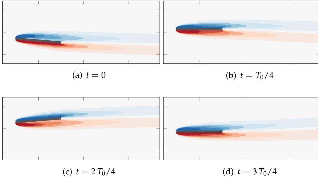
FIGURE 5.13: Supercritical bifurcation. Snapshots of vorticity for the low-amplitude LCO at \tilde{m} = 1000 and U^*/U_c^* = 1.016 .
