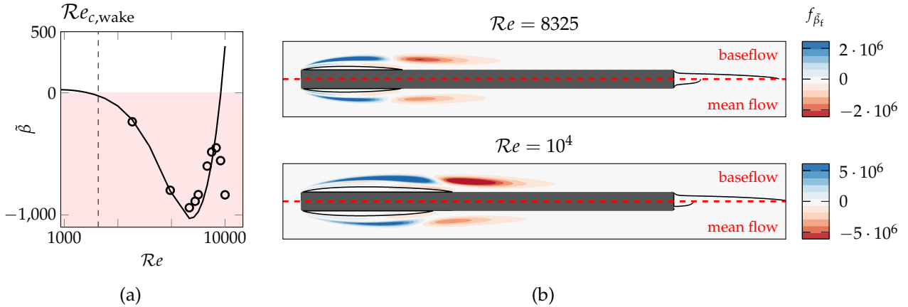
FIGURE 5.11: Weakly nonlinear flutter analysis performed around the base or mean flows for \tilde{m} = 10^4 . (a) Nonlinear coefficient \tilde{\beta} as a function of the Reynolds number obtained with the base (solid line) and mean (circles) flow analyses. Negative and positive values correspond to subcritical and supercritical bifurcation, respectively. (b) Spatial distribution of the nonlinear fluid contribution \tilde{f}_{\tilde{\beta}_i} (cf eq. (5.14)) is presented for both the base and mean flow analyses at Re = 8325 and Re = 10^4 . The integral of that contribution gives the dominant contribution to \tilde{\beta} .
