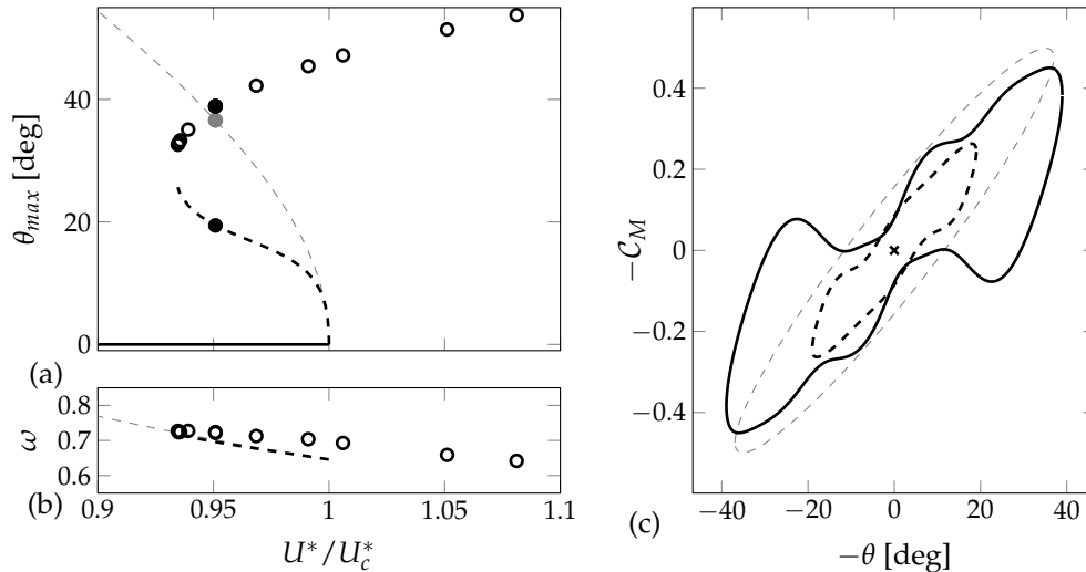
FIGURE 5.14: Subcritical bifurcation for \tilde{m} = 60 and \mathcal{R}e = 500 . Same legend as in fig. 5.12. The critical reduced velocity is U_c^* = 1.33 . The dashed curves corresponds to unstable LCO. The LCO displayed in (c) corresponds to U^* = 0.95U_c^* .
