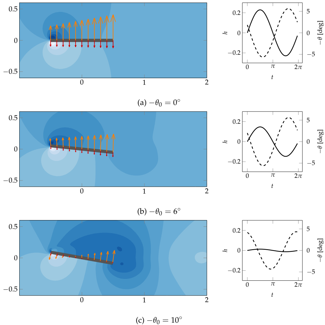
FIGURE 4.8: Visualisation of the critical flutter eigenmodes at three different angles of attack. For each subfigure, the left part represents a snapshots of the mode at t=3\pi/4 , where the blue colormap represents the pressure field, while the arrows materialise the solid displacement (orange) and velocity (red) vectors. On the right part, we show the time signals for the vertical displacement (solid line) and pitching angle (dashed line).
