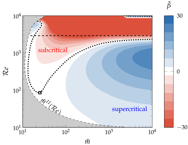
FIGURE 5.5: Effect of mass ratio and Reynolds number on the type of the flutter bifurcation. The colormap represents the criticality indicator \tilde{\beta} in the (\tilde{m}, Re) plane, whereas the dotted line indicates the contour \tilde{\beta} = 0 which separates subcritical and supercritical cases. The gray area on the left represents mass ratios \tilde{m} < \tilde{m}^{II}(Re) , for which a divergence is the primary instability (see fig. 4.9). The upper horizontal dashed line materializes the critical Reynolds Re_{c,wake} above which the wake of the fixed plate becomes unstable.
