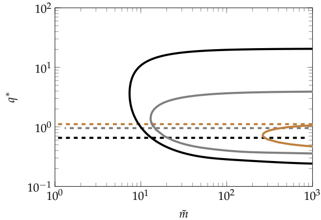
FIGURE 4.12: Linear stability neutral curves for flutter (solid lines) and divergence (dashed lines) instabilities in the plane (\tilde{m}, q^*) for different Reynolds numbers: Re = 10 (brown), Re = 110 (gray), Re = 2900 (black). For a clear identification of the stable/unstable regions, the reader is reported to fig. 4.10.
