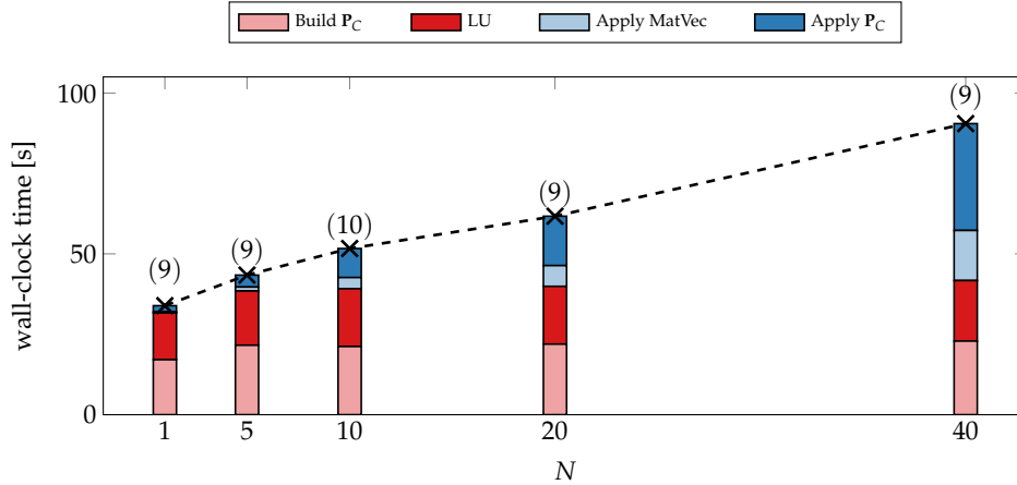
FIGURE 3.5: Wall-clock time spent in the solution of the linear system at the last Newton iteration, for different N . The forcing frequency is \omega = 0.1 . The total time (cross symbols) is split into two phases: preconditioner set-up (red) and GMRES routine (blue). The preconditioner set-up is further split into the building of the preconditioner (light red) and the LU factorization of its diagonal blocks (dark red). The GMRES phase is split into the time spent applying the matrix vector product (light blue) and applying the preconditioner (dark blue). Finally, the GMRES iteration counts are recalled between parenthesis.
