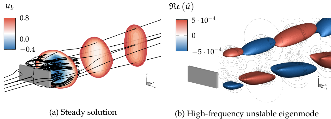
FIGURE 7.3: Linear stability analysis for the three-dimensional flow around of plate of spanwise length L = 2.5 and Re = 100 . Streamwise velocity contours of (a) the steady solution and (b) the high-frequency unstable eigenmode ( \omega = 0.57 ) are presented.
