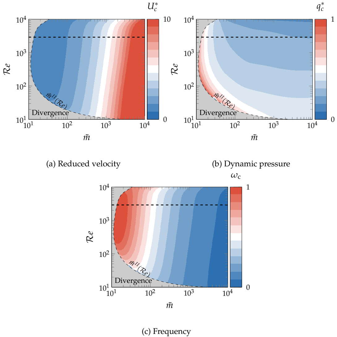
FIGURE 4.13: Influence of mass ratio and Reynolds number on different critical quantities for flutter instability.
