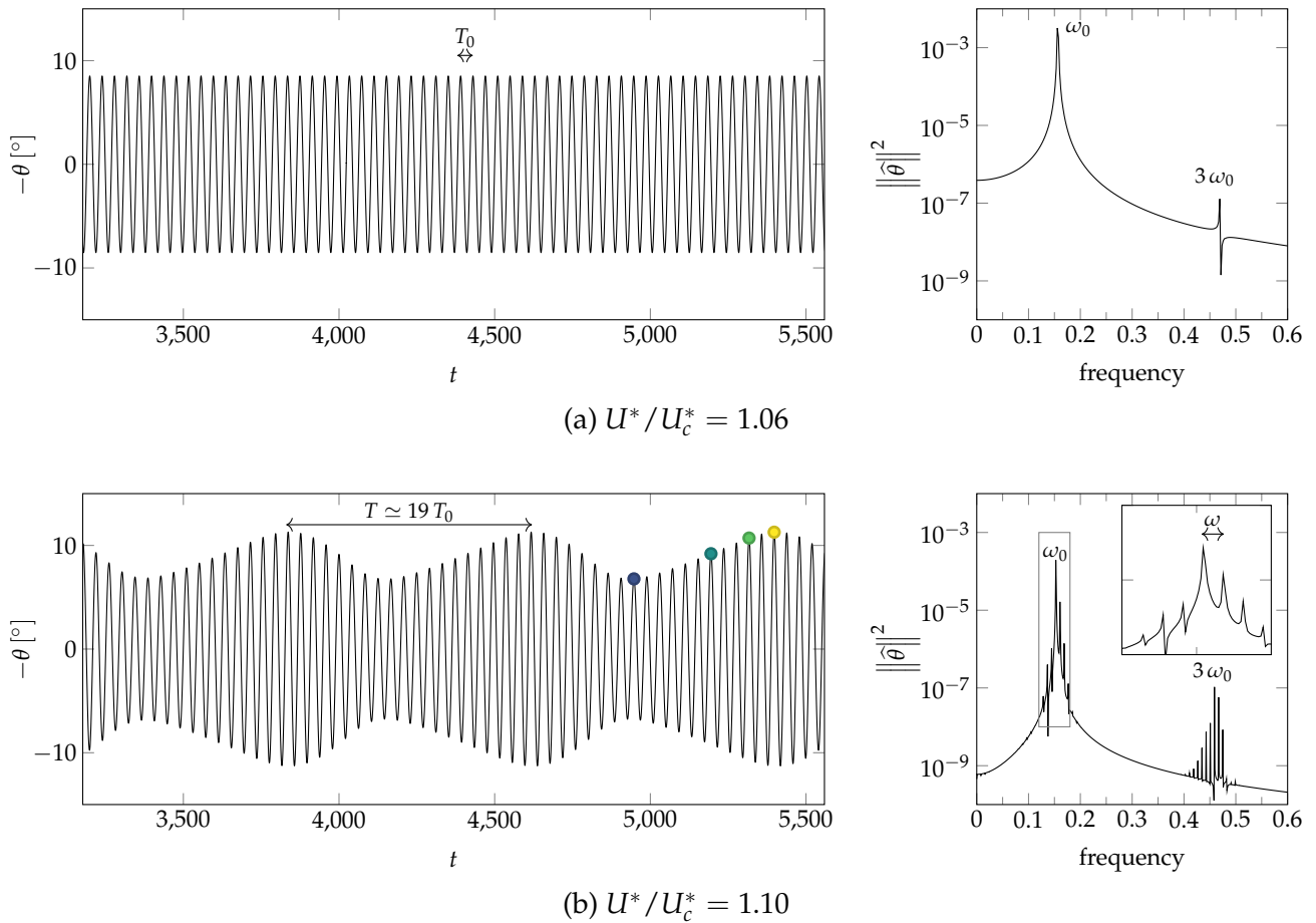
FIGURE 6.2: (a) Periodic and (b) quasi-periodic oscillations of the pitching angle displayed with time series (left column) and Fourier spectra (right column) for two reduced velocities above the critical flutter velocity U_c^* . \omega_0 corresponds to the fundamental frequency of the periodic solution, while \omega is the small frequency shift.
