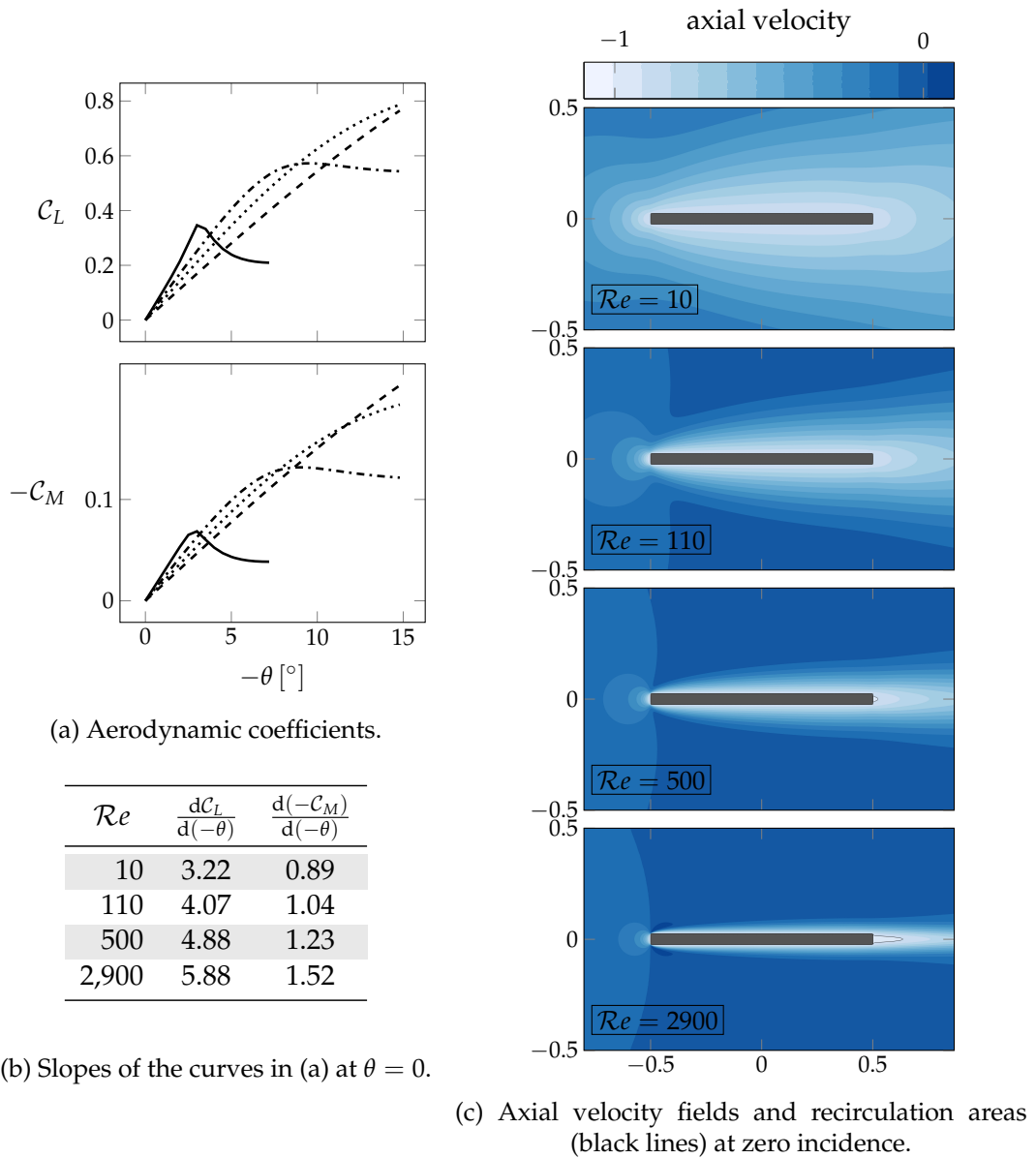
FIGURE 4.11: Features of the steady flow for different Reynolds numbers. In (a), the C_L(\theta) and C_M(\theta) curves for Re = 10 (dashed), Re = 110 (dotted), Re = 500 (dashdotted) and Re = 2900 (solid) are shown. In (b), the slopes of those curves at \theta = 0 are tabulated. In (c), we present the steady solutions associated to the different Reynolds at zero incidence.
