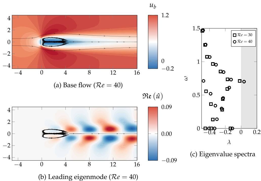
FIGURE 7.2: Results of the linear stability analysis for the two-dimensional configuration. Streamwise velocity u of (a) the steady-state solution and (b) the real part of the unstable eigenmode. (c) Eigenvalues are depicted with circles in the complex plane (growth rate \lambda and frequency \omega ). The unstable region is shown in gray. Only eigenvalues with positive frequencies are shown, the spectrum being symmetric.
