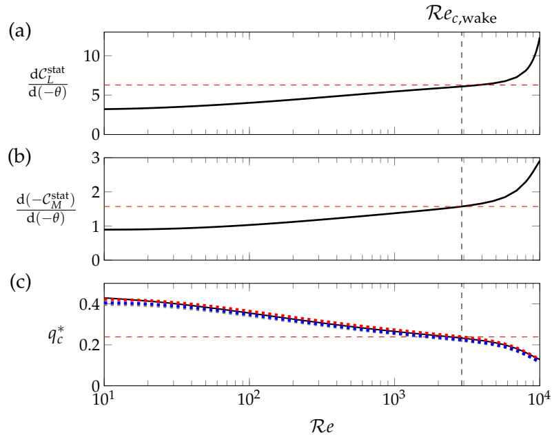
FIGURE 4.14: Calibration of Theodorsen and quasi-steady models with the slopes of the steady C_L^{\text{stat}}(\theta) and C_M^{\text{stat}}(\theta) curves, evaluated at \theta_0 = 0 . The slopes of the lift and moment coefficients are shown as a function of Re in (a) and (b) respectively. The critical dynamic pressure computed with full Navier–Stokes (solid line), Theodorsen (dotted red) and quasi-steady models (QSM1 in dotted gray and QSM2 in dotted blue) are presented in (c) for a large mass ratio \tilde{m} = 10^4 . The horizontal dashed line shows the threshold predicted by original (non-calibrated) Theodorsen theory. The vertical dashed line materializes the critical Reynolds for the wake instability.
