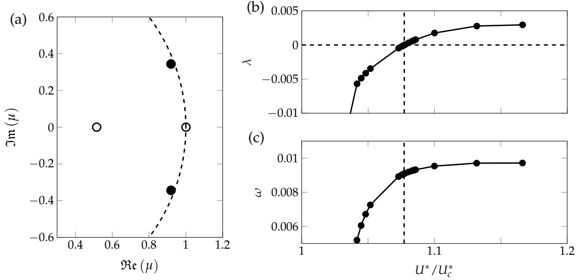
FIGURE 6.6: (a) Floquet multipliers computed for the periodic base flow shown in fig. 6.3 for the reduced velocity U^*/U_c^* = 1.073 . The stability boundary (unit circle) is depicted by the dashed curve. (b-c) Evolution of the growth rate \lambda and frequency \omega of the leading Floquet mode (black dots in figure a) as a function of the reduced velocity. The mode becomes unstable at a critical velocity U^*/U_c^* \simeq 1.078 .
