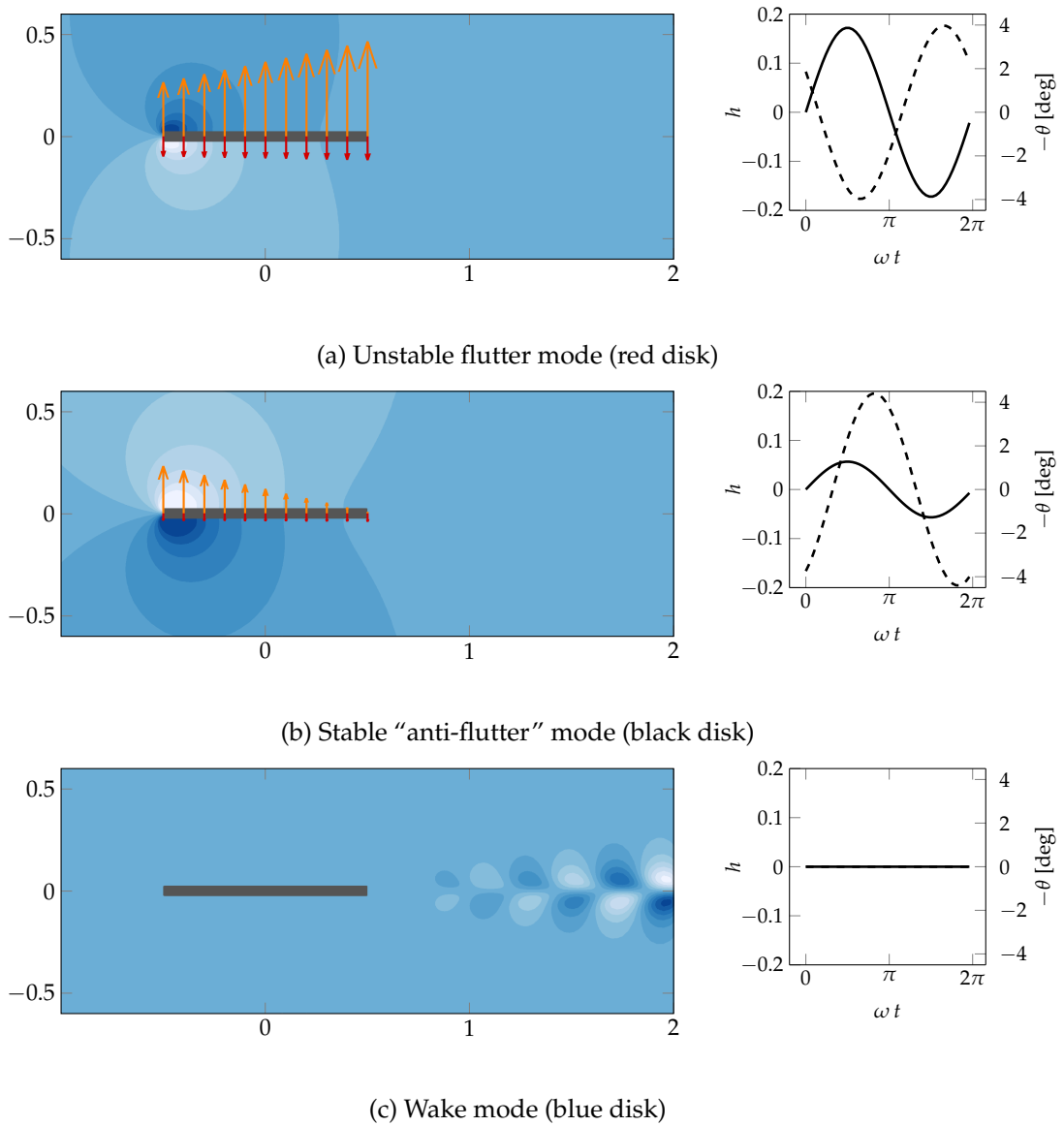
FIGURE 4.2: Visualisation of the three leading eigenmodes of fig. 4.1b. For each subfigure, the left part represents a snapshots of the mode at t=3\pi/4 , where the blue colormap represents the pressure field, while the arrows materialise the solid displacement (orange) and velocity (red) vectors. On the right part, we show the time signals for the vertical displacement (solid line) and pitching angle (dashed line). The modes are normalized to unit solid mechanical energy.
