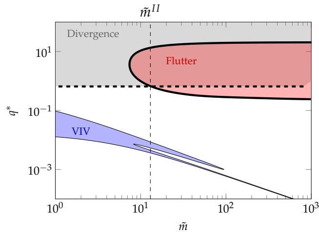
FIGURE 4.10: Alternative representation, using dynamic pressure q^* , of the neutral curves of fig. 4.9. Same color conventions are used.
