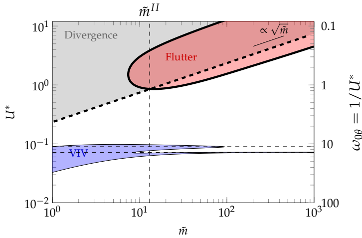
FIGURE 4.9: Neutral curves in the plane (\tilde{m}, U^*) for flutter (red area, thick line), divergence (gray area, dashed thick line) and VIV (blue area, thin line) instabilities ( Re = 2900 ). The thin horizontal dashed lines materialize the reduced velocities for which the heaving (lower line) and pitching (upper line) natural frequencies equal the VIV mode frequency \omega_w .
