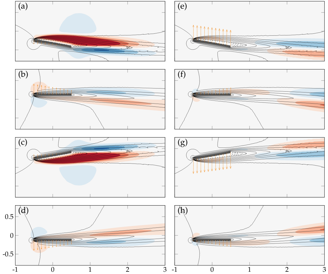
FIGURE 6.7: Periodic evolution of the flow and solid displacement fields for the unstable Floquet mode (with positive frequency \omega > 0 ) at U^*/U_c^* = 1.10 . The streamwise velocity (red and blue) and solid displacement (orange arrows) fields are shown for the (a-d) real and (e-h) imaginary parts of the Floquet mode at instants (a,e) t = 0 , (b,f) t = T_0/4 , (c,g) t = T_0/2 and (d,h) t = 3T_0/4 .
