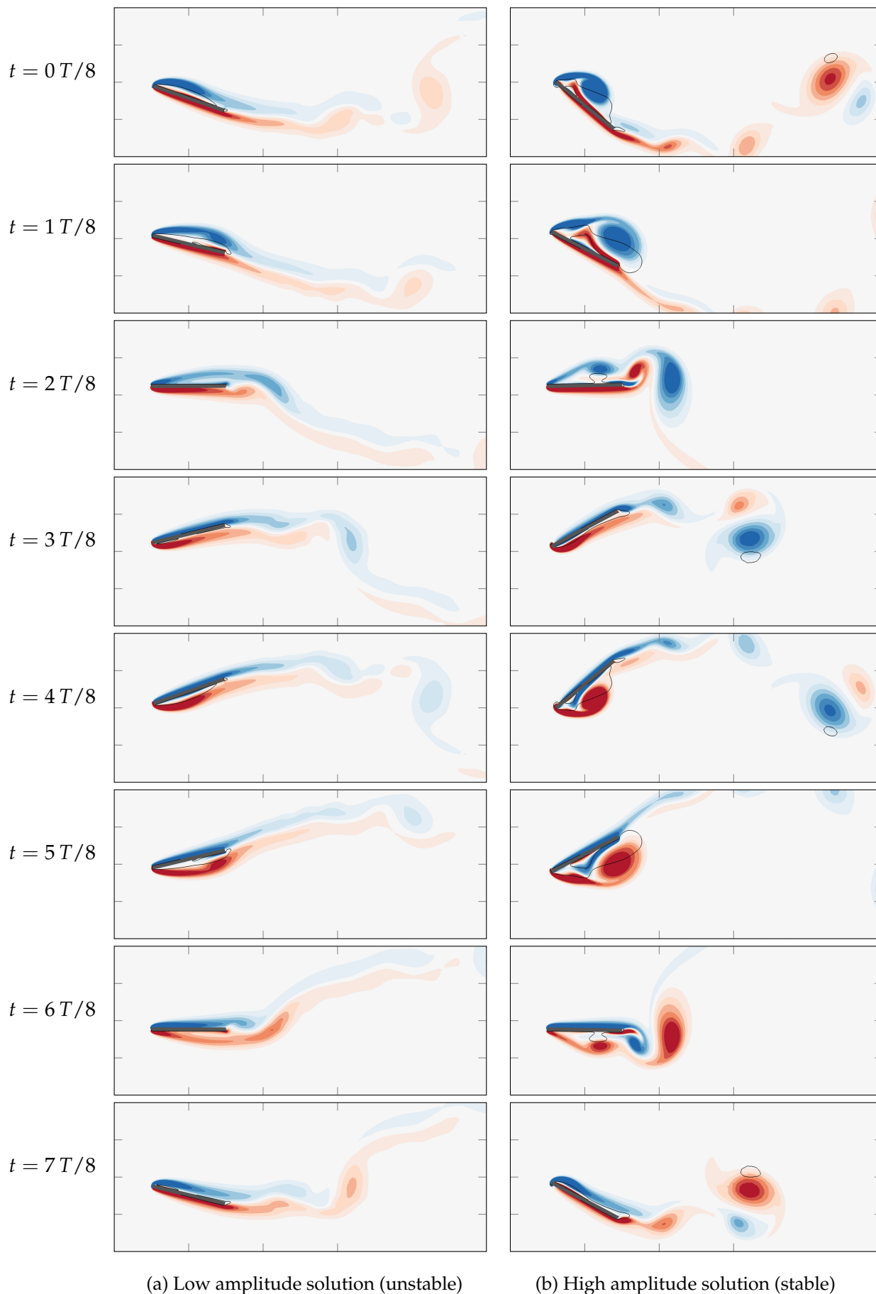
FIGURE 5.15: Vorticity snapshots of the two coexisting flutter LCO's in the subcritical case ( \tilde{m} = 60 , U^*/U_c^* = 0.95 ).
