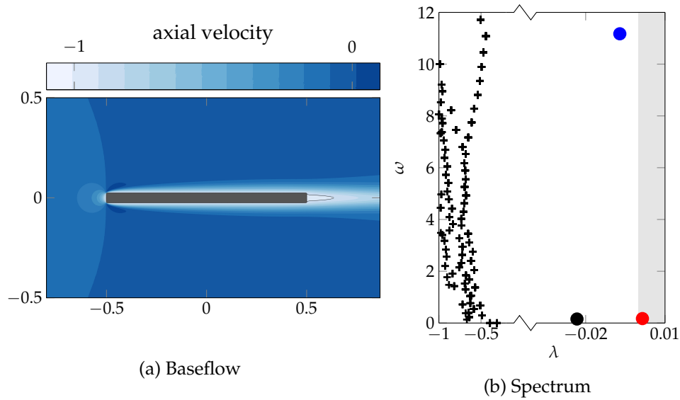
FIGURE 4.1: Linear stability analysis of the steady baseflow illustrated in 4.1a. The spectrum of the fluid-structure operator \mathcal{J} at ( U^* = 4.7 , Re = 2900 , \tilde{m} = 1000 ) is shown in 4.1b. The leading mode, marked with a red disk, is slightly unstable and is responsible for the flutter instability. It is depicted in fig. 4.2a. All modes marked by crosses correspond to the fluid modes that are present without any fluid structure coupling. In particular, the high-frequency wake mode (blue disk) is presented in fig. 4.2c.
