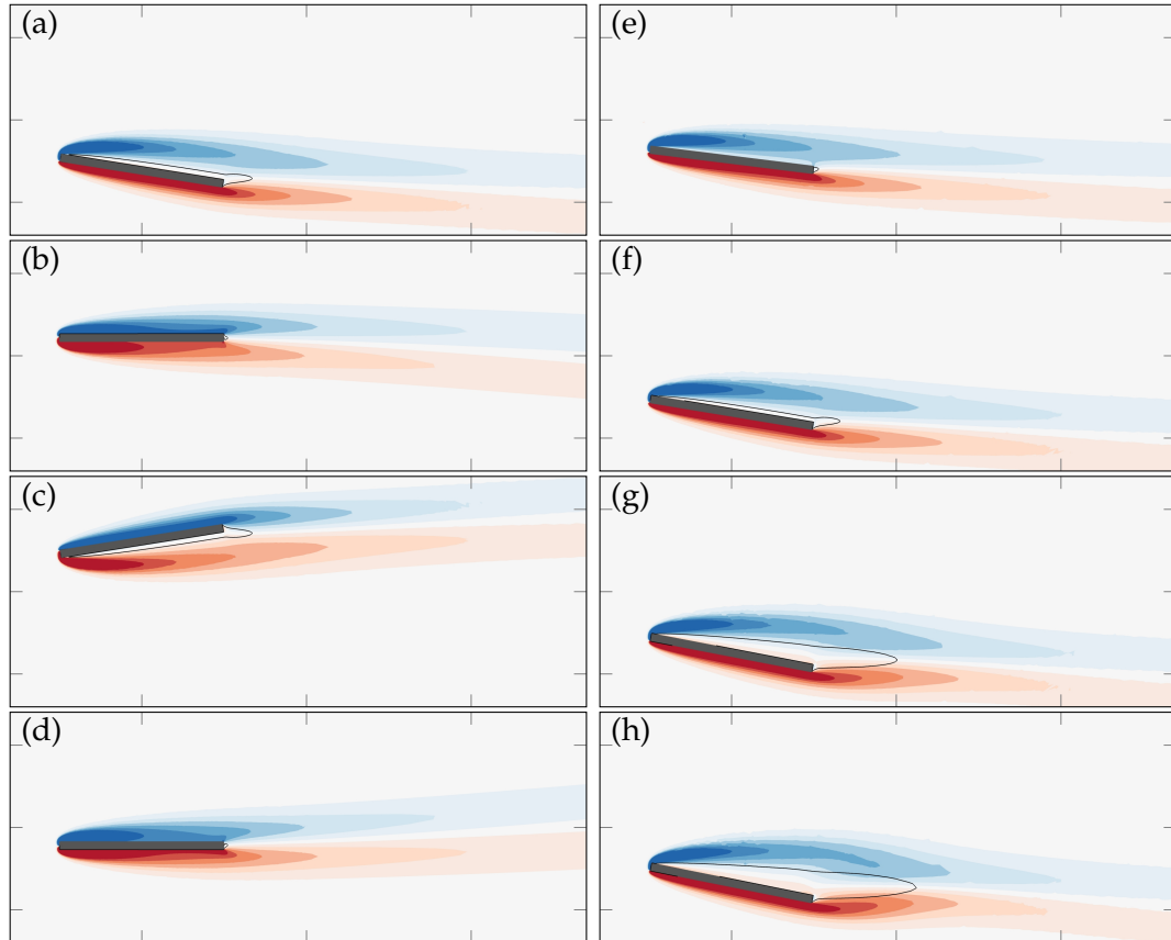
FIGURE 6.3: (a-d) Periodic and (e-h) quasi-periodic solutions displayed with the streamwise velocity field. The periodic solution obtained for U^* = 1.073U_c^* is displayed at four instants of the period (a) t = 0 , (b) t = T_0/4 , (c) t = T_0/2 and (d) t = 3T_0/4 . The slow evolution of the quasi-periodic solution obtained for U^* = 1.1U_c^* is shown by displaying the solution at the four instants marked by colored disks in fig. 6.2(b). The thin black curves, corresponding to the contour of zero streamwise velocity, delimit regions of flow recirculation.
