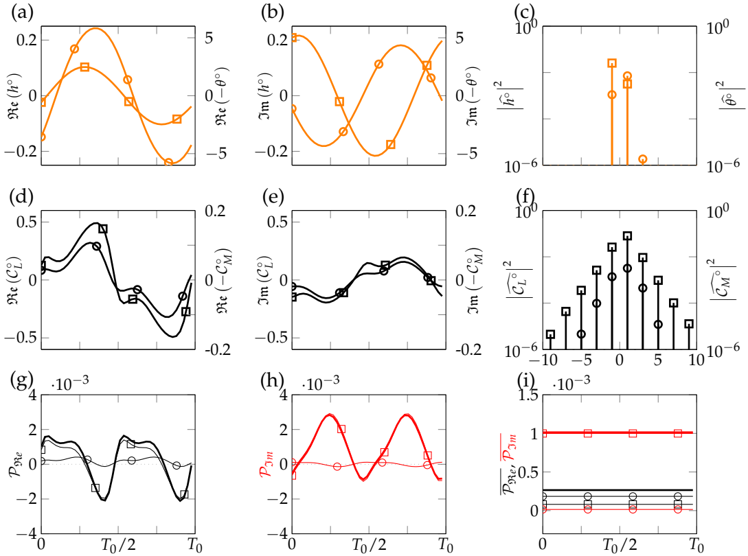
FIGURE 6.8: Periodic evolution of the (a-c) heaving (squares) and pitching (circles) components and (d-f) lift (squares) and moment (circles) coefficients for the unstable Floquet mode (with positive frequency \omega > 0 ) at U^*/U_c^* = 1.10 . (g-h) Instantaneous power provided by the fluid to the solid: total power (thick line), heaving power (squares) and pitching power (circles). The real and imaginary parts of the time signals are displayed in (a,d,g) and (b,e,h), respectively. The modulus of the Fourier harmonics are presented in (c,f). (i) Mean power of the real (black) and imaginary (red) parts of the signal corresponding to the time series in (g) and (f) respectively.
