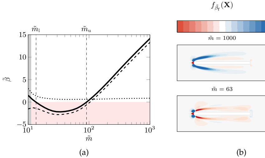
FIGURE 5.6: Fluid and geometric nonlinearities. (a) Fluid \tilde{\beta}_f (dashed line) and geometric \tilde{\beta}_g (dotted line) contribution to the nonlinear coefficient \tilde{\beta} (solid line) as a function of the mass ratio, (b) Spatial distribution of \tilde{f}_{\tilde{\beta}_f}(\mathbf{x}) (its integral over the domain gives the value of the fluid contribution \tilde{\beta}_f ) for two values of the mass ratio corresponding to a supercritical bifurcation (top, \tilde{m} = 1000 ) and a subcritical bifurcation (bottom, \tilde{m} = 63 ). The Reynolds number is Re = 540 .
