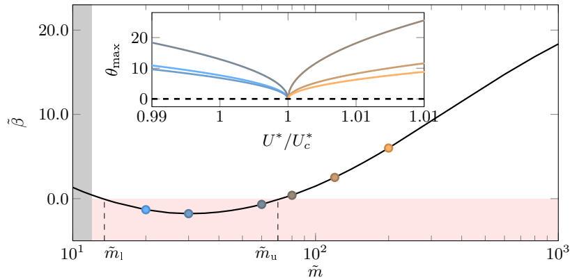
FIGURE 5.4: Nature of the flutter bifurcation at different mass ratio and constant Re = 500 . The value of the criticality indicator \tilde{\beta} , built from weakly nonlinear analysis, is shown as a function of mass ratio. In the insert the amplitude of \theta is represented as a function of U^*/U_c^* for the different mass ratio marked with solid symbols on the main curve ( \tilde{m} = 20, 30, 60, 80, 120, 200 ). Note that we do not investigate the range \tilde{m} < 12 materialized by the gray area, since for those low mass ratio a static divergence mode is already unstable when the flutter threshold U_c^* is reached (cf fig. 4.9). This scenario is out of the validity assumptions of the present weakly nonlinear analysis.
