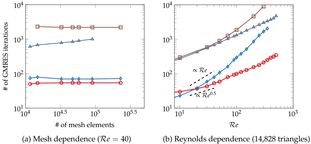
FIGURE 7.6: Influence of (a) the number of mesh elements and (b) the Reynolds number Re on the number of inner iterations required to solve eq. (7.12) with the mAL (—○—), PCD (—◇—), SIMPLE (—△—), and Stokes (—□—) preconditioners. The relative tolerance is set to 10^{-3} and the shift to zero.
