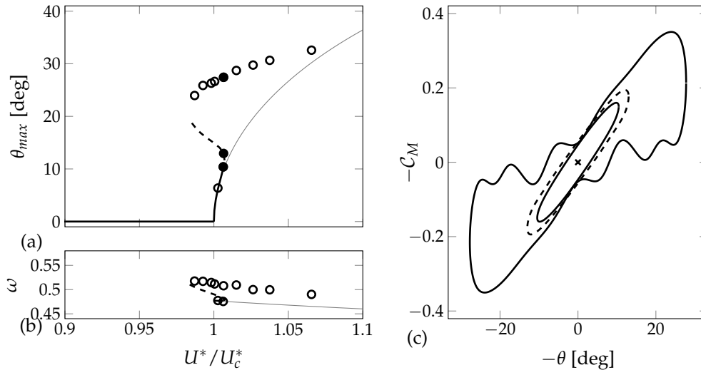
FIGURE 5.17: Bifurcation for intermediate mass ratio \tilde{m} = 120 ( Re = 500 ). Same legend as in fig. 5.12. The critical reduced velocity is U_c^* = 1.78 . The three LCO displayed in (c) corresponds to U^*/U_c^* = 1.006 .
