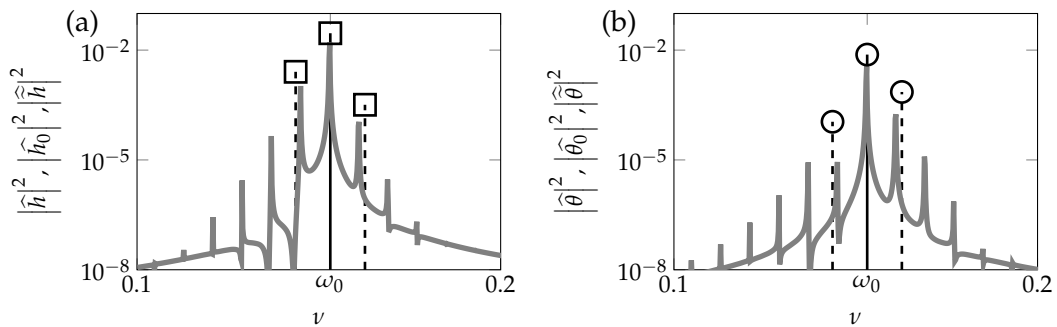
FIGURE 6.13: Comparison of the Fourier spectra of the base LCO \mathbf{q}_0 (solid peaks) and Floquet perturbation \tilde{\mathbf{q}} (dashed peaks) with respect to the fully nonlinear quasi-periodic time-marching solution (gray lines) for the heaving (a) and pitching (b) degrees of freedom ( U^*/U_c^* = 1.10 ). The amplitude \epsilon of \tilde{\mathbf{q}} is arbitrary.
