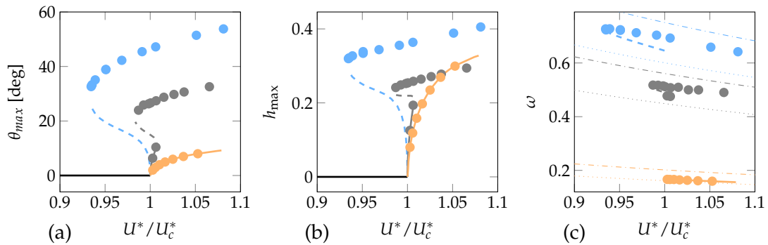
FIGURE 5.18: Transition from subcritical to supercritical bifurcations at low Reynolds number ( Re = 500 ) when increasing the mass ratio ( \tilde{m} = 60 in blue, \tilde{m} = 120 in grey and \tilde{m} = 1000 in orange). (a) Maximal pitching angle, (b) maximal heaving displacement and (c) frequency of the LCO as a function of U^*/U_c^* . Dots and curves correspond to results of time-marching and time-spectral methods, respectively, while solid and dashed curves distinguish stable from unstable LCOs. In (c), the natural heaving and pitching frequencies are represented by dotted and dash-dotted curves, respectively.
