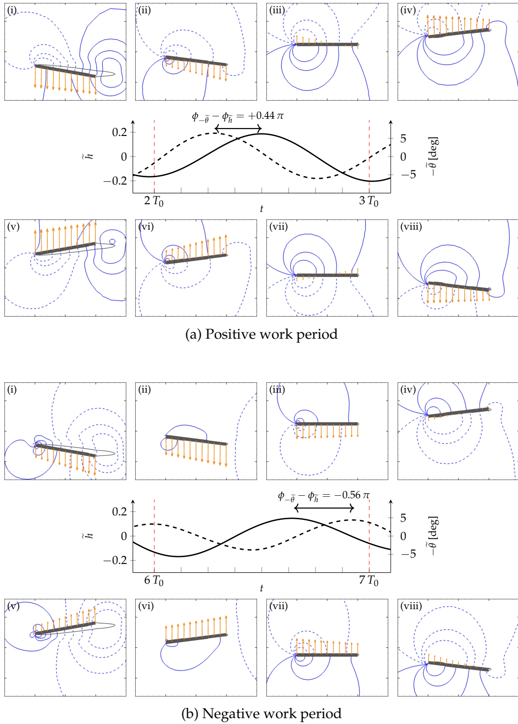
FIGURE 6.10: Temporal evolution of the quasi-periodic perturbation on two periods corresponding to (a) maximal fluid energy extraction by the solid and (b) maximal solid energy dissipation by the fluid, both indicated with vertical dashed lines in fig. 6.9. The heaving and pitching displacement are show with solid and dashed lines, respectively. Snapshots (i) to (viii) are taken at the instants t = n T_0 , t = (n + 1/8) T_0 , ..., t = (n + 7/8) T_0 ( n = 2 in (a) and n = 6 in (b)). They show the perturbation pressure field (blue contours, negative contours are dashed) and displacement vector (orange arrows). The thin black contour represents the recirculation zone of the LCO. The unperturbed position of the plate is displayed in these figures.
