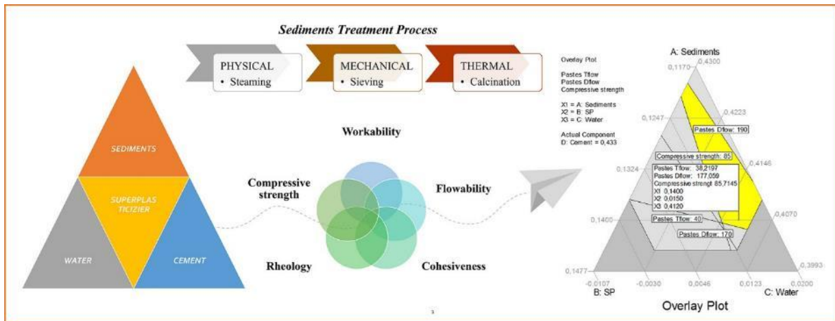
Figure 2-1: Graphical abstract
