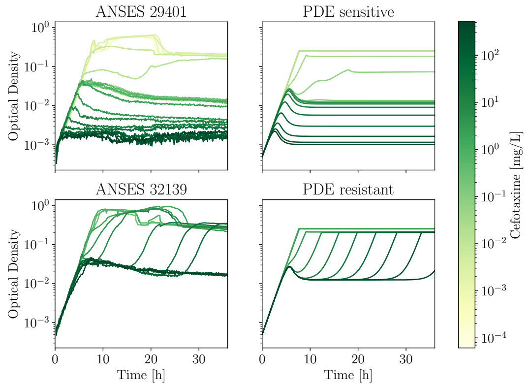
Figure 3.8: On the left are two clinical isolates (top sensitive, bottom resistant). On the right are simulations of the PDE model with similar behaviours.
