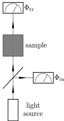
Figure 2.18: Measurement model.
