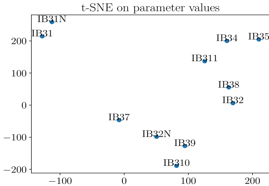
Figure 5.9: t-SNE on (the logarithms of) the parameter values.
