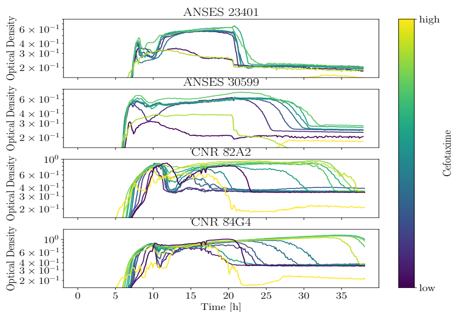
Figure 5.14: Zoom on the stationary phase of the growth curves of different stains submitted to different concentrations of antibiotics.
