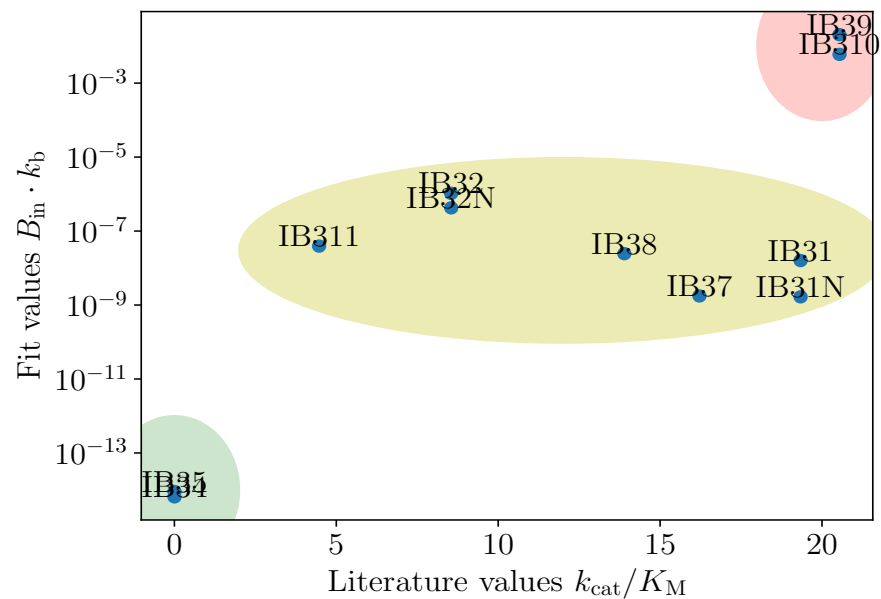
Figure 5.13: Comparison of the efficiency of \beta -lactamase per cell, from the model and from the literature. The Pearson correlation coefficient between k_{\text{cat}}/K_M and \log(B_{\text{in}} \cdot k_b) is 0.72, and the associated p-value of correlation is 0.013.
