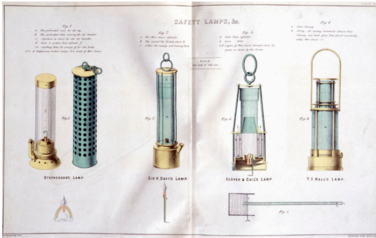
Figure 1-8 George Stephenson's safety lamp (left) compared with other miners' lamps. http://www.bbc.co.uk/schools/primaryhistory/famouspeople/george_stephenson/images/stephenson_lamp_small.jpg
