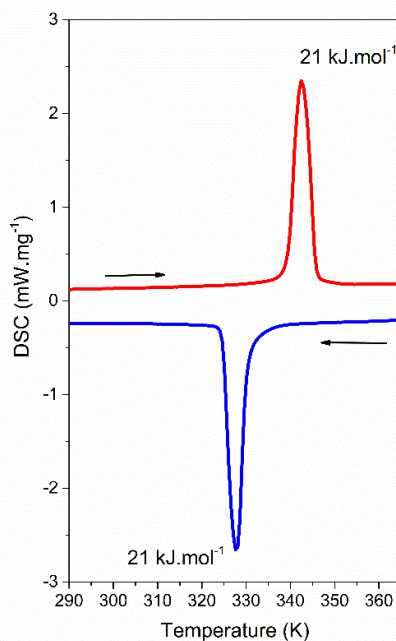
Fig 2.24) DSC measurement of complex 5 heating (red) and cooling (blue) (second thermal cycle).
