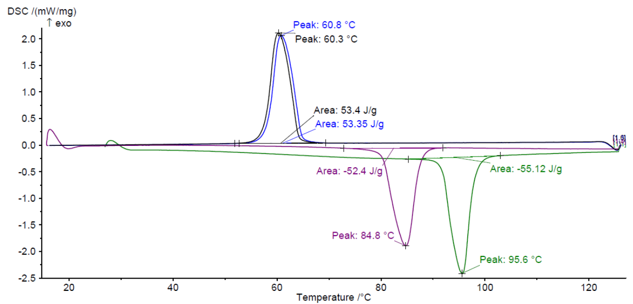
Fig A.2.1 DSC Thermograms for complexes 1 (up) and 2 (down). First heating cycle in green.
