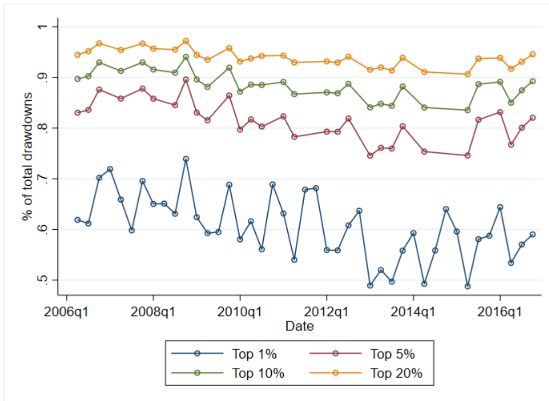
Figure 3.4: Cumulative distribution of drawdowns
