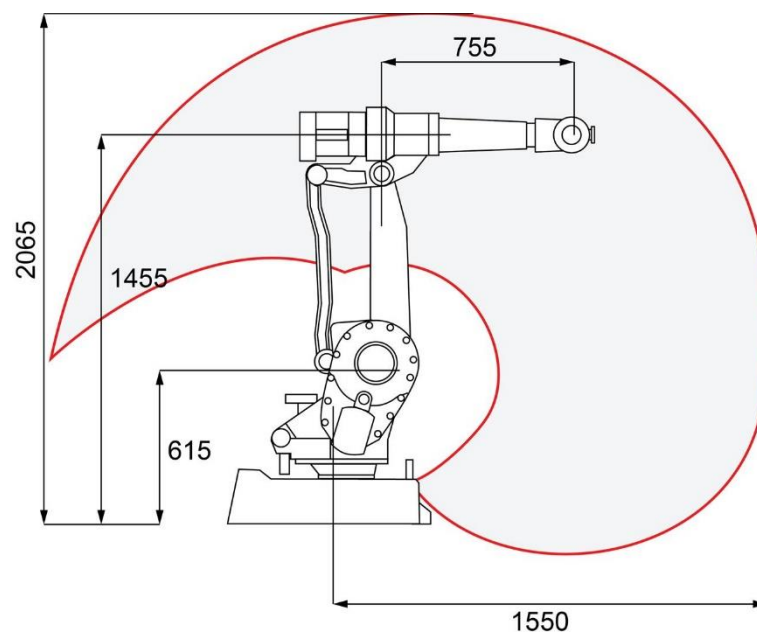
Figure 1.12 Working envelop of ABB IRB 2400/16 robot.
