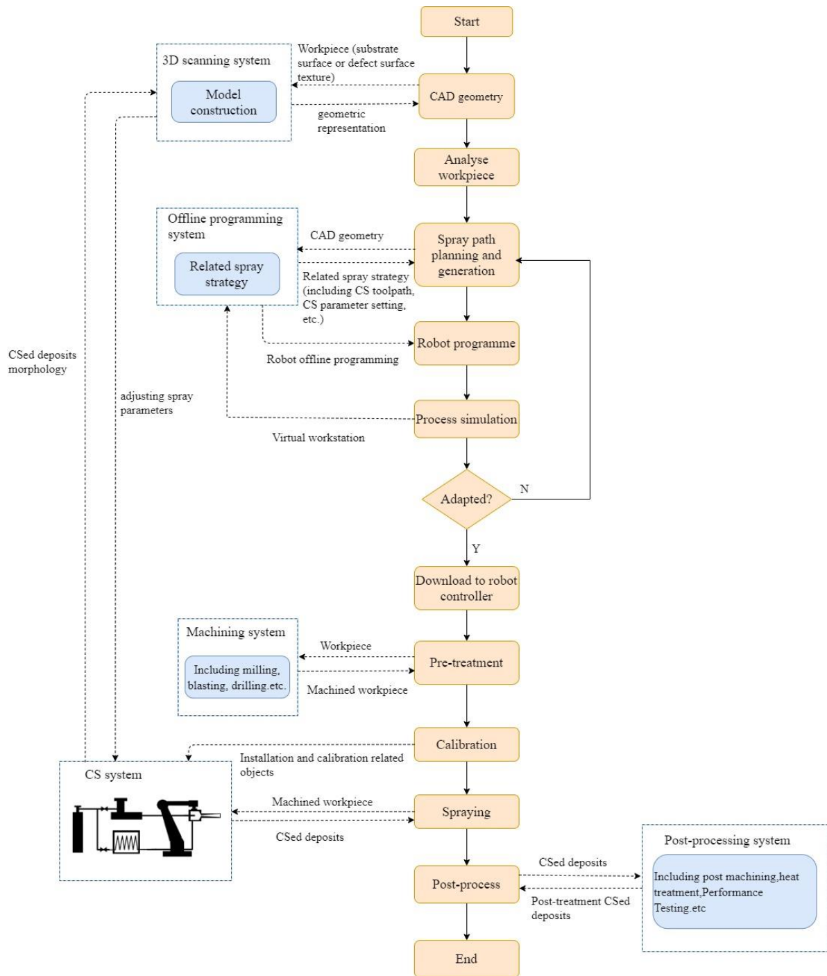
Figure 2.7 Flowchart of CSAM process.
