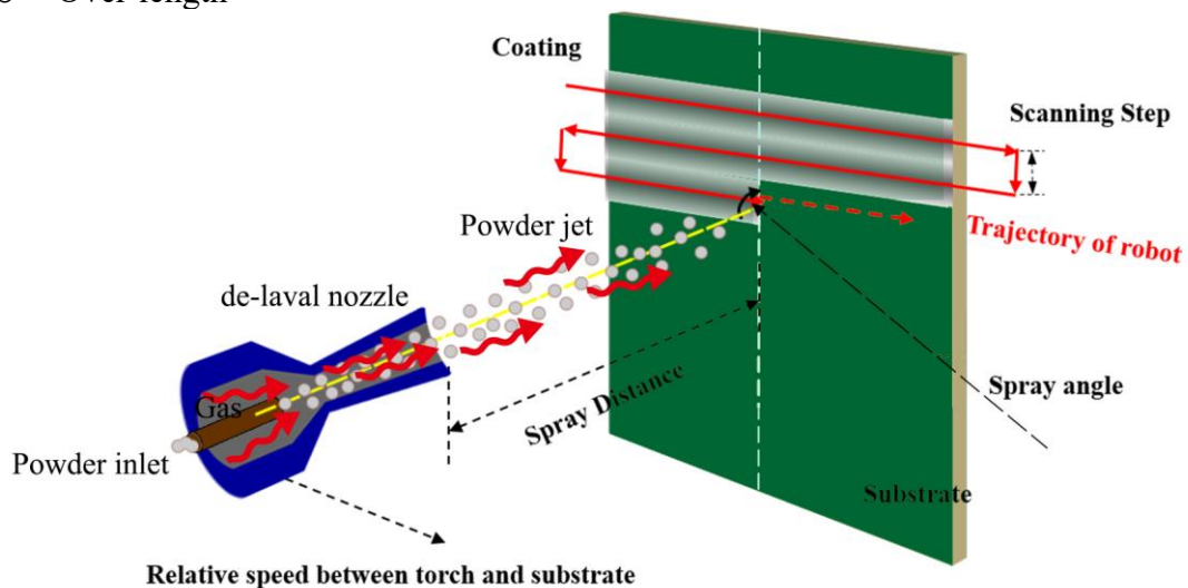
Figure 1.3 Kinematic parameters in the cold spraying process.
