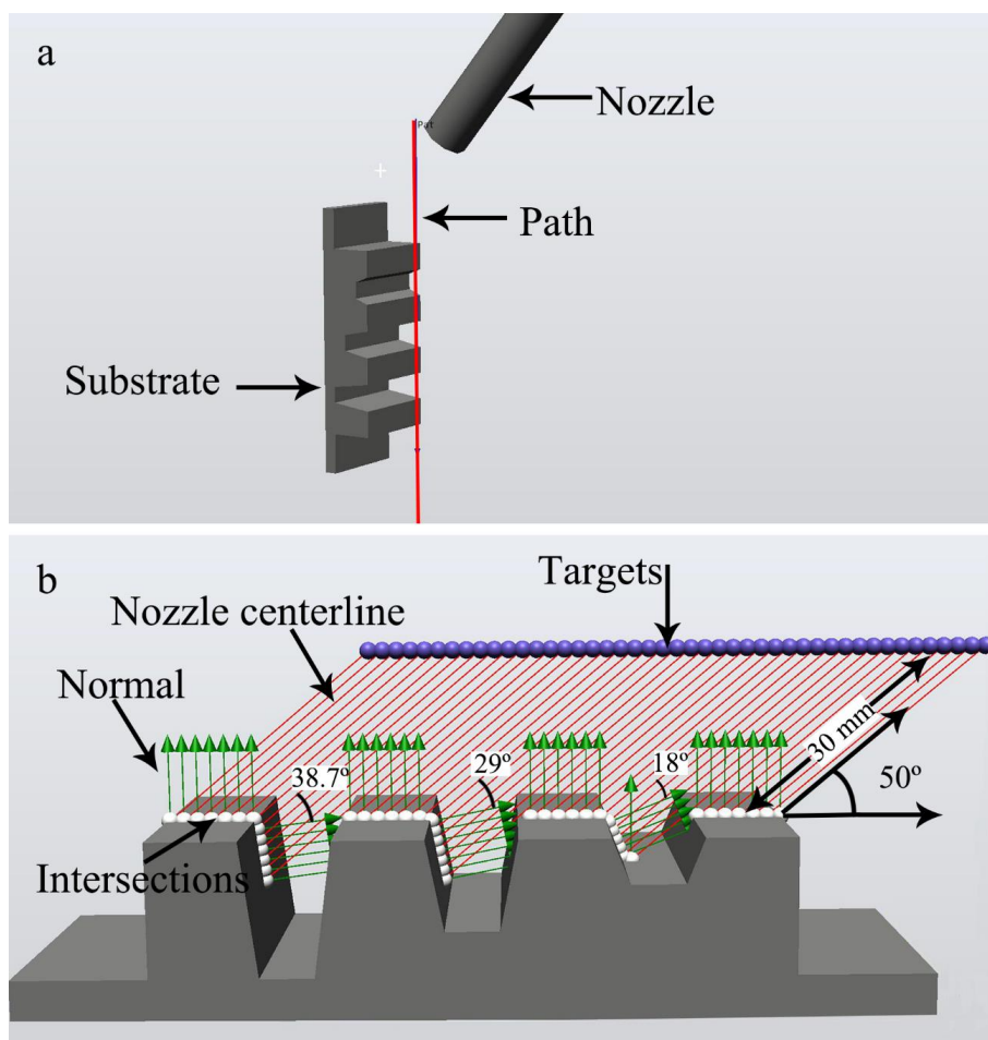
Figure 3.17 (a) Generation of trajectory; (b) target points for coating thickness simulation.
