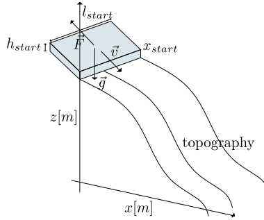
Figure 5.4: The avalanche model.
