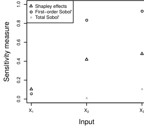
Figure 2.5: Comparison between Shapley effects and Sobol' indices when inputs are correlated on a linear model with three Gaussian inputs. X_1 is independent from X_2 and X_3 , and X_2 and X_3 are highly correlated (correlation \rho = 0.9 ).
