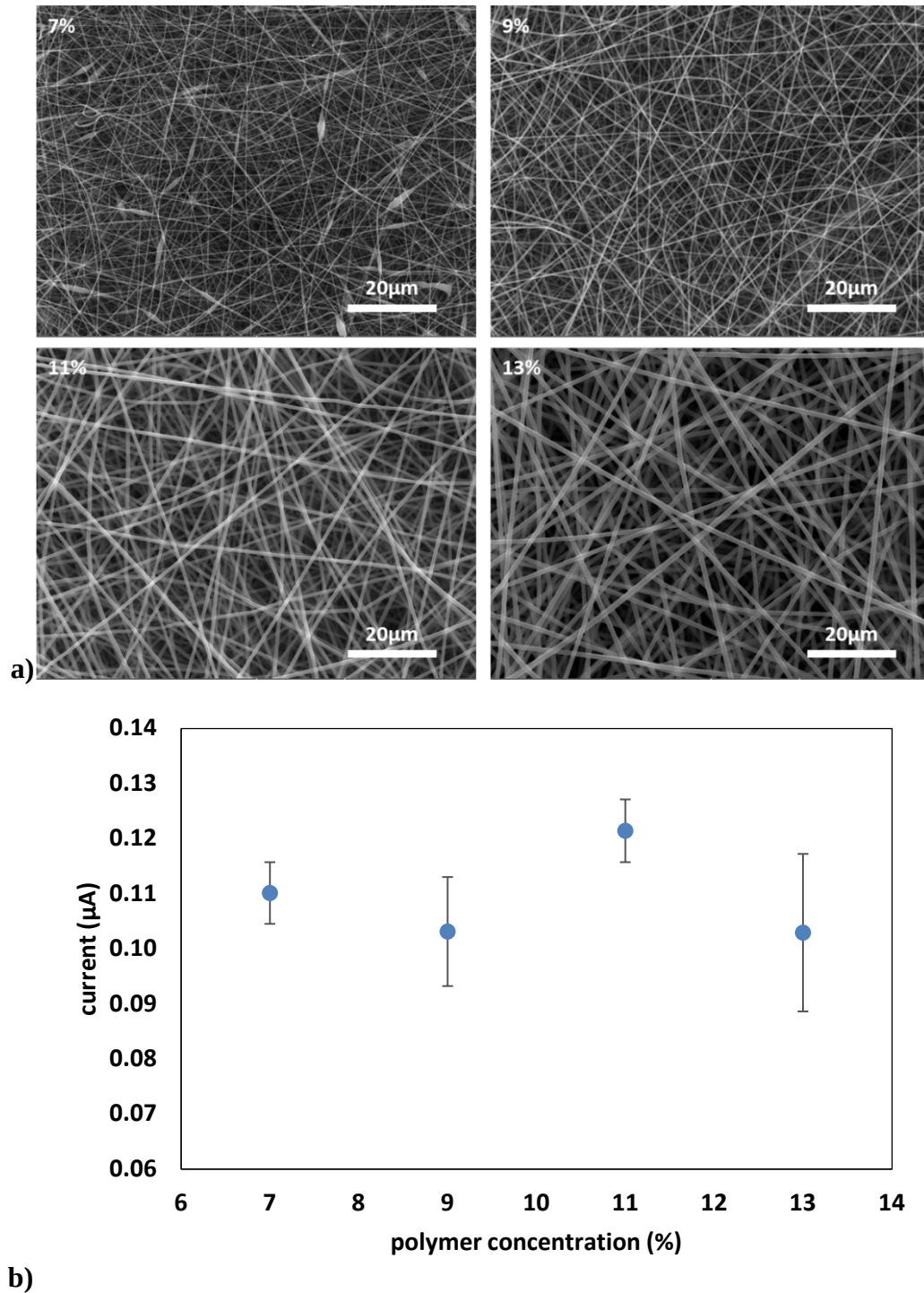
Fig. 3.8 a) SEM images of PLA fibers fabricated from polymer solutions at various concentrations. b) Evolution of the current as a function of the polymer concentration.
