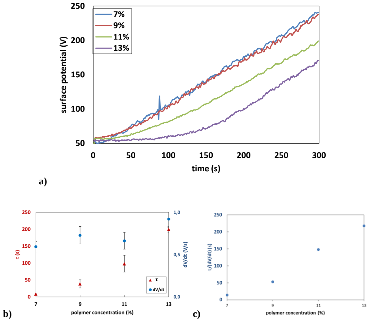
Fig. 3.9 a) Examples of experimental curves of the surface potential as a function of the polymer concentration. b) Characteristic time \tau and slope \frac{dV}{dt} = i\dot{R}_m and c) \tau/\left(\frac{dV}{dt}\right) ratio as a function of the polymer concentration.
