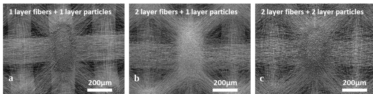
Fig. 4.36 SEM images of multilayer samples formed by coupling different layers of PLA fibers and PCL 14k particles (a: bilayer samples by coupling one layer of PLA fibers and one layer of PCL 14k particles; b: two layers of PLA fibers and one layer of PCL particles alternately; c: two layers of PLA fibers and two layers of PCL particles alternately)
