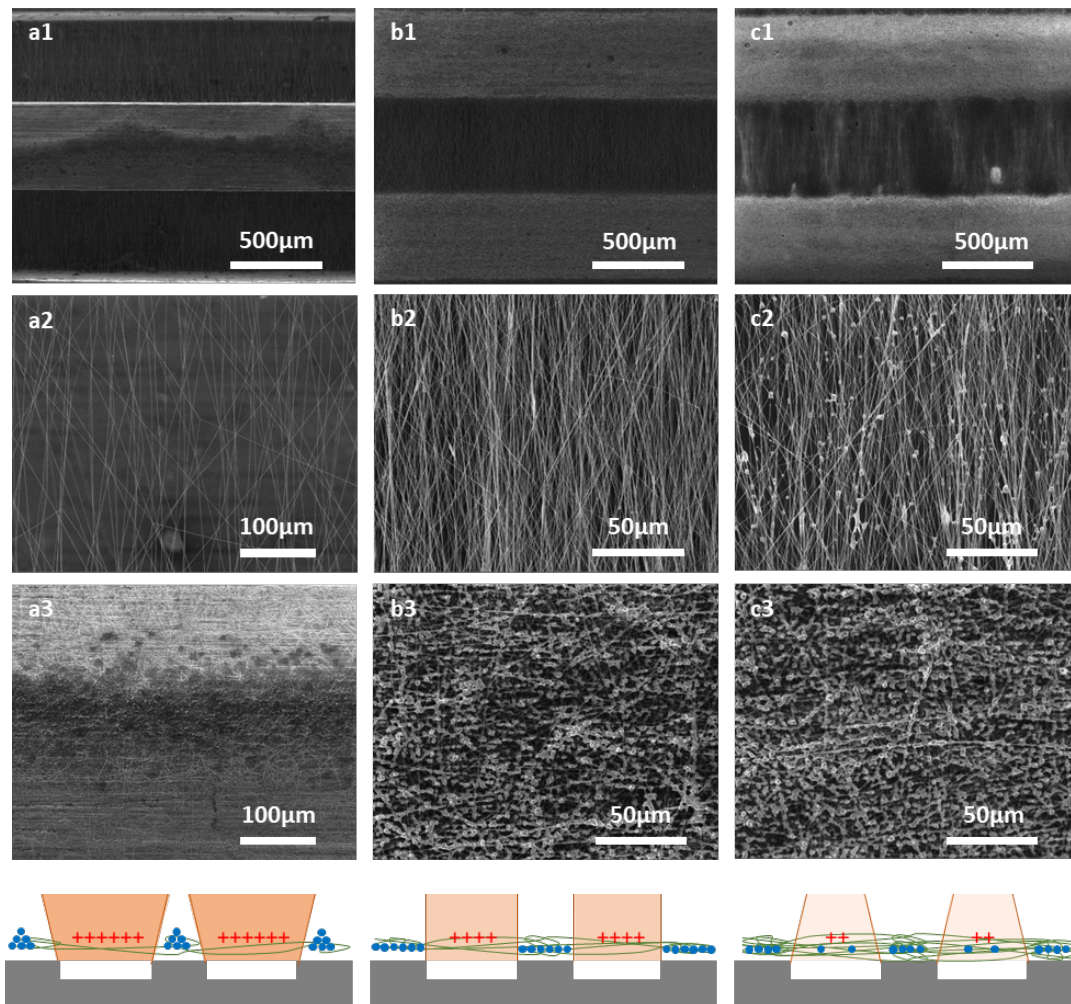
Fig. 4.19 Bilayer samples obtained from the deposition of a first layer of PLA fibers electrospun during a time t_{spin} covered by a layer of electrosprayed PCL 14k particles on the striated collector (a: t_{spin} = 15s , b: t_{spin} = 3min and c: t_{spin} = 5min ). a1, b1, c1 show grooves and gaps; a2, b2, c2 are pictures taken over the suspended fibers; a3, b3, c3 are pictures taken over the grooves.
