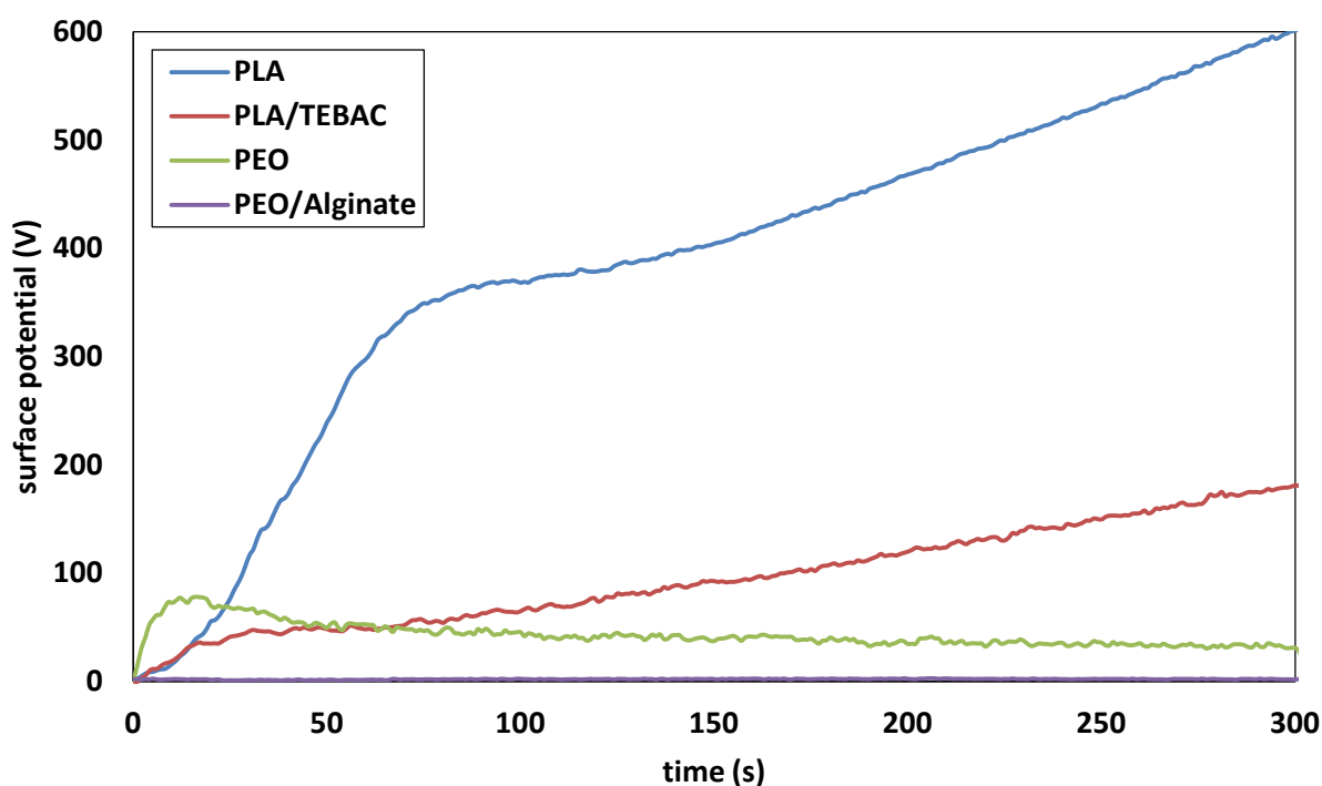
Fig. 4.25 Curves of surface potential of four types of fibers generated on the grid collector.
