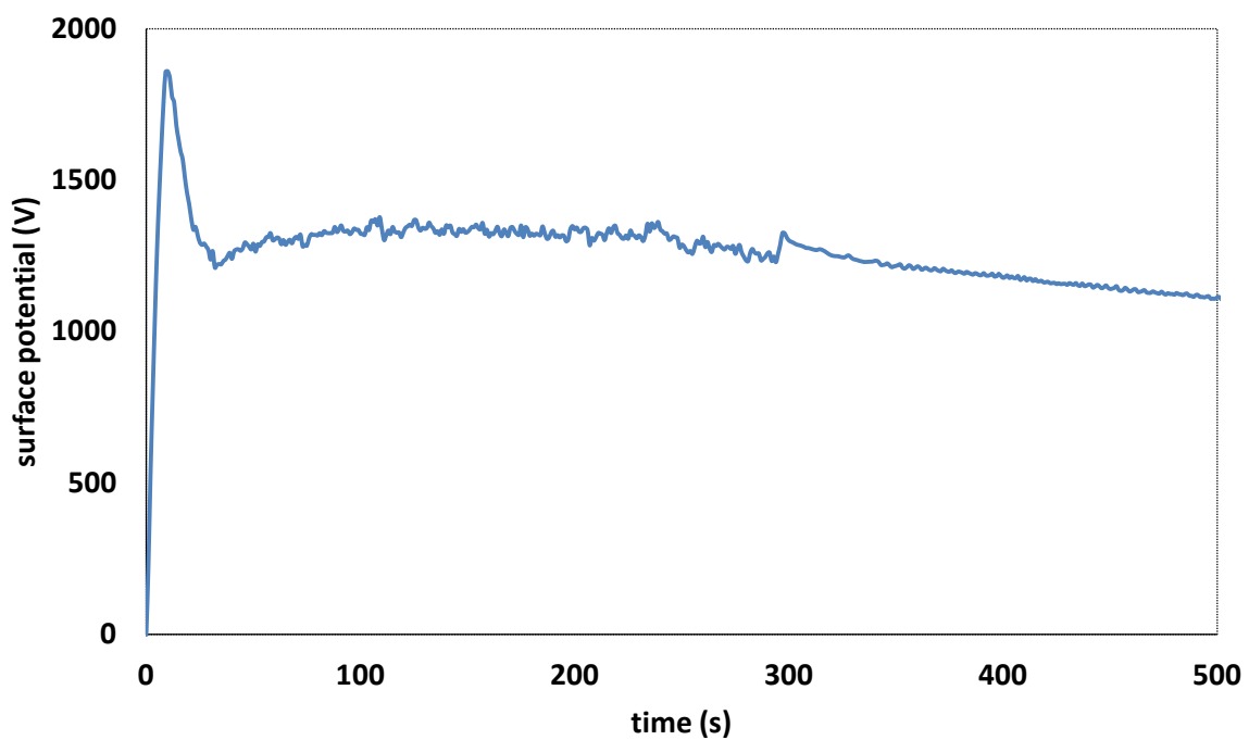
Fig. 4.27 Comparison of morphology of bilayer samples generated by coupling PLA fibers with PCL 14k particles on the grid and the intensity of surface potential induced by PLA fibers on a single gap collector with a gap = 3 mm. Electrospinning stopped at 300 s.
