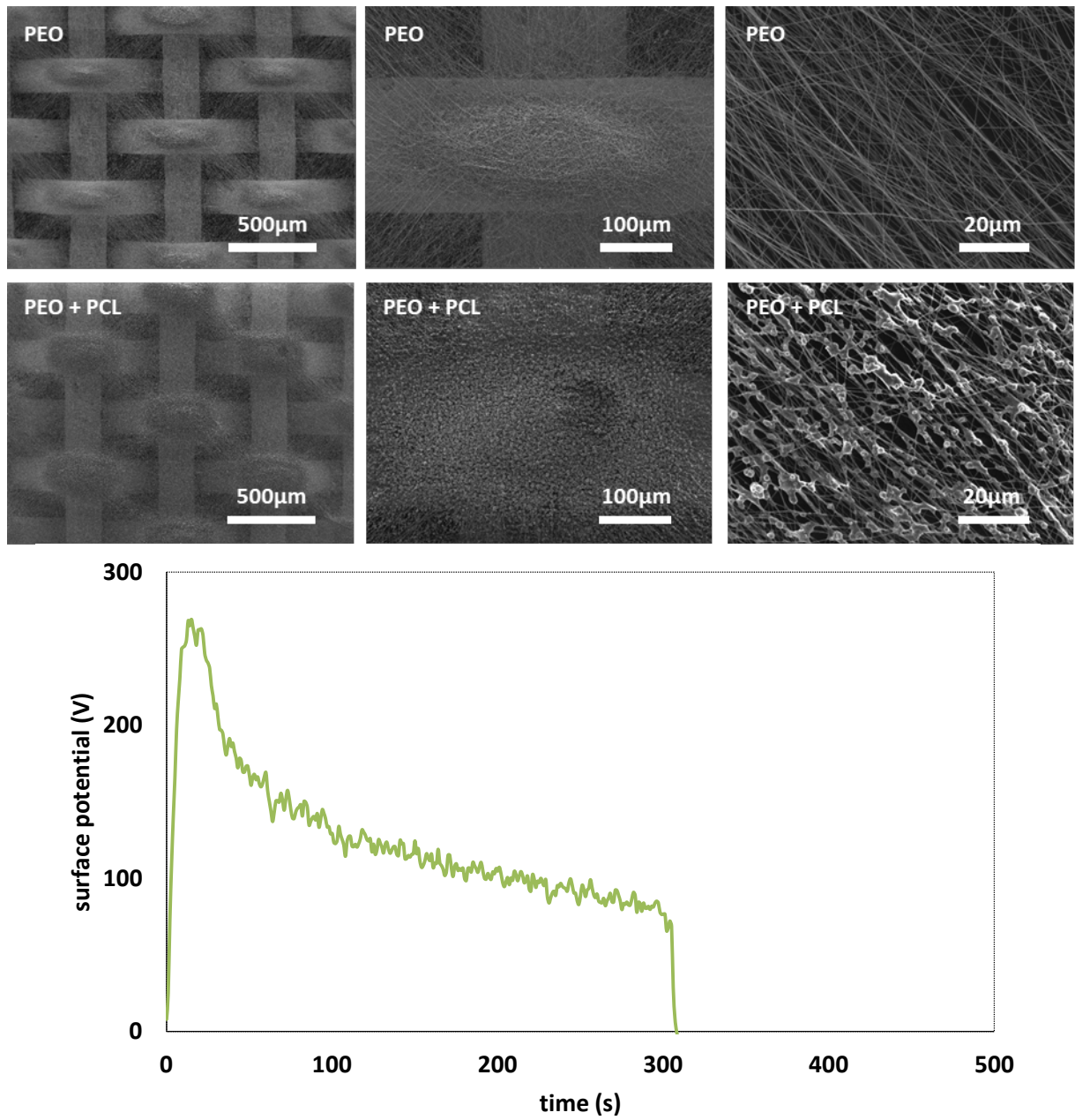
Fig. 4.30 comparison of morphology of bilayer samples generated by coupling PEO fibers with PCL 14k particles on the grid and the intensity of surface potential induced by PEO fibers on a single gap collector with a gap = 3 mm. Electrospinning stopped at 300 s.
