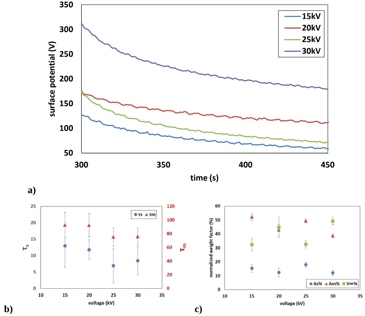
Fig. 3.15 a) Examples of curves giving the surface potential decay as a function of time for various applied voltage. b) Short and medium times and c) normalized weight factors as a function of applied voltage on the emitter.
