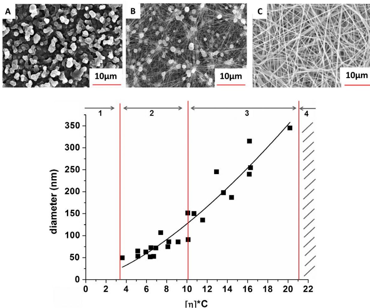
Fig. 1.2 SEM images of electrospayed PCL particles (a), beaded PCL fibers (b), electrospun PCL fibers (c) and variation of fibers average diameter with [\eta]C (d): 1: electrospaying, 2: beaded electrospun fibers, 3: bead-free electrospun fibers and zone 4: no electrospinning
