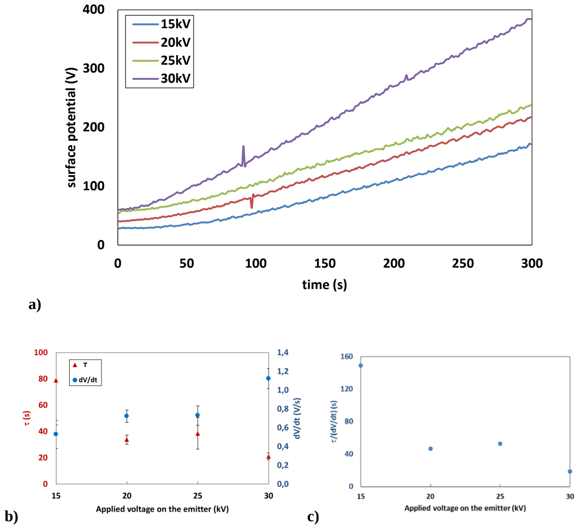
Fig. 3.6 a) Examples of experimental curves of the surface potential as a function of time for various applied voltages. b) Characteristic time \tau and slope \frac{dV}{dt} = i\dot{R}_m and c) \tau / \left(\frac{dV}{dt}\right) ratio as a function of the applied voltage.
