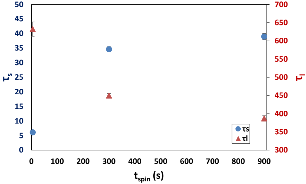
Fig. 4.15 Short \tau_s and long \tau_l characteristic times of the surface potential decay of suspended PLA fibers for a gap g = 3 \text{ mm} and for different electrospinning times t_{\text{spin}}
