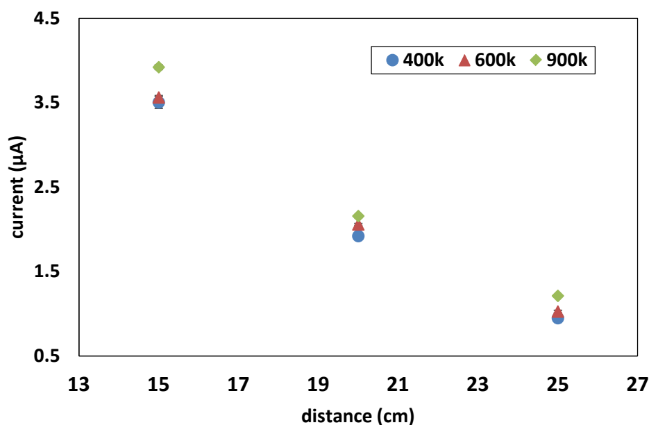
Fig. 3.19 comparison of the current formed by electrospinning PEO fibers with different molar masses in different distances
