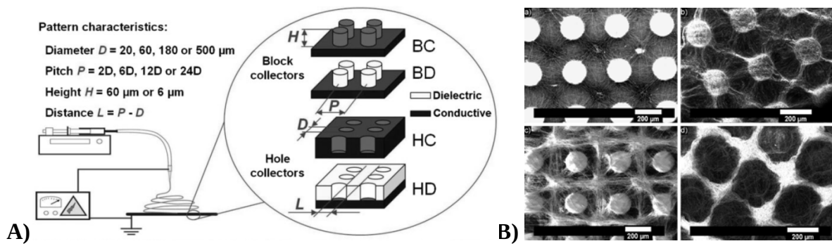
Fig. 1.19 A) Electrospinning on micropatterned collectors with different characteristic sizes and electrical properties. B) Nanofibrous membranes obtained with Blocks of D=180\mu\text{m} , H=60\mu\text{m} and L=3H=360\mu\text{m} . BC collector: (a) Topside view and (b) downside view. BD collector: (c) topside view and (d) downside view. Reprinted with the permission from [112]
