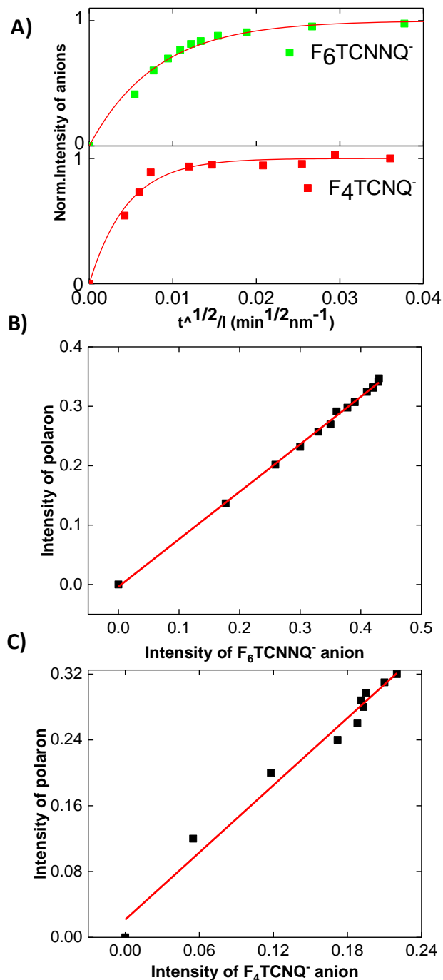
Figure 4.8. A) Plot of normalized absorptions of both F_6TCNNQ^- ( \lambda=1158 nm) and F_4TCNQ^- ( \lambda=1158 nm) vs t^{1/2}/l to determine the diffusion coefficients. B)-C) Plot of absorbance of the dopant anions vs that of the polarons (2500 nm). The linear fit supports integer charge transfer between C_{12} -PBTBT and both F_4TCNQ^- and F_6TCNNQ^- .
