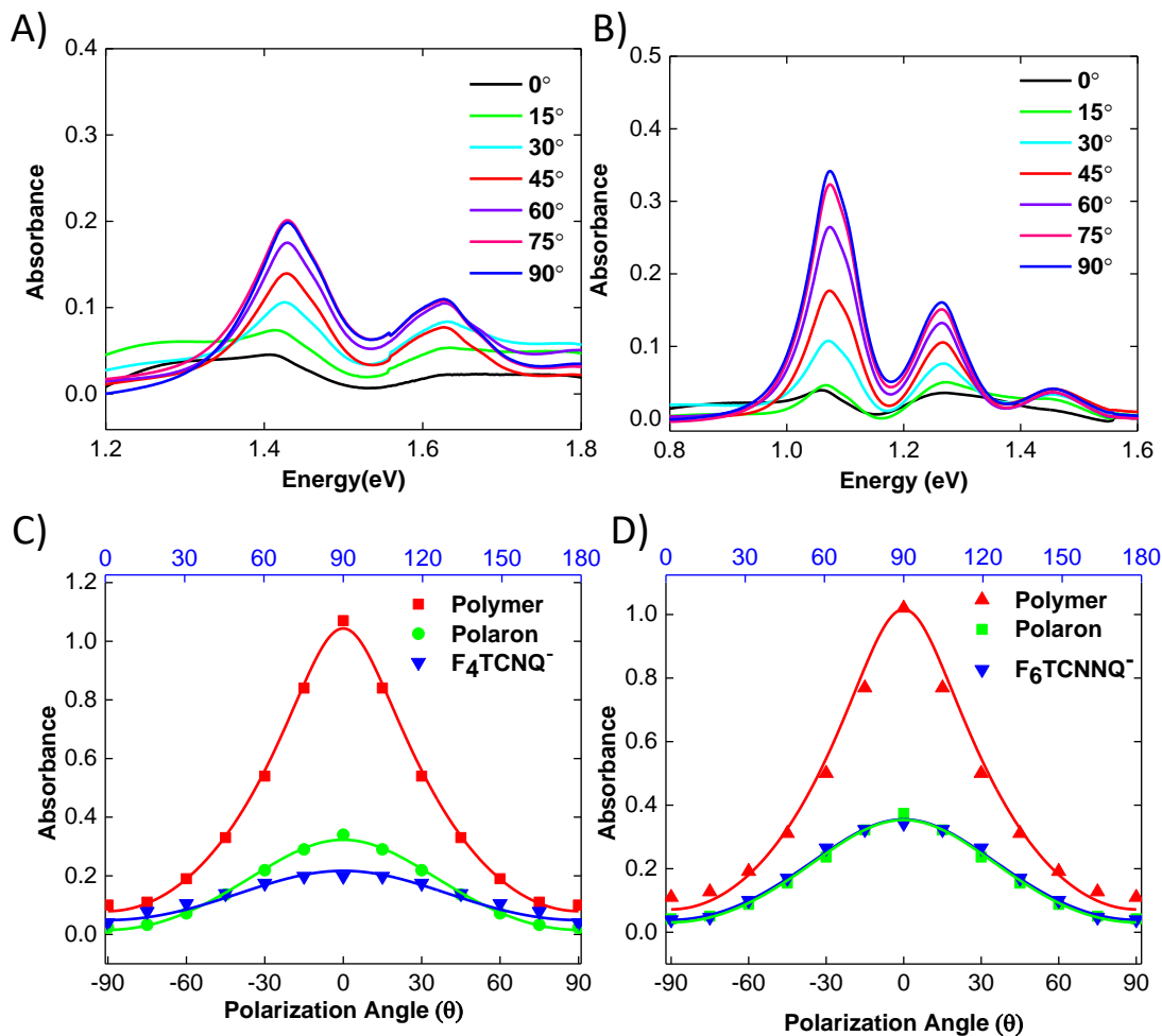
Figure 4.6. Absorbance of the dopant anions after subtracting the background absorbance of the polaronic contribution P2 for A) F_4TCNQ^- and B) for F_6TCNNQ^- . C) Angular distribution of absorption bands of pristine C_{12} -PBTTT before doping, the F_4TCNQ^- anion ( \lambda=873\text{nm} ) and the P1 band ( \lambda=2500\text{nm} ). D) Angular distribution of the absorption bands of oriented pristine C_{12} -PBTTT before doping, the F_6TCNNQ^- anion ( \lambda=1158\text{nm} ) and the polaronic P1 band ( \lambda=2500\text{nm} ).
