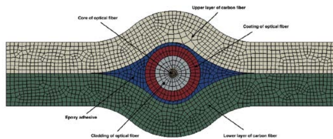
Figure 2-62 : Numerical meshed model of fiber optic sensor embedded in-between two composite plies.
