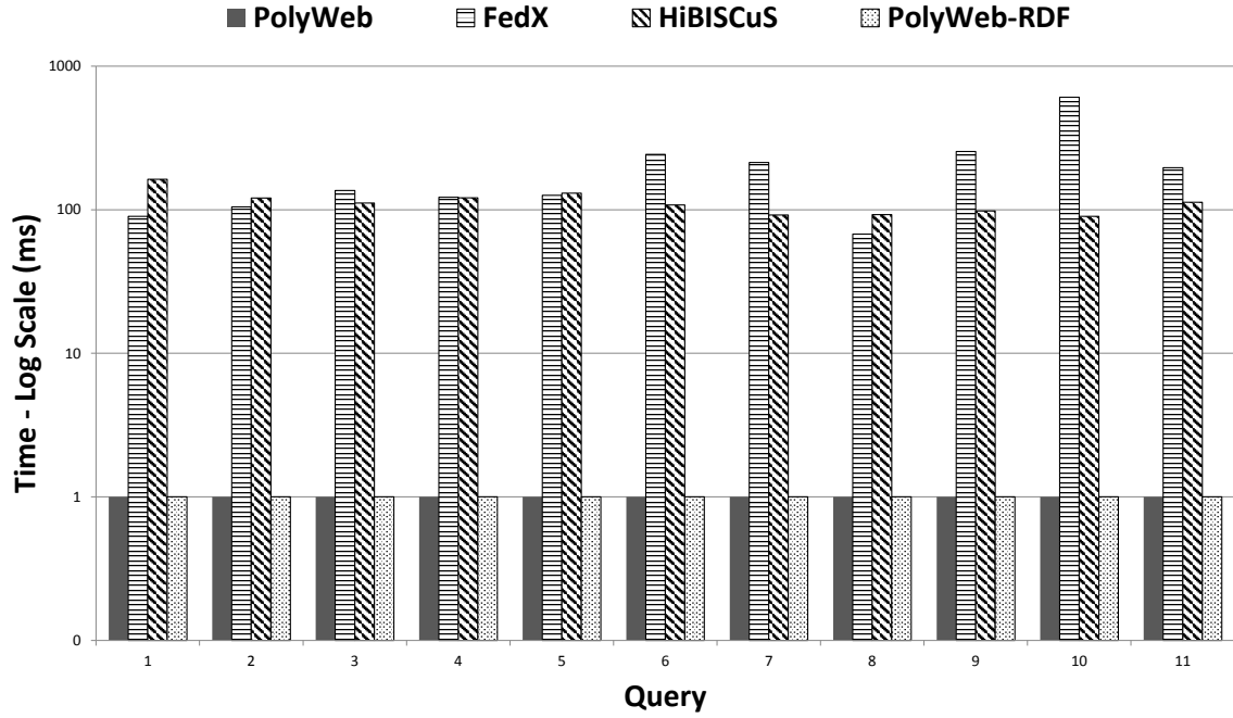
Figure 2.1: Comparison of source selection time
