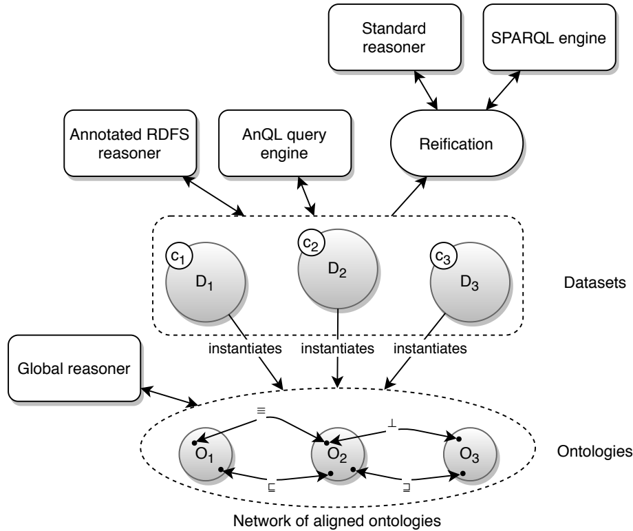
Figure 6.6: Overview of how the contributions relate to each others
