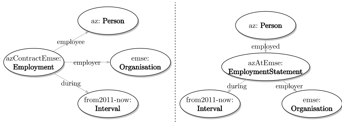
Figure 6.2: Example of nary relations: on the left, as a class; on the right, as a split property
