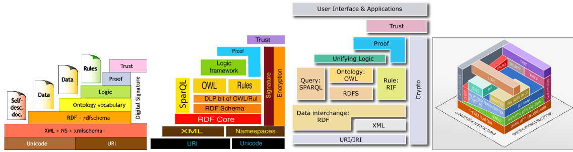
Figure 1: The Semantic Web layer cake and its evolution. From left to right: from [Berners-Lee et al., 2001] in 2001; 2004 version from W3C; 2007 version from Wikipedia; 2009 version posted on Flickr
