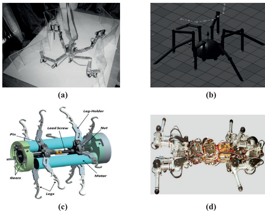
Figure 1.10 – Representation of the: (a) Robot of Rimon et al.[RSS01], (b) Robot of Gasparetto et al.[GVS08] , (c) Robot of Valdastrri et al.[Val+09] and (d) MORITZ robot [ZP03]
