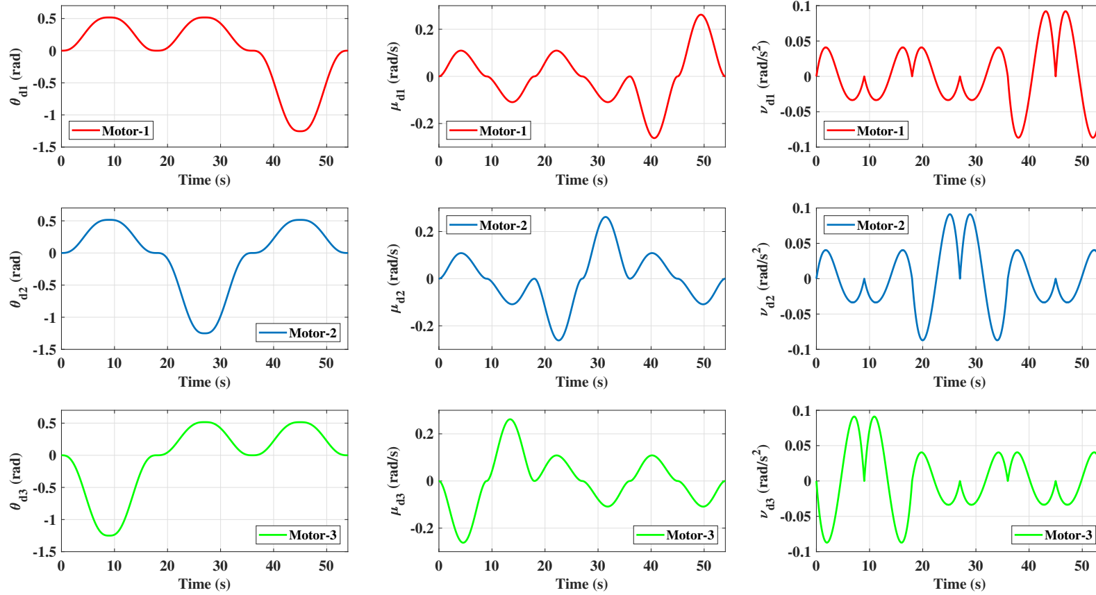
Figure 4.7 – Theoretical angular positions ( \theta_d ), velocities ( \mu_d ) and accelerations ( \nu_d ) of the pulleys of Motor-1 (red) , Motor-2 (blue) and Motor-3 (green) for one spring pull experiment
