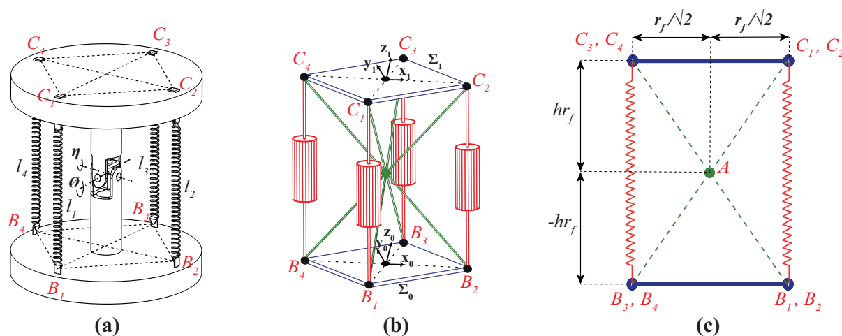
Figure 3.17 – Representation of the (a) Tensegrity mechanism at home-pose, (b) 3D view of the correlation to a 4-SPS-U manipulator and (c) 2D view of the manipulator
