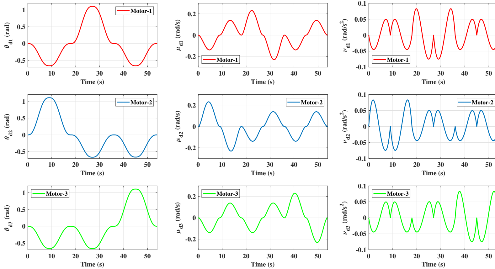
Figure 4.8 – Theoretical angular positions ( \theta_d ), velocities ( \mu_d ) and accelerations ( \nu_d ) of the pulleys of Motor-1 (red), Motor-2 (blue) and Motor-3 (green) for two springs pull experiment
