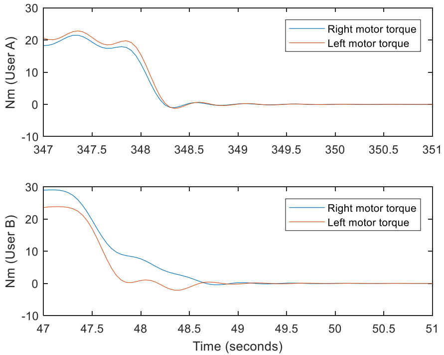
Figure 6.2.2. Motor torques during braking for user A and user B (experimental results)
