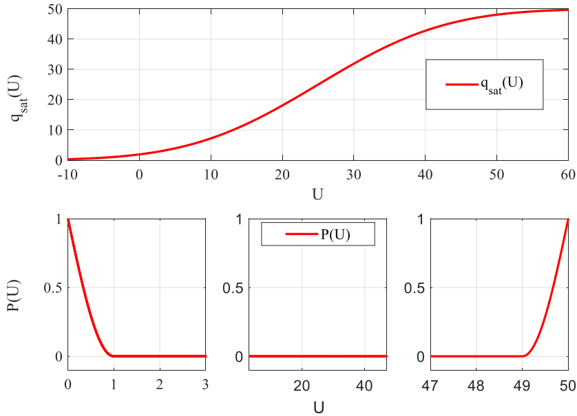
Figure 5.5.1. Smooth saturation function q_{\text{sat}} (above) and penalty function P_s for U_{\text{max}} = 50N (below)
