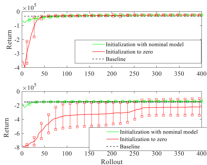
Figure 5.6.3. The mean performance of PoWER for both initialization (Top: \eta = 2 and bottom \eta = 1/2 )
