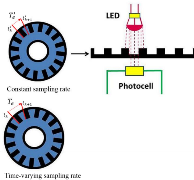
Figure 3.3.2. Working principles of the incremental encoder, constant sampling and time-varying sampling (Pogorzelski and Hillenbrand n.d.)
