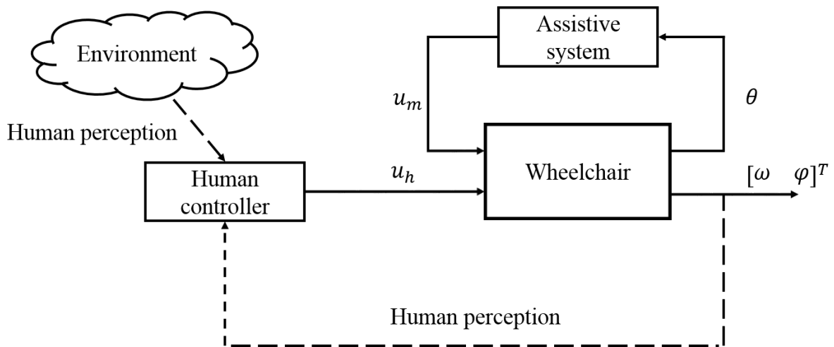
Figure 3.1.1. Power-assistance framework
