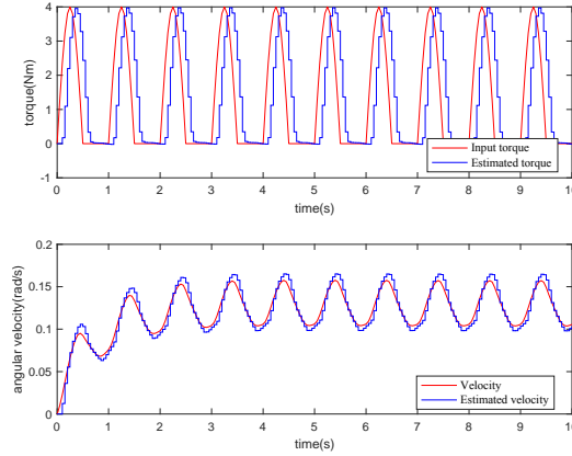
Figure 3.2.1. Driving simulation on a flat road without assistance (torque/velocity)
