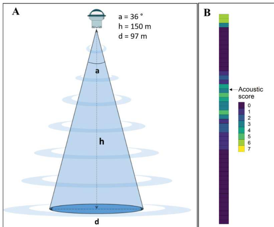
Figure 2.1: Technical specifications of the Marine Instruments M3I echosounder buoy. (A): beam width or cover angle (a), depth range (h), and diameter (D) at 150 m, (B): example of an acoustic sample.
