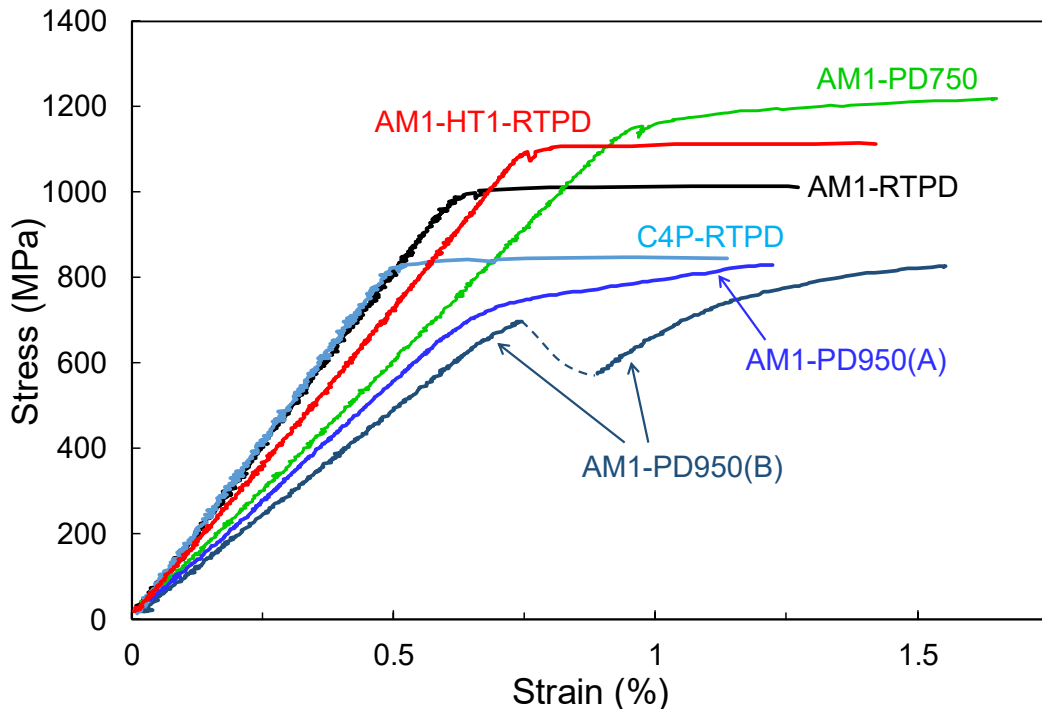
Figure 3.1. Tensile curves of pre-deformation applied to as-solutioned AM1 at RT (AM1-RTPD), at 750\text{ }^\circ\text{C} (AM1-PD750), at 950\text{ }^\circ\text{C} (AM1-PD950), and at RT after aging treatments Type-1 (AM1-HT1-RTPD), and applied to as-solutioned CMSX-4 Plus at RT (C4P-RTPD). Stress relaxation and creep during pause of tensile deformation are expressed as dashed line for AM1 pre-deformed at 950\text{ }^\circ\text{C} (AM1-PD950(B)).
