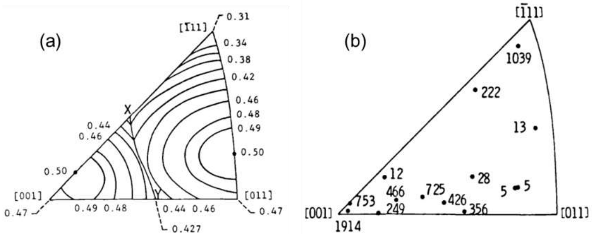
Figure 1.18. (a) Schmid factor contours for \langle 112 \rangle \{111\} slip systems. (b) Creep lives of MarM200 SX specimen tested at 750 °C / 689 MPa, creep duration in h associated with orientation. [83]
