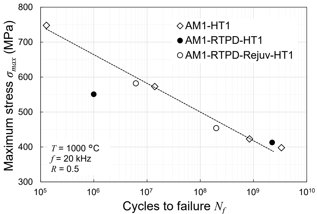
Figure 5.2. Results of VHCF tests at 1000\text{ }^\circ\text{C} / f = 20\text{ kHz} / R = 0.5 in S-N diagram. The maximum stress is plotted as a function of the number of cycles to failure
