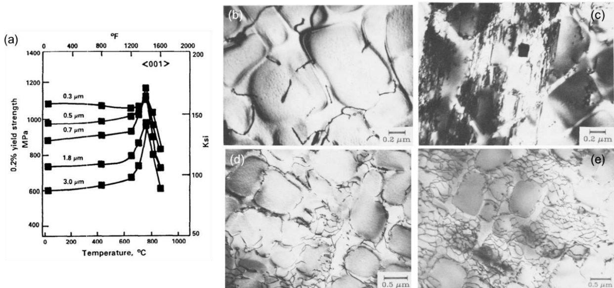
Figure 1.12. Effect of temperature and precipitation size on 0.2% offset yield strength of oriented \langle 001 \rangle PWA1480 (a) [49]. Dislocations observed after tensile tests on PWA1480 at 20 ^{\circ}C (b), 705 ^{\circ}C (c), 982 ^{\circ}C (d), and 1093 ^{\circ}C (e), g = \langle 200 \rangle [63].
