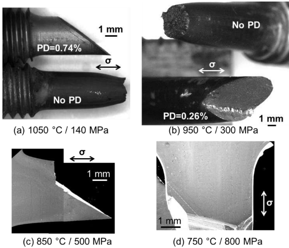
Figure 1.41. Observed images of specimens' fracture surfaces after the creep rupture tests.
