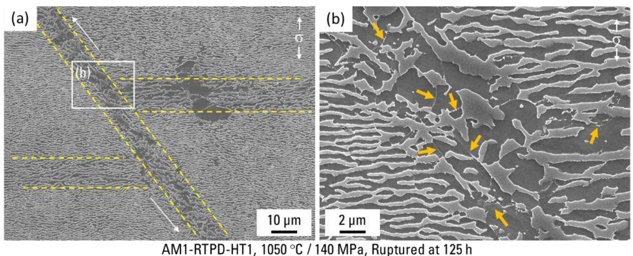
Figure 4.9. Precipitation scale microstructures of AM1-RTPD-HT1 after creep rupture test at 1050 °C / 140 MPa. In (a), dotted lines are showing microstructure coarsened bands and arrows are indicating direction of sliding. (b) is a magnified image of the area surrounded by the rectangle in (a). Arrows in (b) are pointing at recrystallized grain boundaries.
