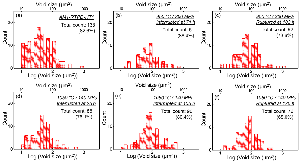
Figure 4.33. Histograms of counts of voids in the microstructure coarsened bands vs. void size in a logarithmic scale of \mu\text{m}^2 obtained by image analyses along longitudinal sections of AM1 specimen. The total void count and percentage of voids in the band are labeled in the figures.
